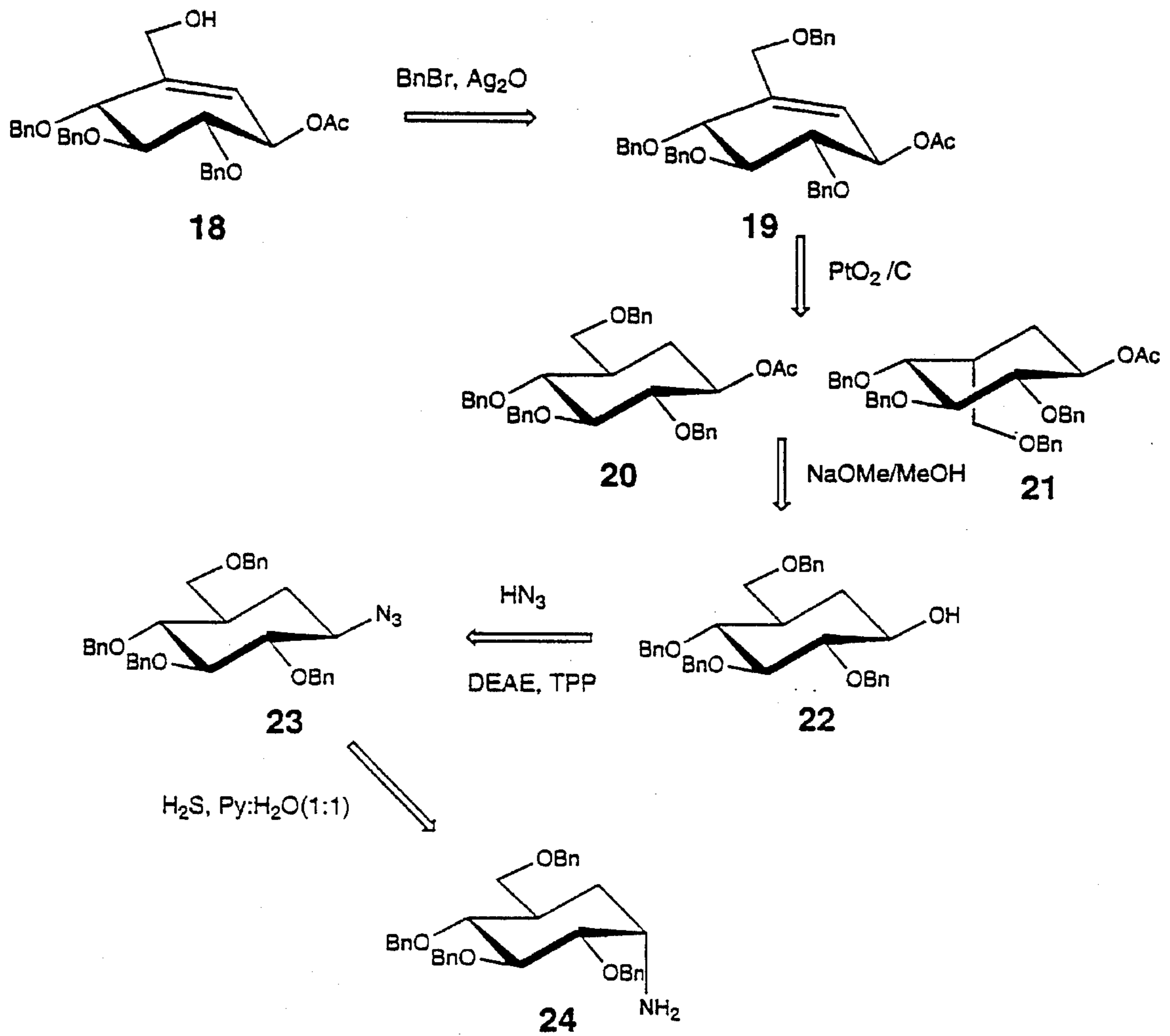
1D-(1,2,4,13,5)-1-amino-2,3,4-tri-O-benzyl-5-c-benzyloxymethyl-1,2,3,4-cyclohexane tetrol
