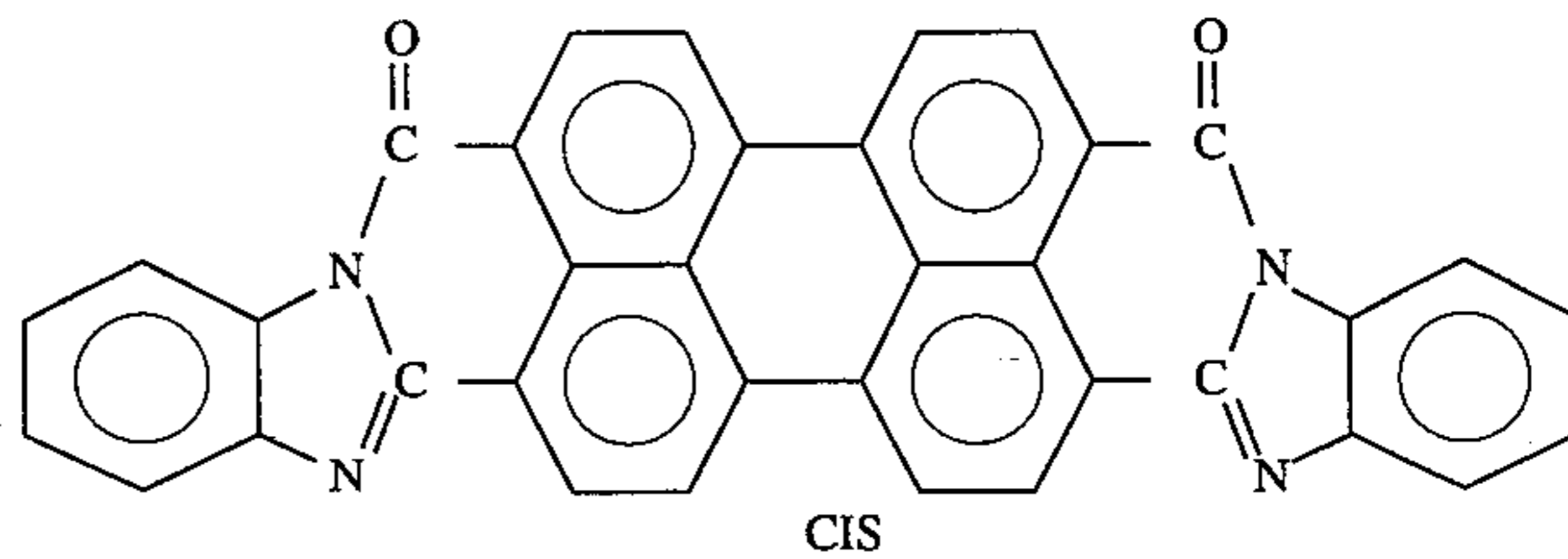
bisbenzimidazo(2,1-a-1',1'-b)anthra(2,1,9-def:6,5,10-d'e'f)diisoquinoline-6,11-dione
