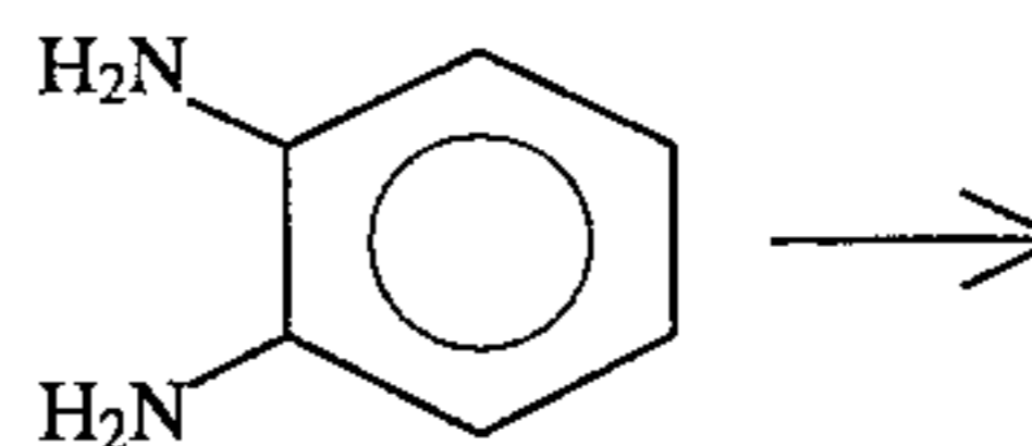
1, 2-phenylene
