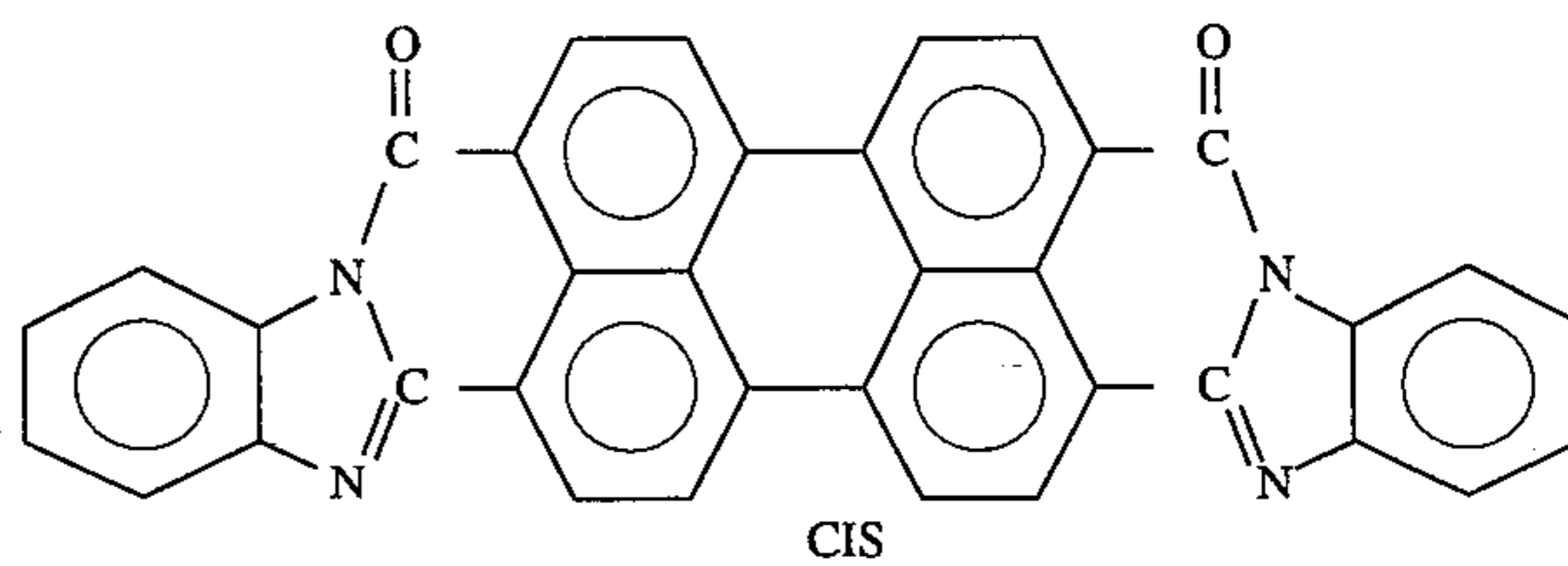
bisbenzimidazo(2,1-a-1',1'-b)anthra(2,1,9-def:6,5,10-d'e'f)diisoquinoline-6,11-dione
