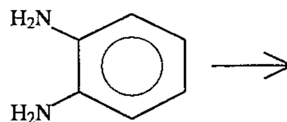
1, 2-phenylene
