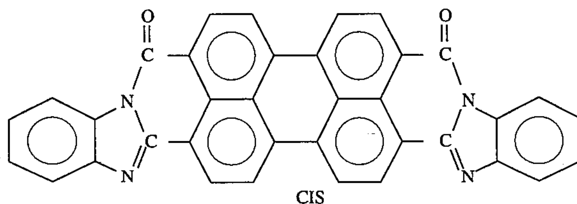
bisbenzimidazo(2,1-a-1',1'-b)anthra(2,1,9-def:6,5,10-d'e'f)disoquinoline-6,11-dione
