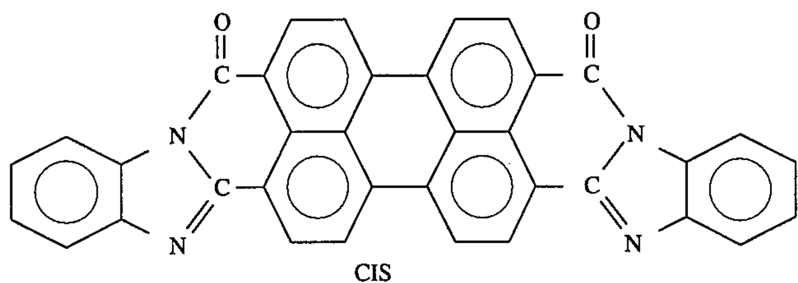
bisbenzimidazo(2,1-a-1',1'-b)anthra(2,1,9-def:6,5,10-d'e'f)diisoquinoline-6,11-dione
