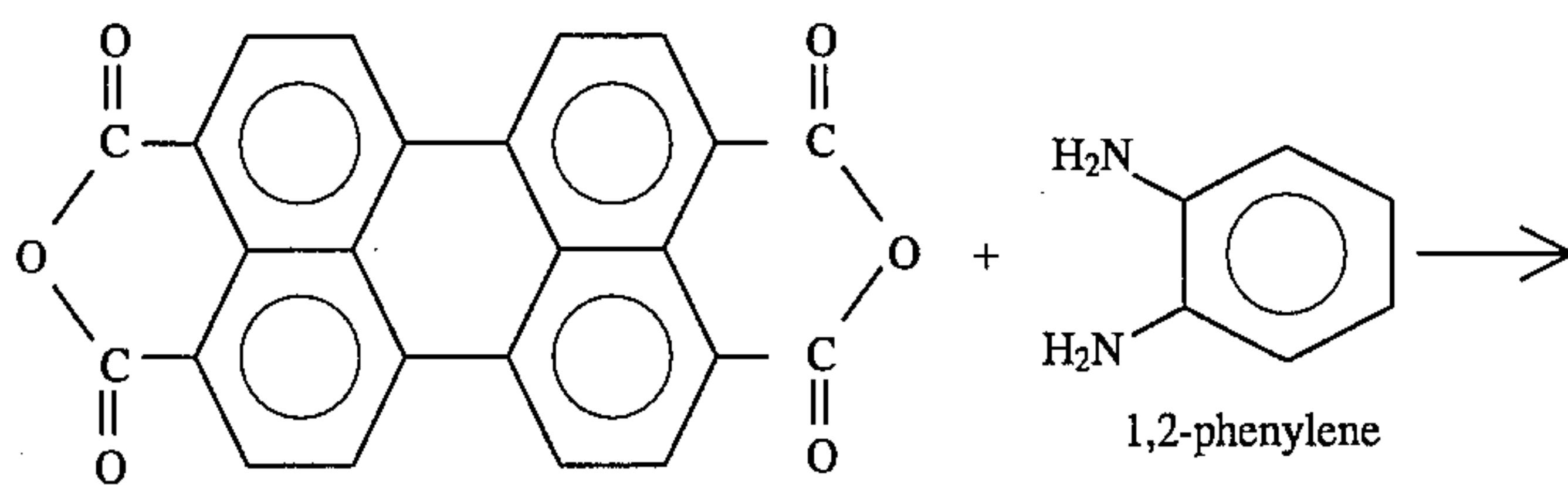
Perylene 3,4,9,10-tetracarboxylic acid dianhydride
