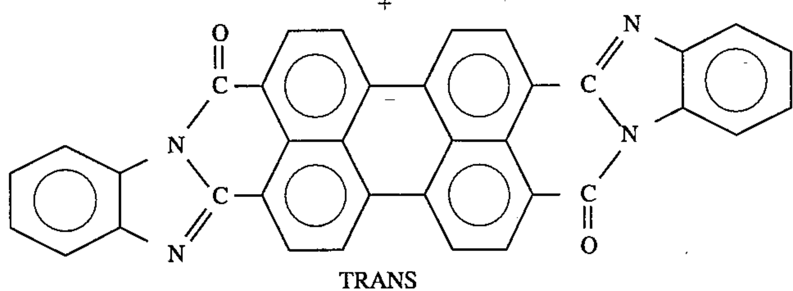
bisbenzimidazo(2,1-a-1',1'-b)anthra(2,1,9-def:6,5,10-d'e'f)diisoquinoline-10,21-dione
