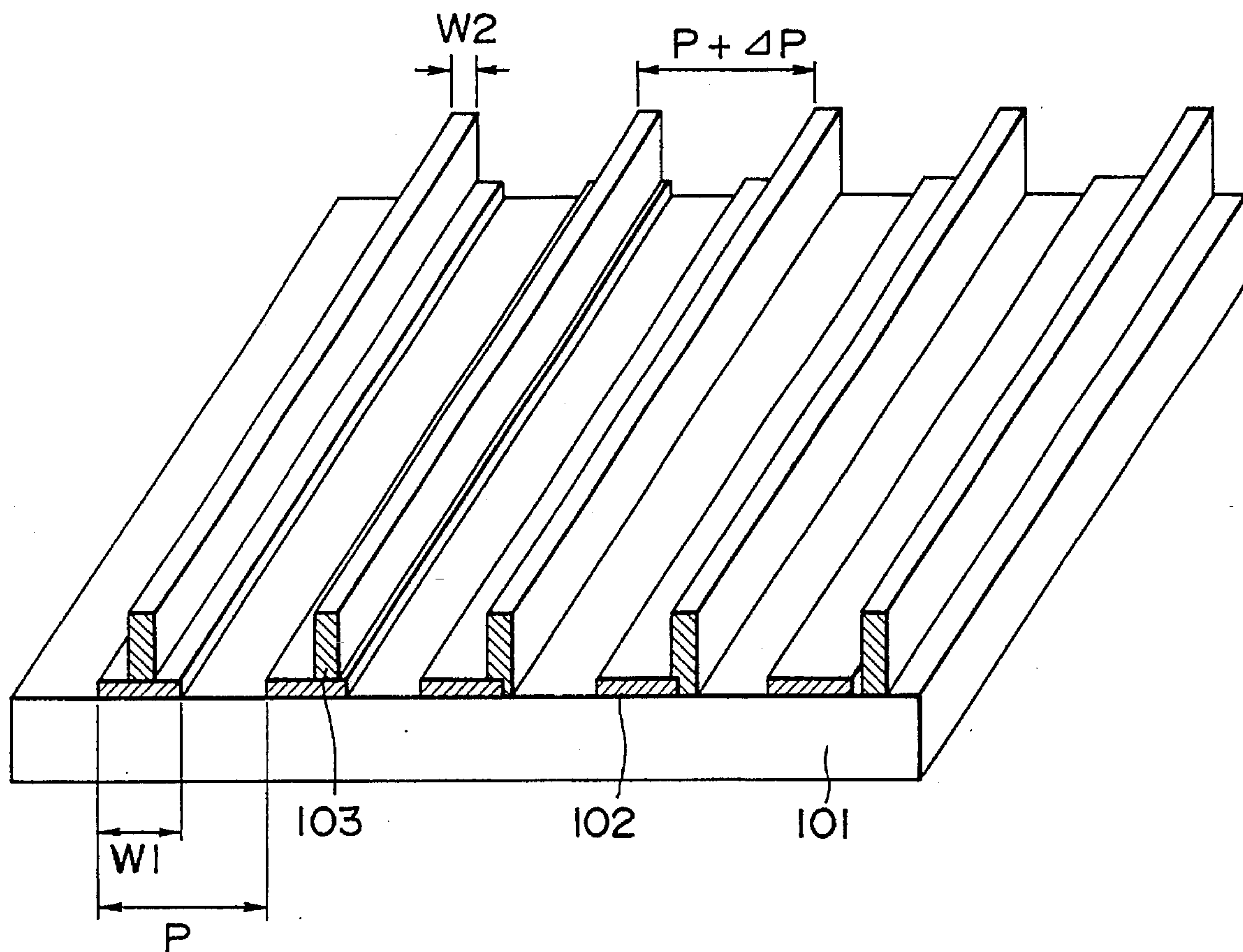
FIG. 7 (PRIOR ART)
