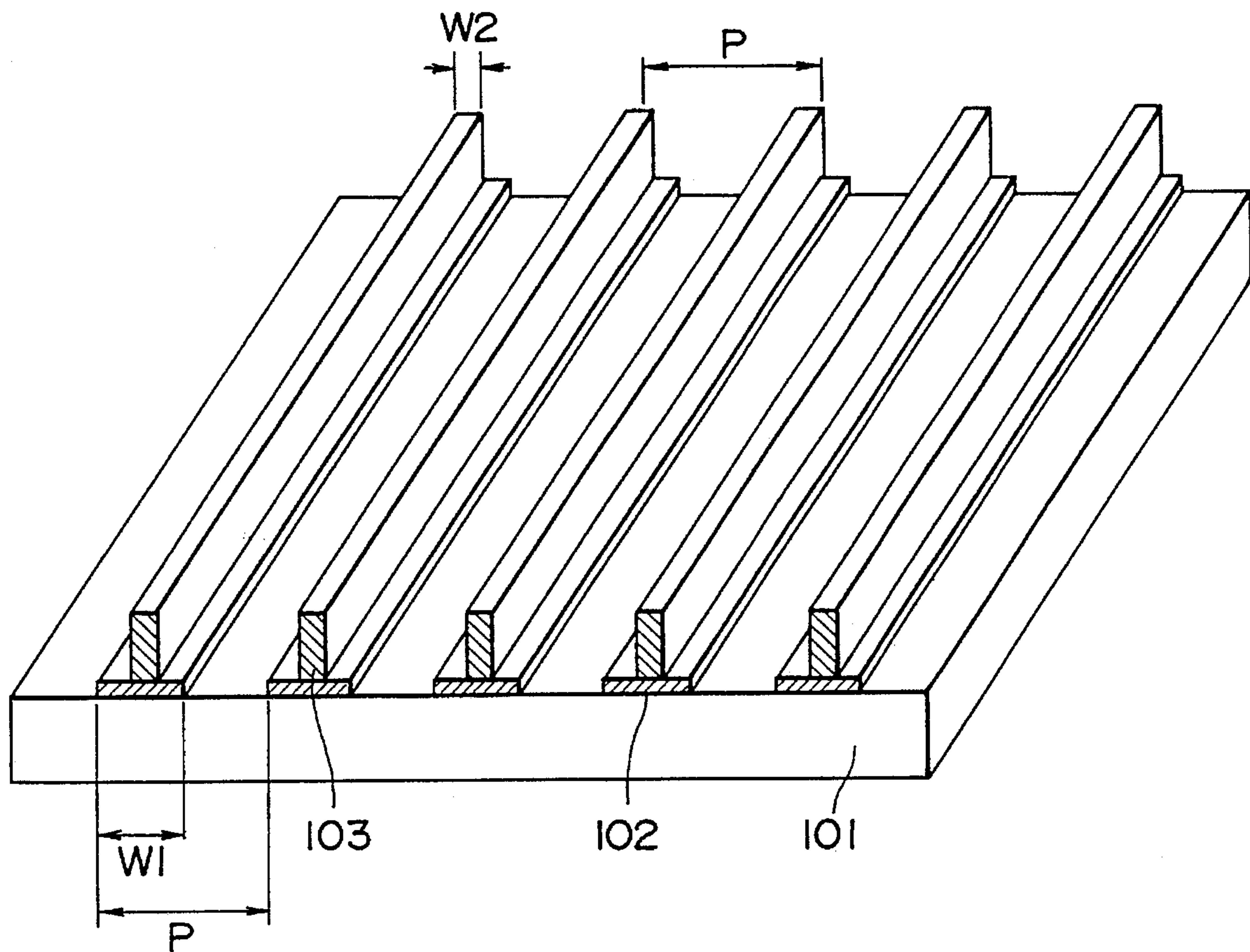
FIG. 6 (PRIOR ART)
