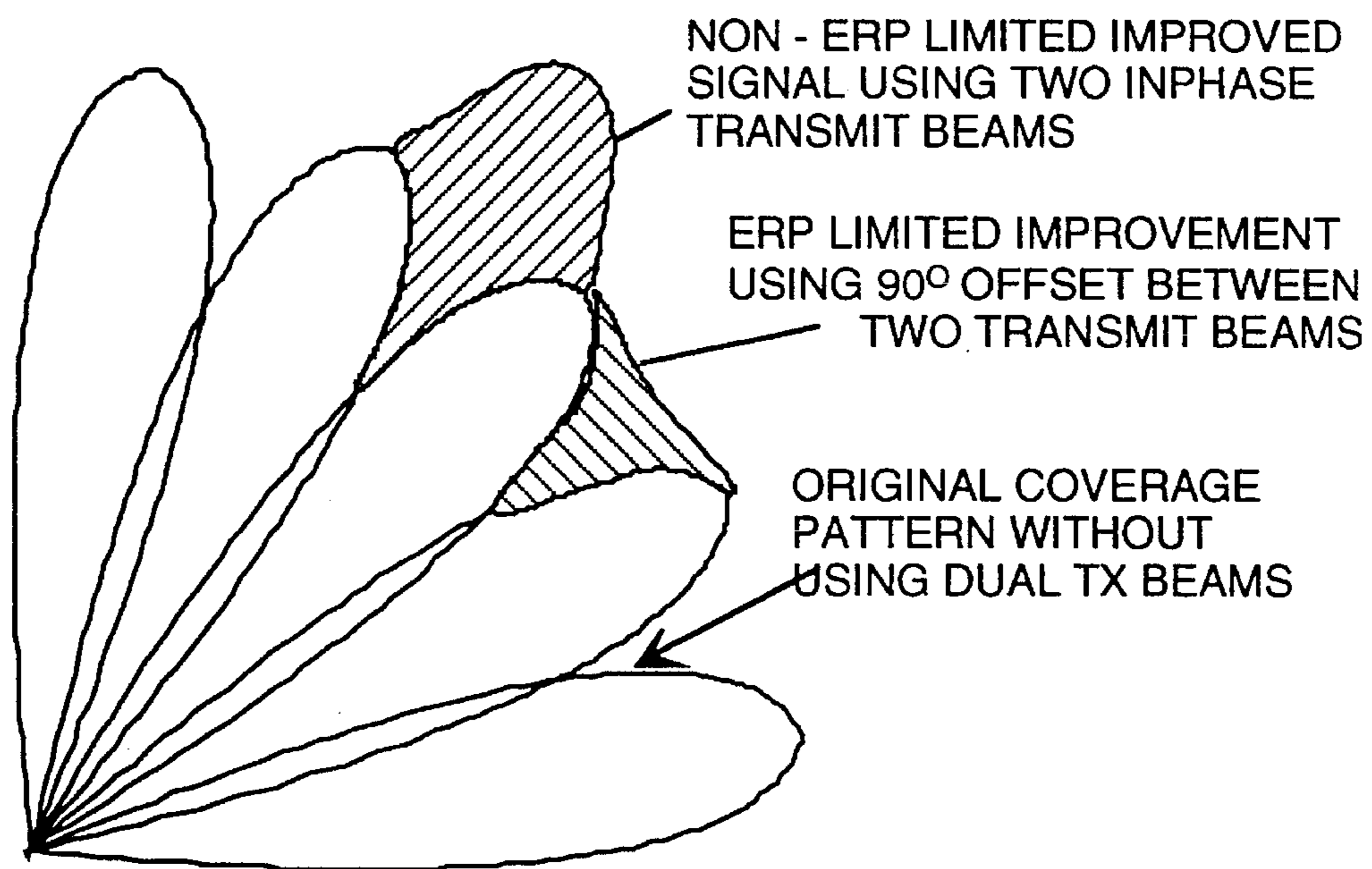
Fig. 14 (c)
