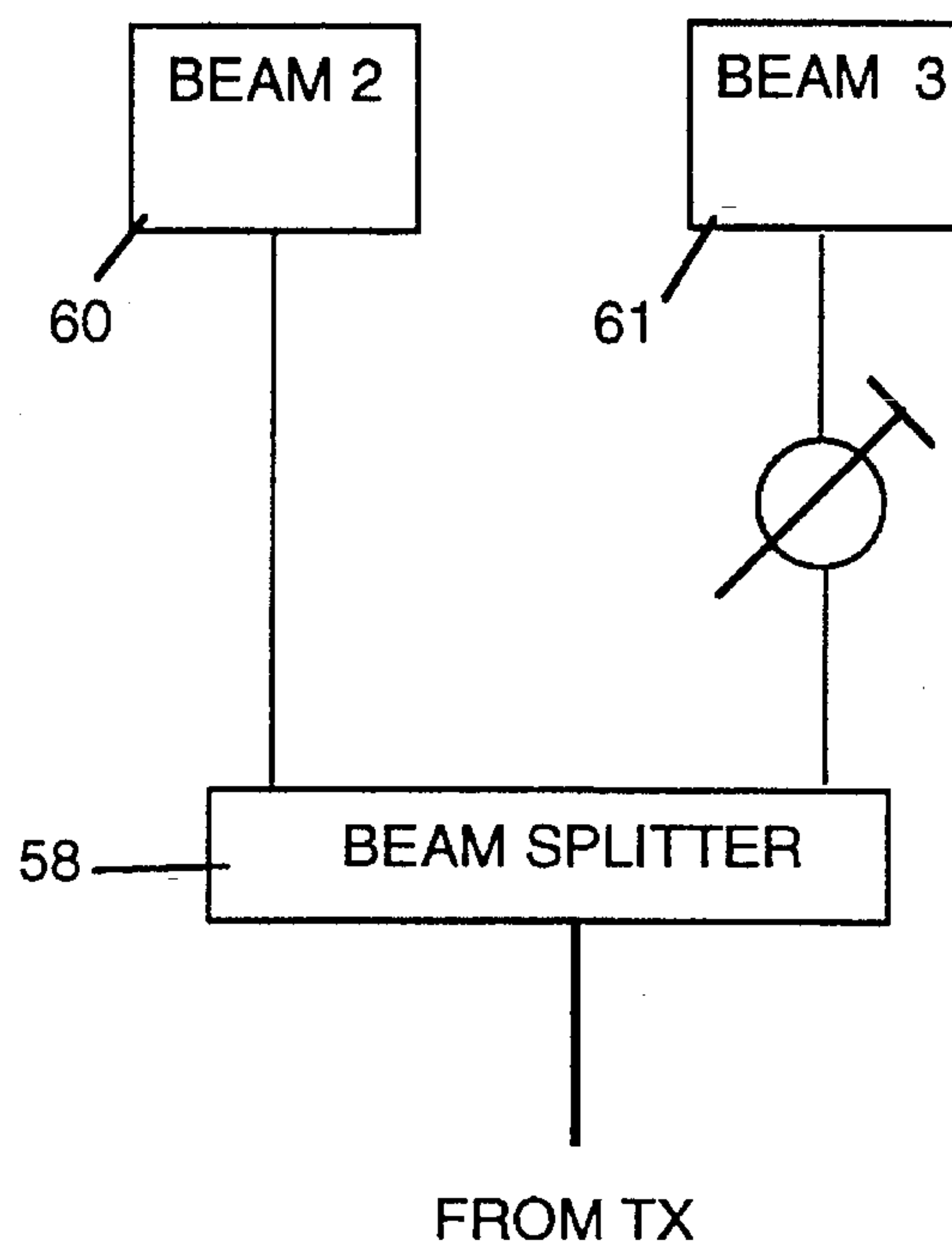
Fig. 14 (b) QUADRATURE
