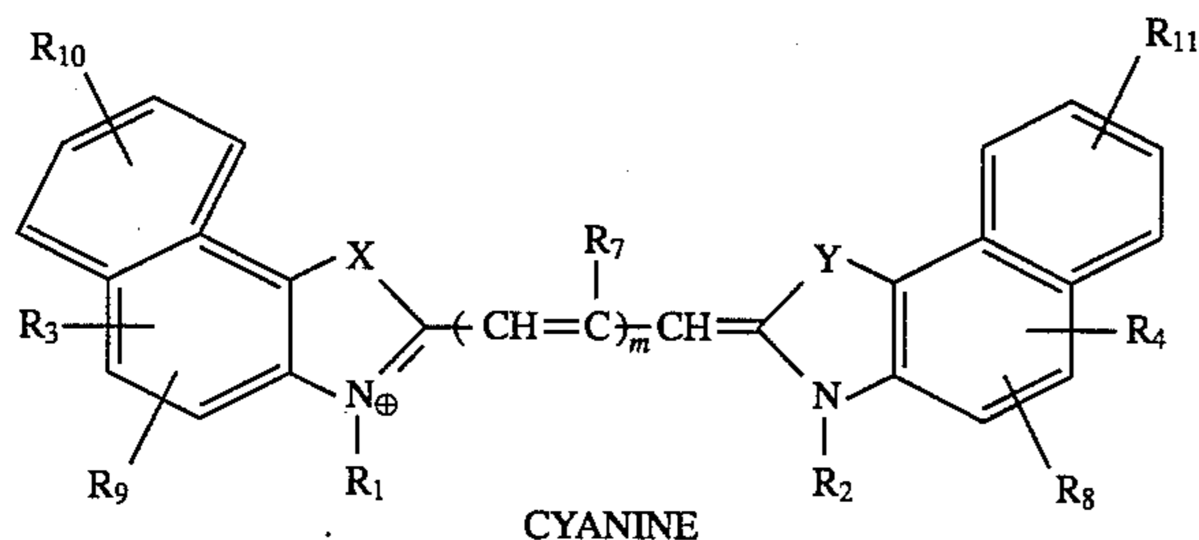
CYANINE
