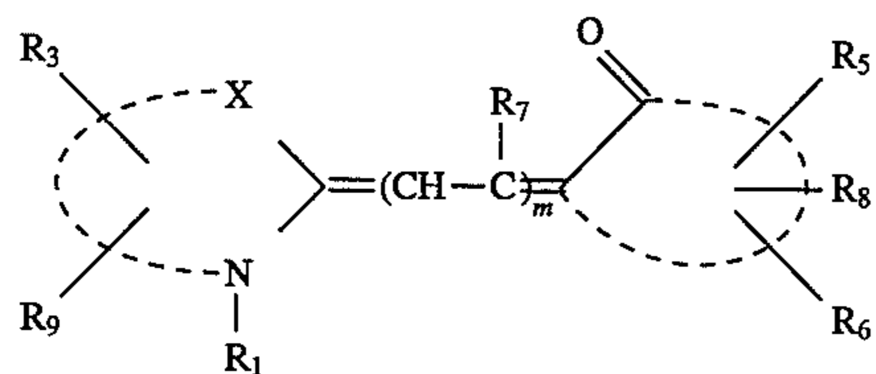
MEROCYANINE
