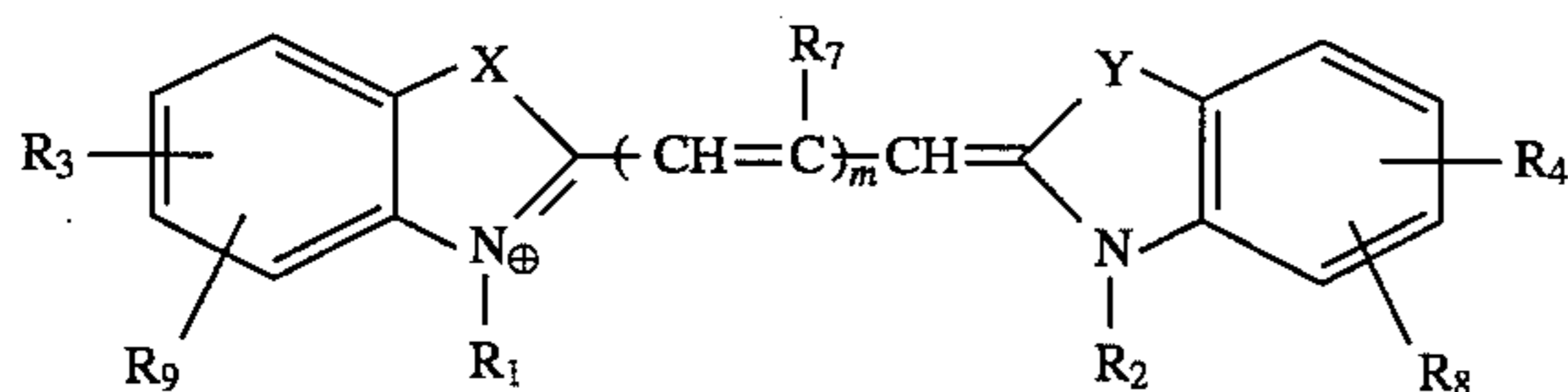
CYANINE
