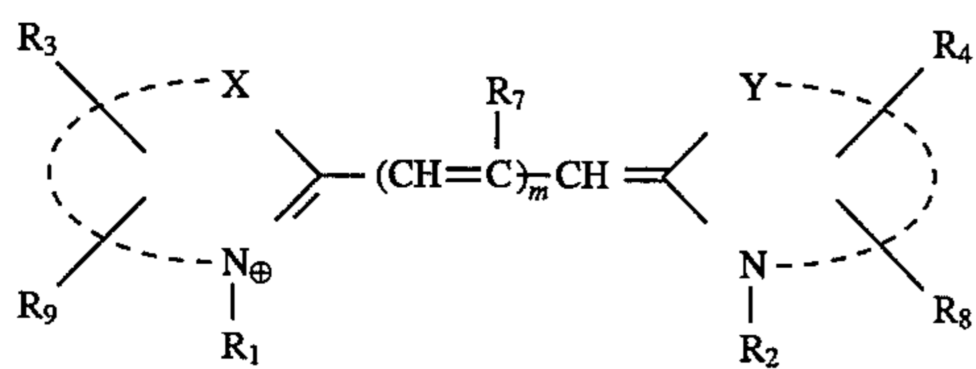
CYANINE
