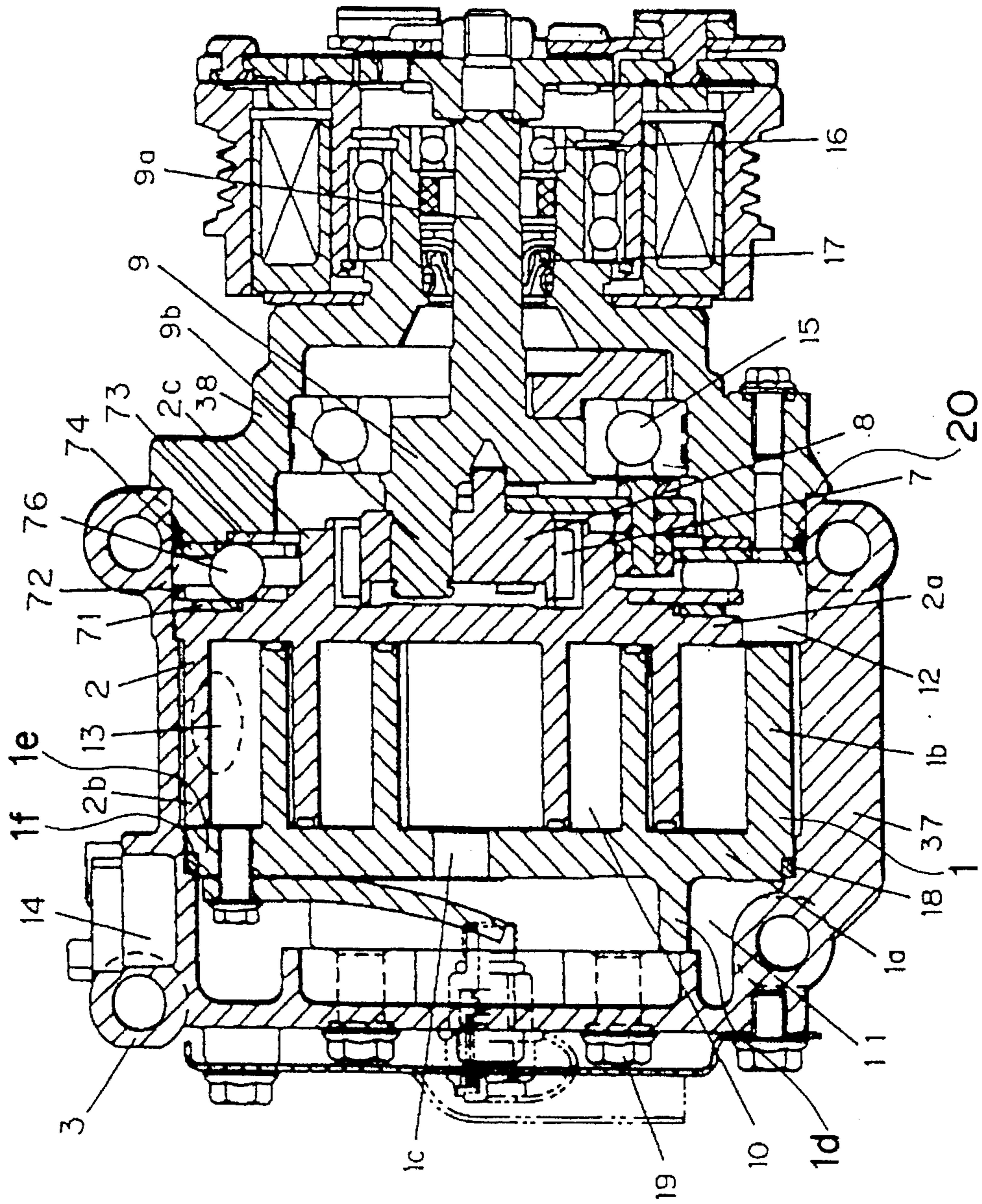
Fig. 8 PRIOR ART
