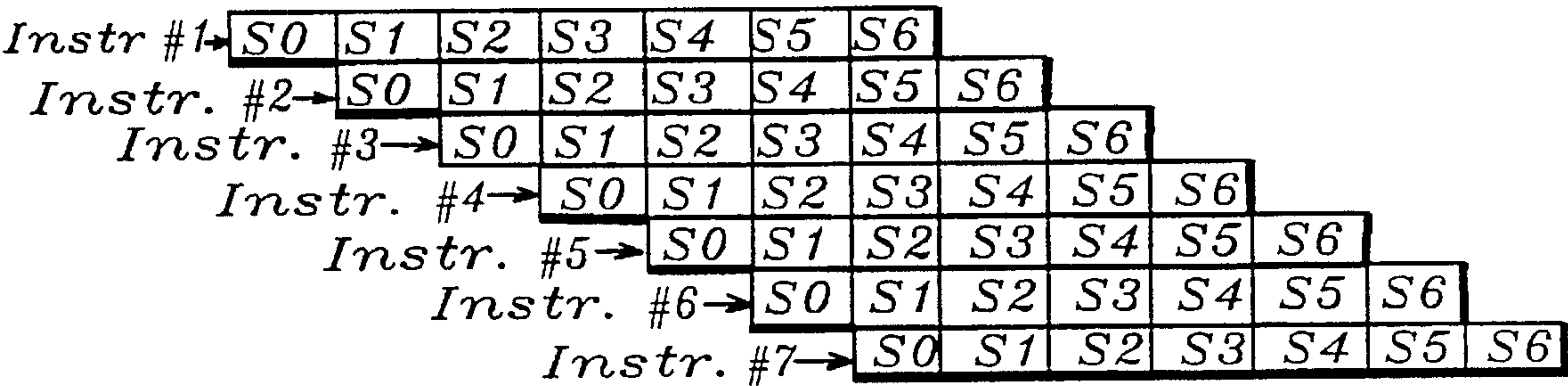
FIG 7 PIPELINE
