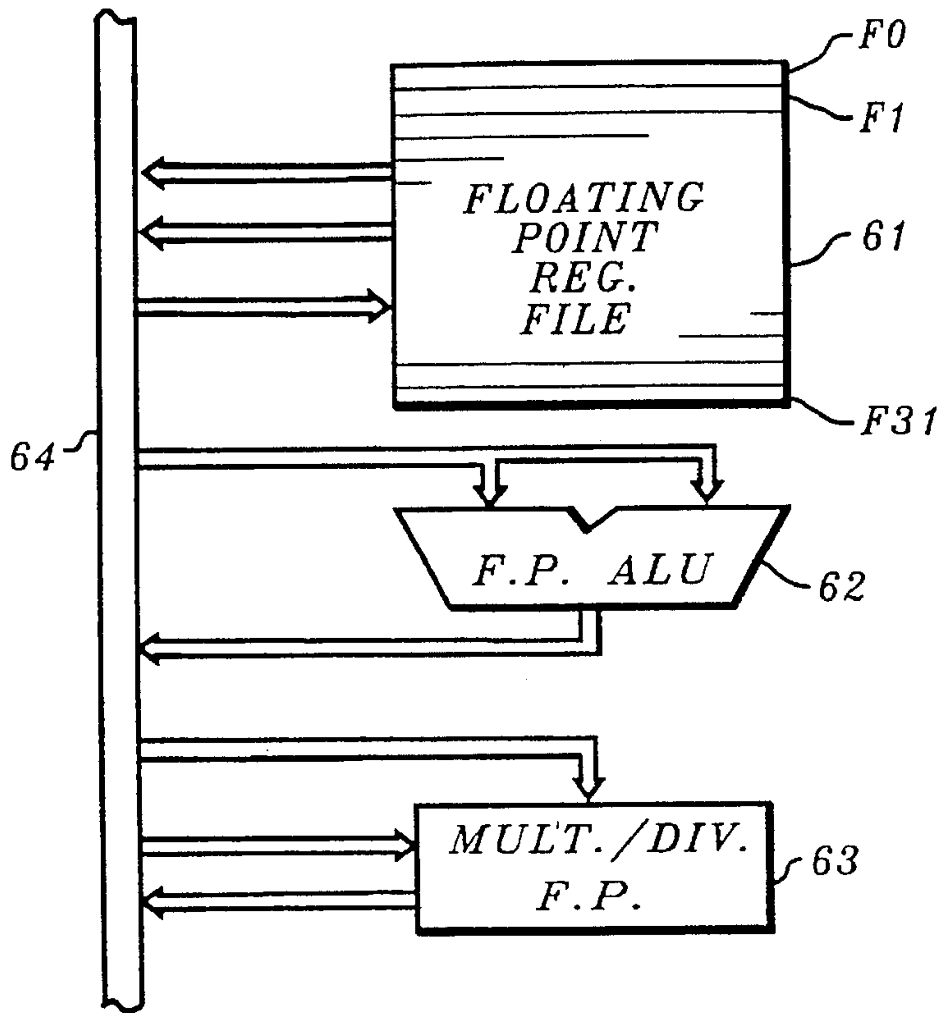
FIG 6 F-BOX
