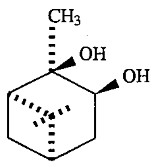
(1R, 2R, 3S, 5R)-(-)-pinanediol [\alpha]^{21} = -8.6^\circ (c = 6.5, toluene) for material which is >99% ee
