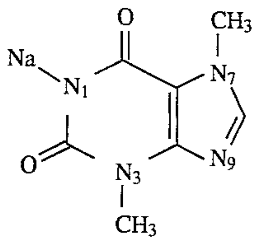
Sodium theobromine II.
