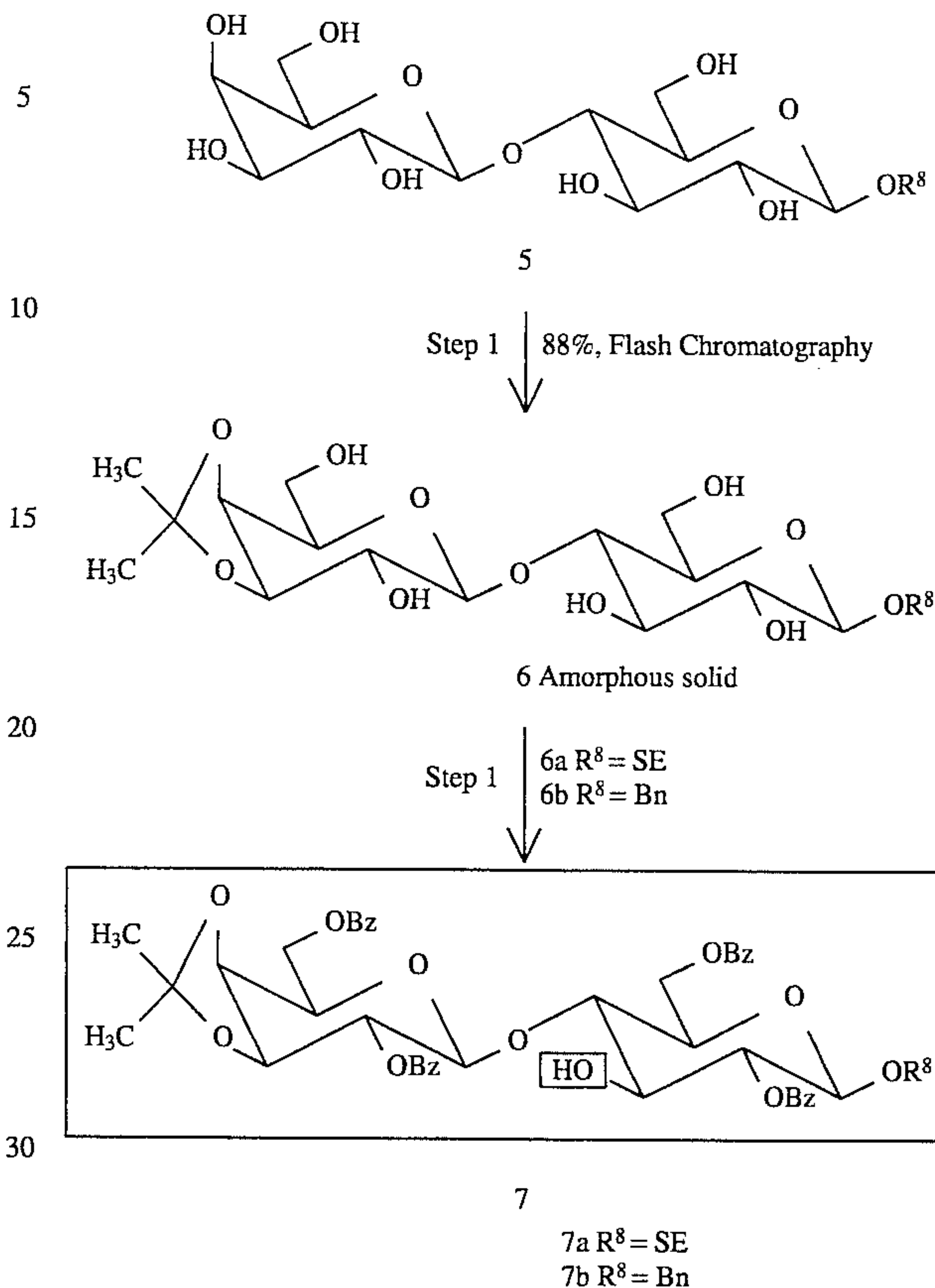
Reaction Scheme 1
