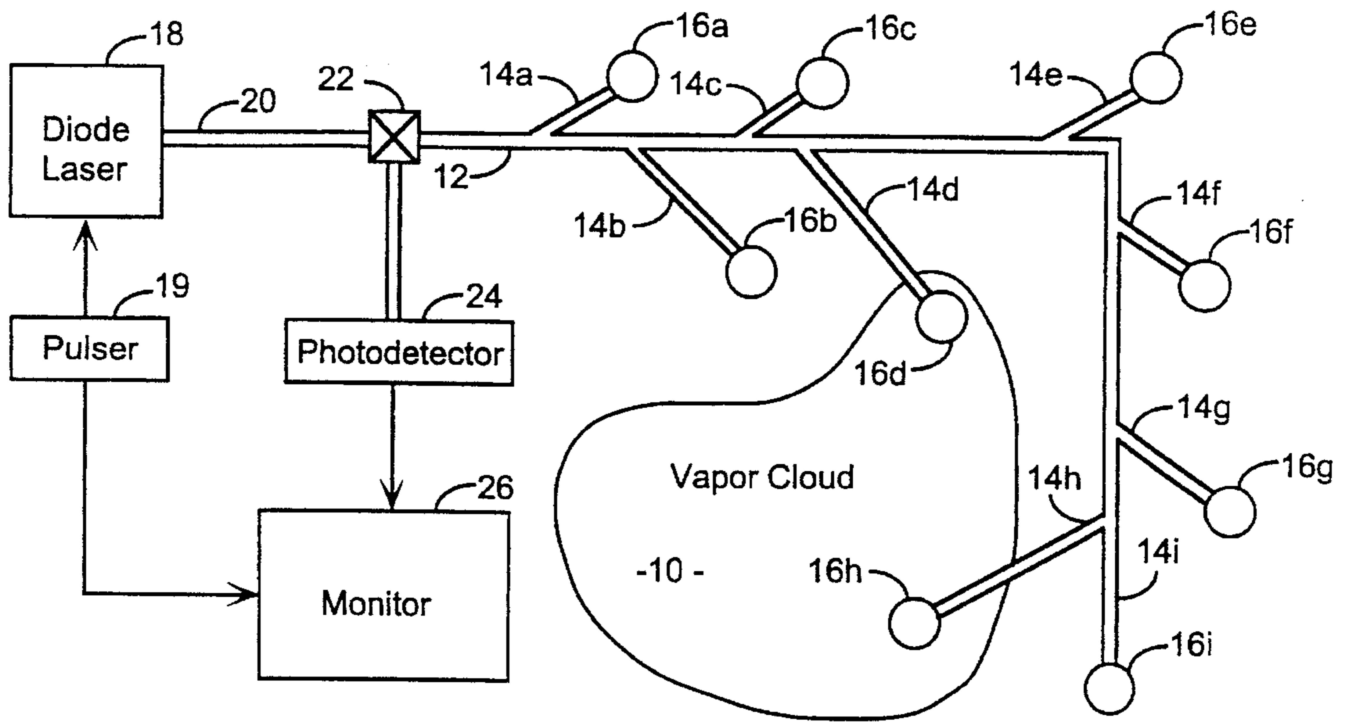
Intensity-Based Fiber Optic Dosimeter Network
