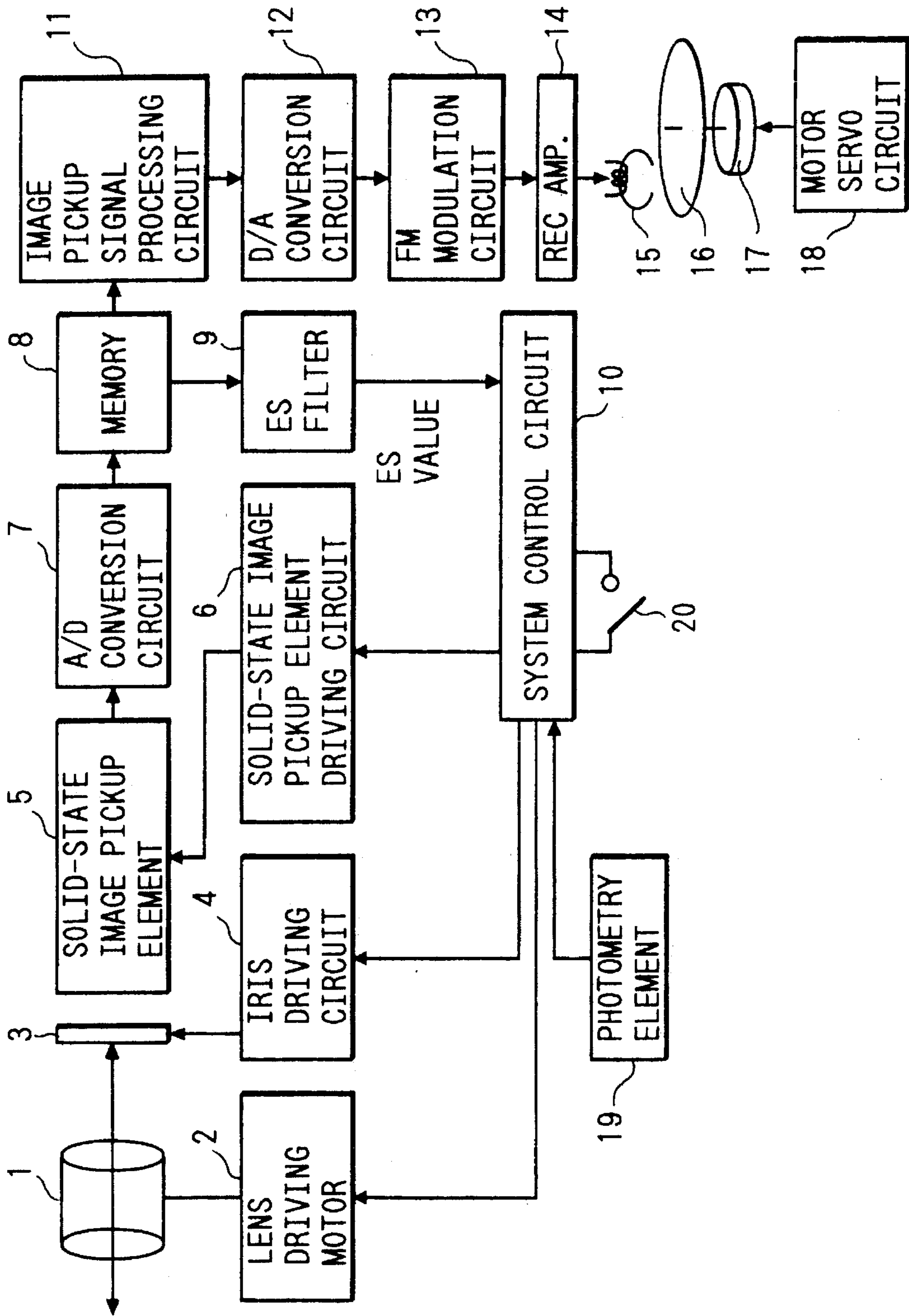
FIG. 1 (PRIOR ART)
