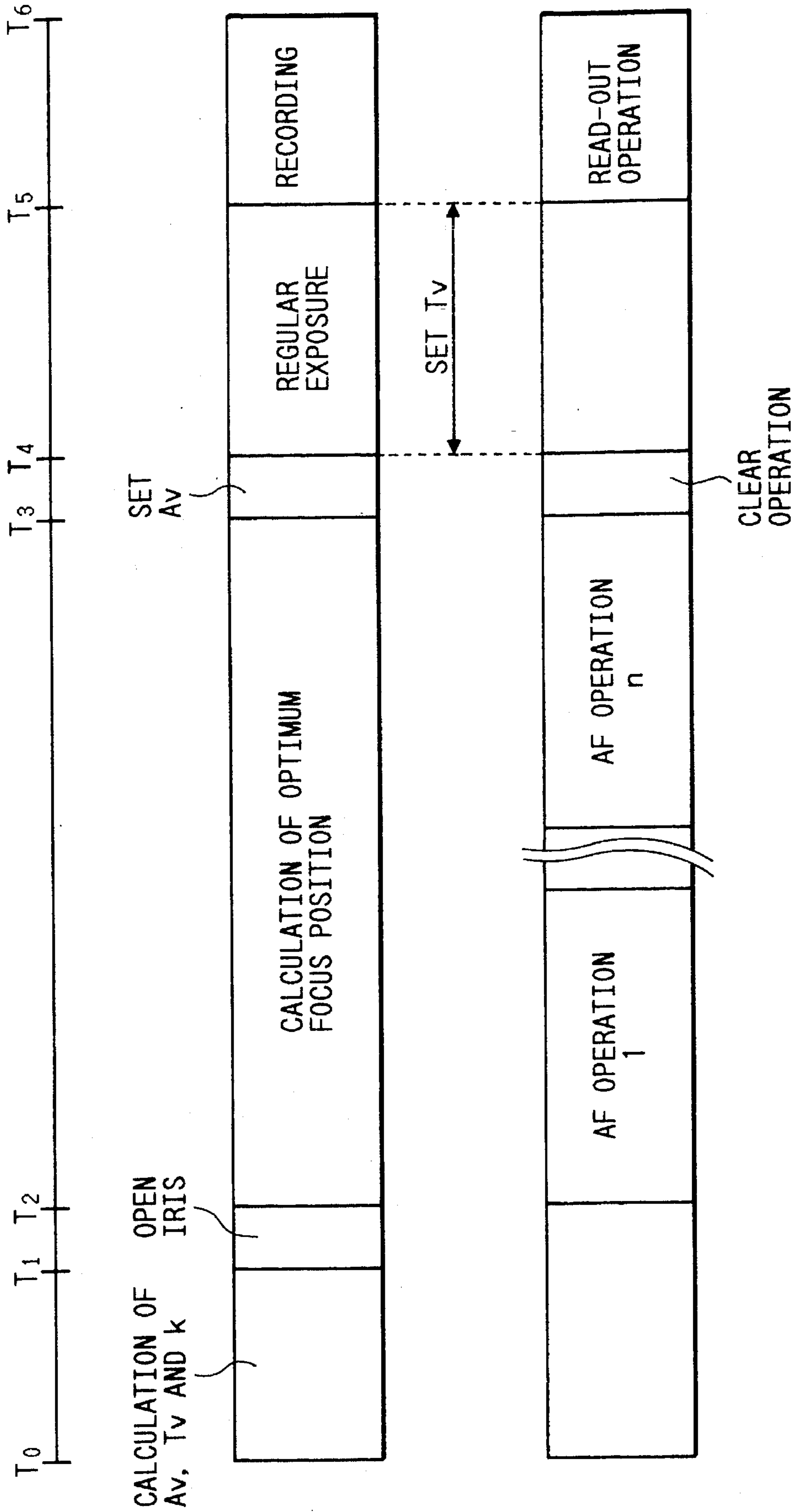
FIG. 3 (PRIOR ART)
