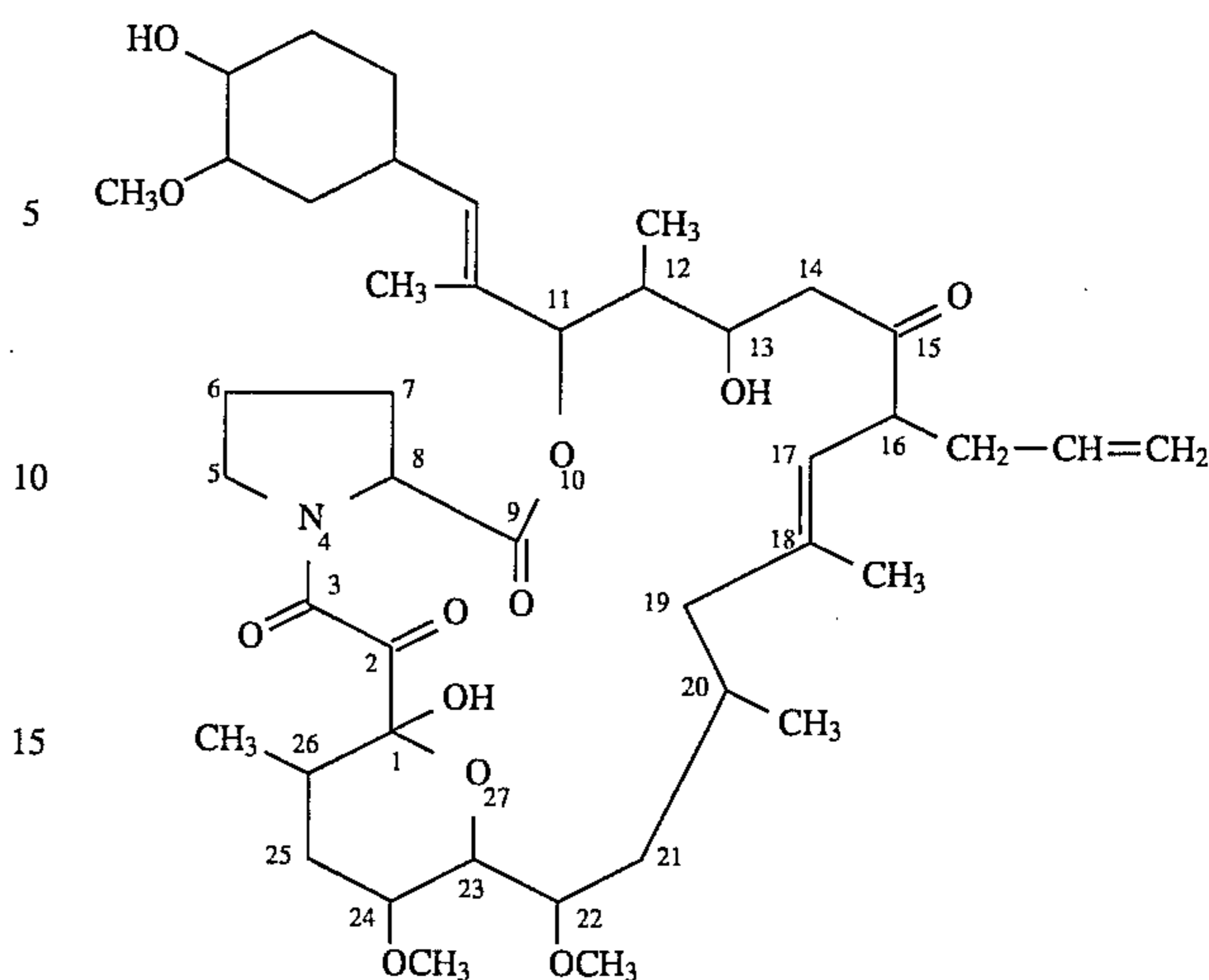
16-Allyl-1,13-dihydroxy-11-[2-(4-hydroxy-3-methoxycyclohexyl)-1-methylvinyl]-22,24-dimethoxy-12,18,20,26-tetramethyl-10,27-dioxo-4-azatricyclo[21.3.1.0 4,8 ]heptacos-17-ene-2,3,9,15-tetraone
