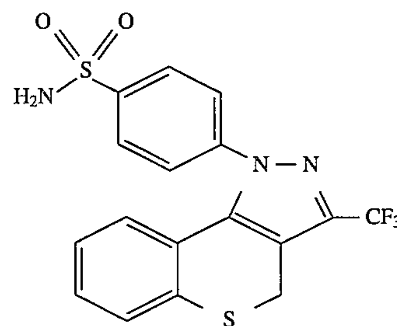
4-[1,4-Dihydro-3-(trifluoromethyl)-[1]benzothiopyrano[4,3-c]pyrazol-1-yl]benzenesulfonamide
