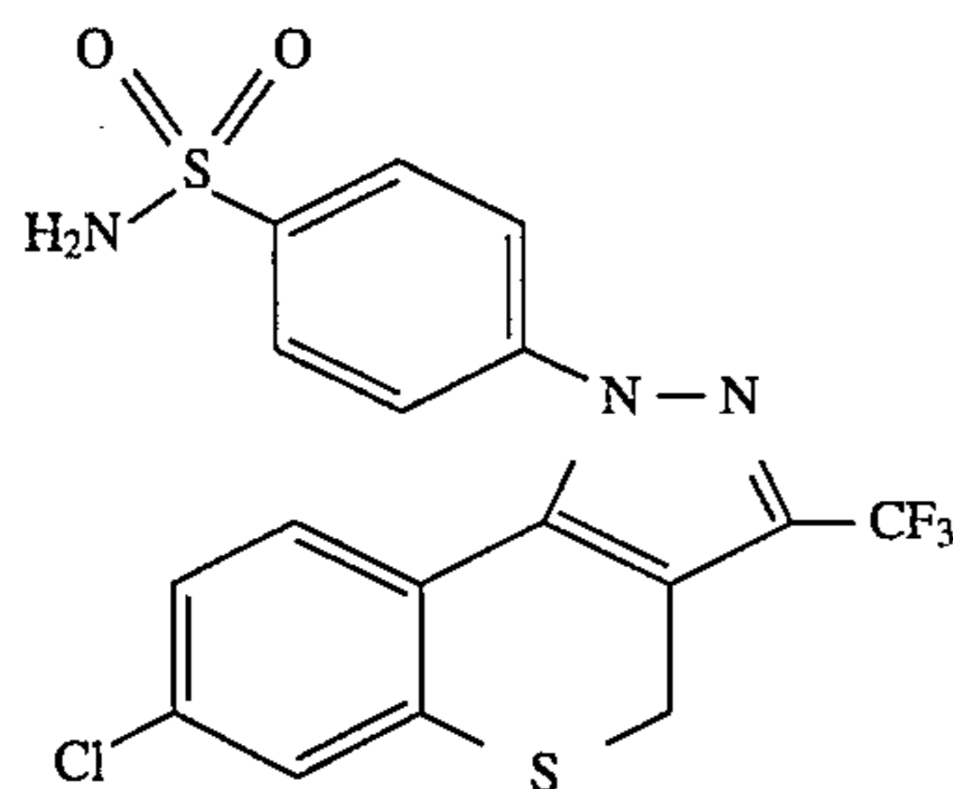
4-[7-Chloro-1,4-dihydro-3-(trifluoromethyl)-[1]benzothiopyrano[4,3-c]pyrazol-1-yl]benzenesulfonamide
