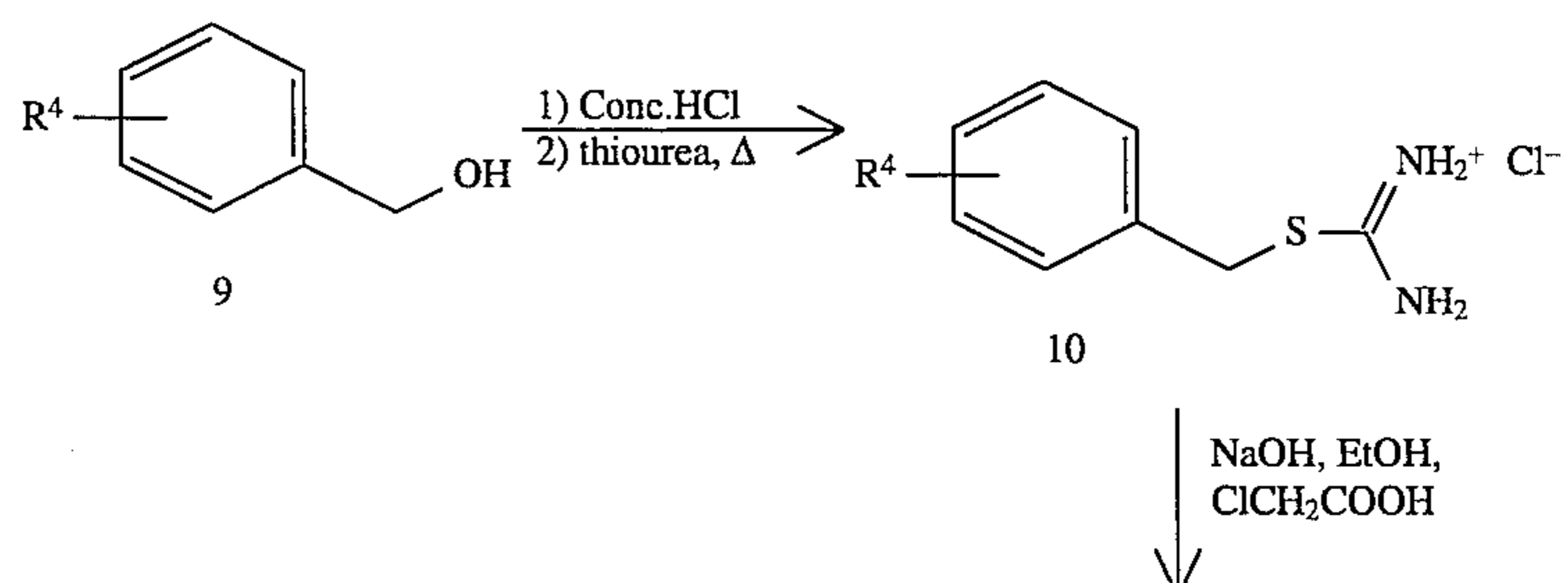
SCHEME III
