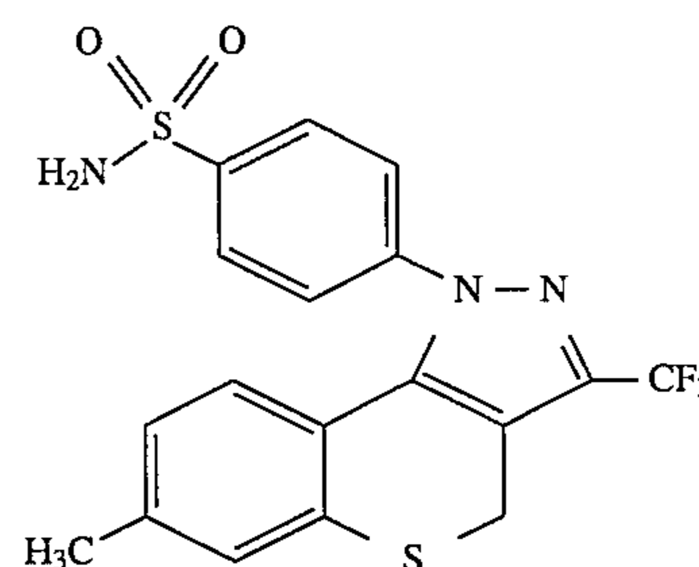
4-[1,4-Dihydro-7-methyl-3-(trifluoromethyl)-[1]benzothiopyrano[4,3-c]pyrazol-1-yl]benzenesulfonamide
