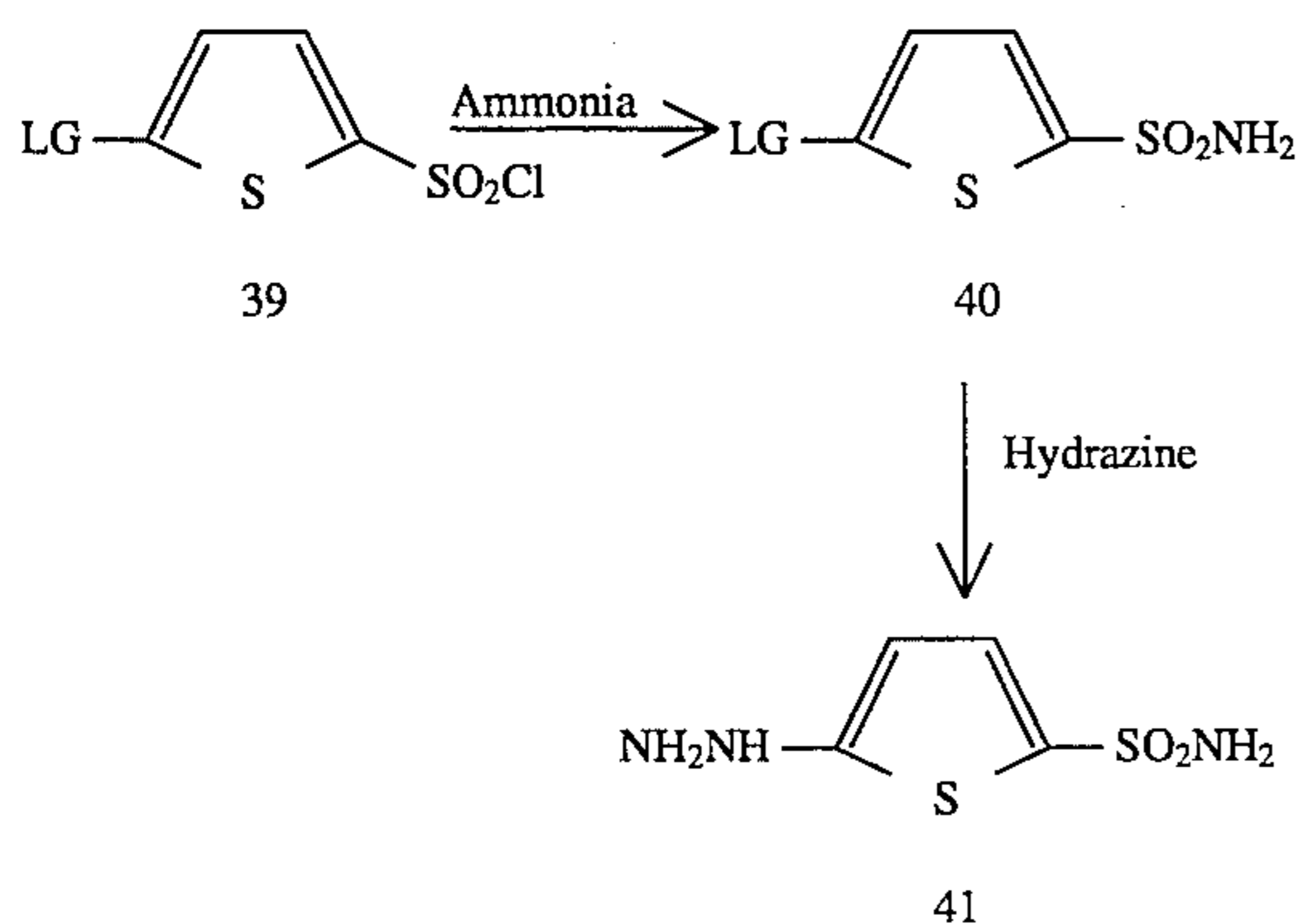
SCHEME XII
