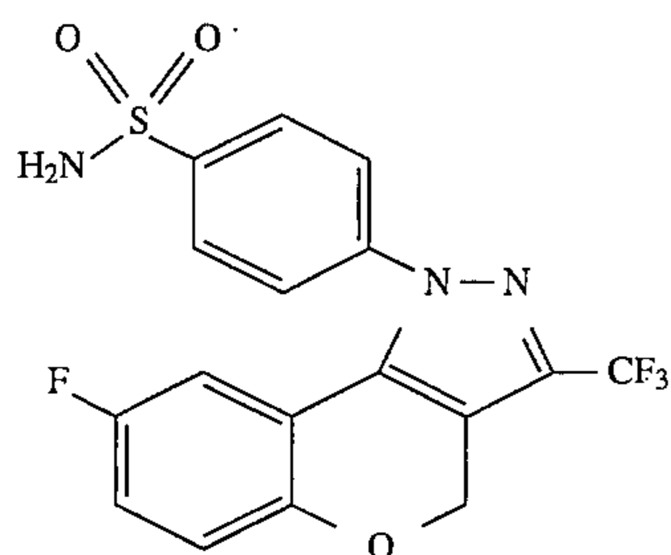
4-[1,4-Dihydro-8-fluoro-3-(trifluoromethyl)-[1]benzopyrano[4,3-c]pyrazol-1-yl]benzenesulfonamide
