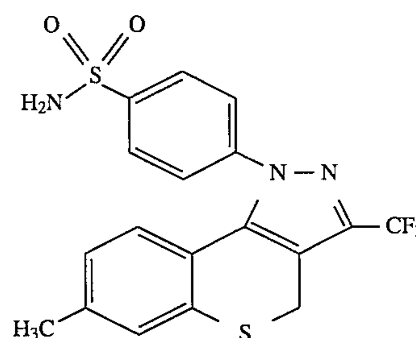
4-[1,4-Dihydro-7-methyl-3-(trifluoromethyl)-[1]benzothiopyrano[4,3-c]pyrazol-1-yl]benzenesulfonamide
