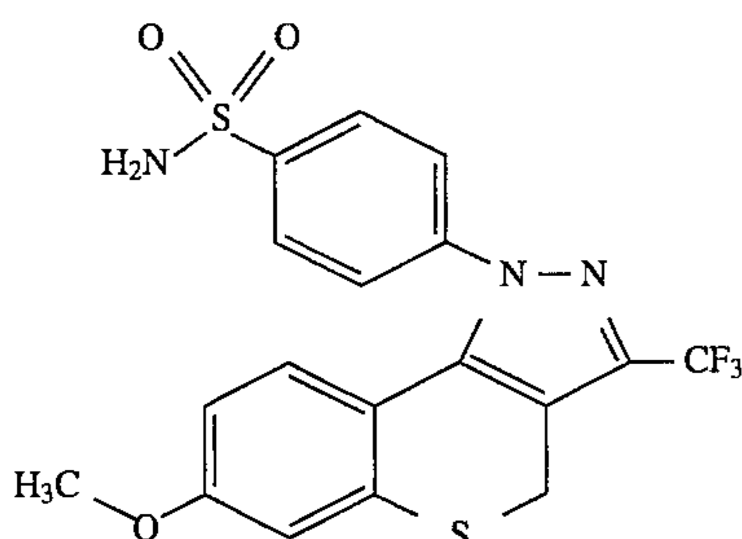
4-[1,4-Dihydro-7-methoxy-3-(trifluoromethyl)-[1]benzothiopyrano[4,3-c]pyrazol-1-yl]benzenesulfonamide
