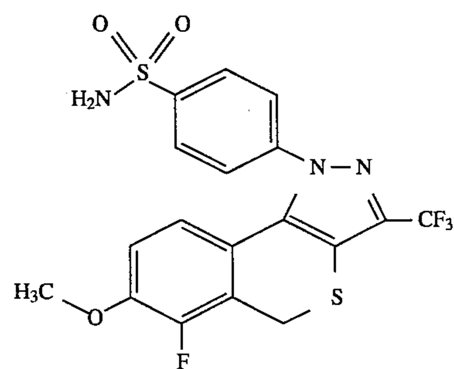
4-[1,5-Dihydro-6-fluoro-7-methoxy-3-(trifluoromethyl)-[2]benzothiopyrano[4,3-c]pyrazol-1-yl]benzenesulfonamide
