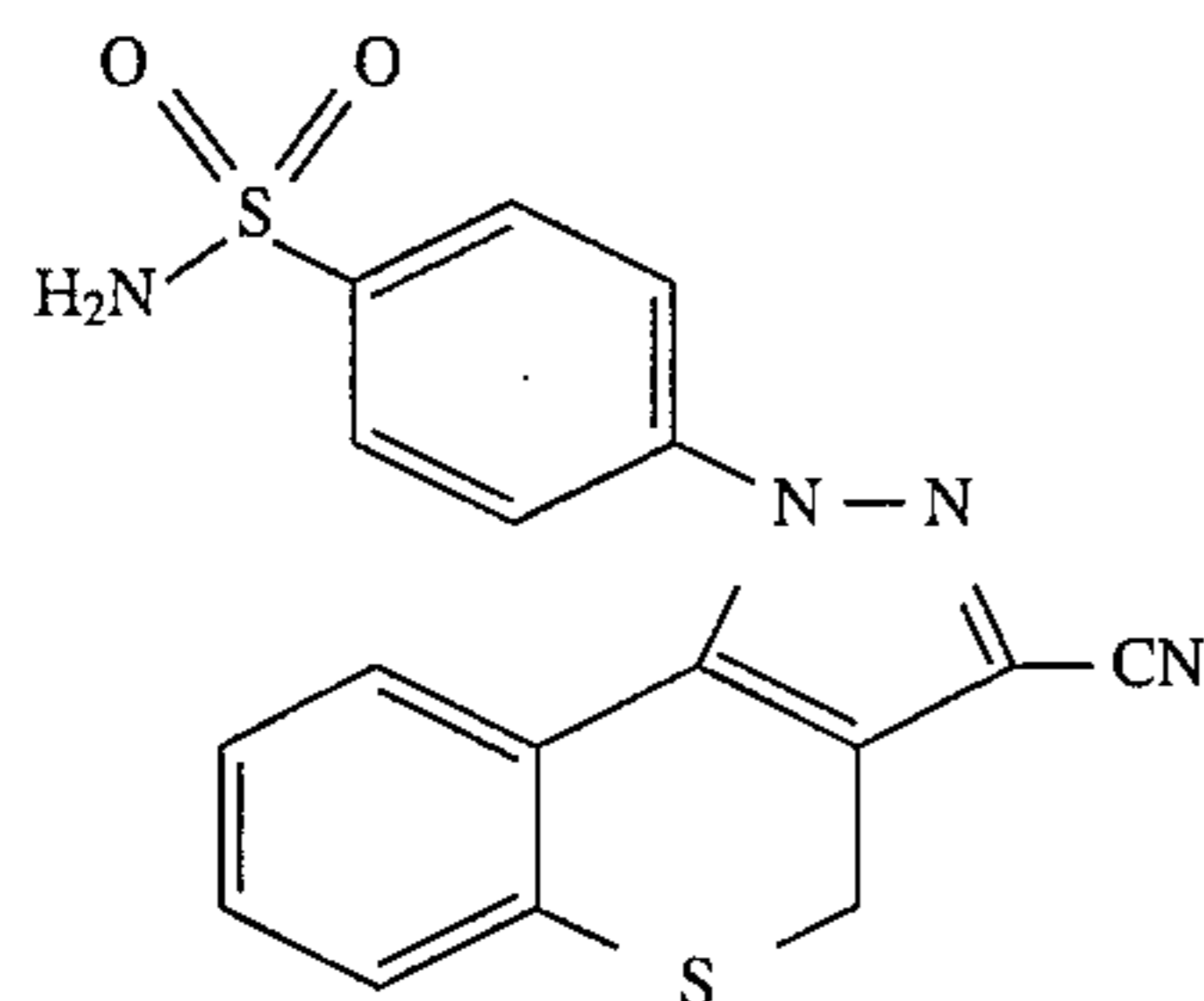
1-[4-(Aminosulfonyl)phenyl]-1,4-dihydro-[1]benzothiopyrano[4,3-c]pyrazol-3-carbonitrile
