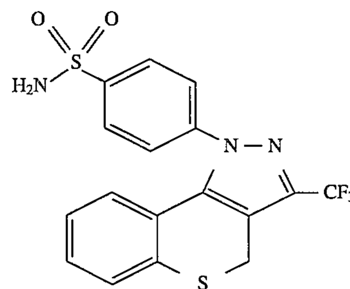
4-[1,4-Dihydro-3-(trifluoromethyl)-[1]benzothiopyrano[4,3-c]pyrazol-1-yl]benzenesulfonamide
