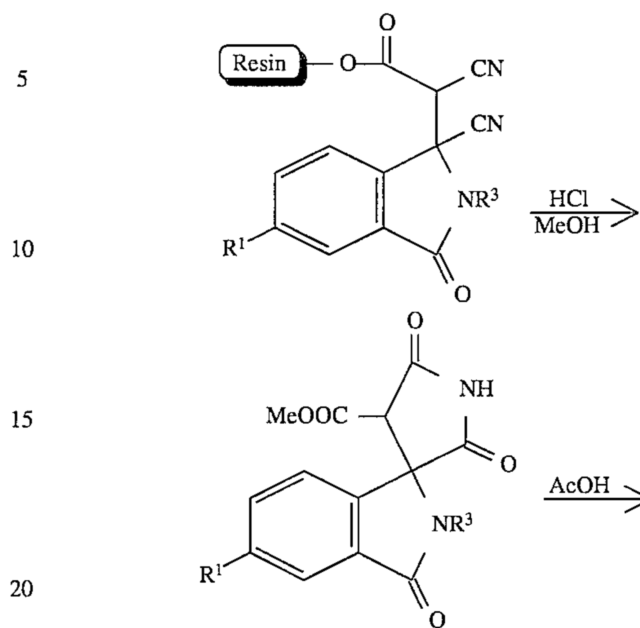
-continued SCHEME 12
