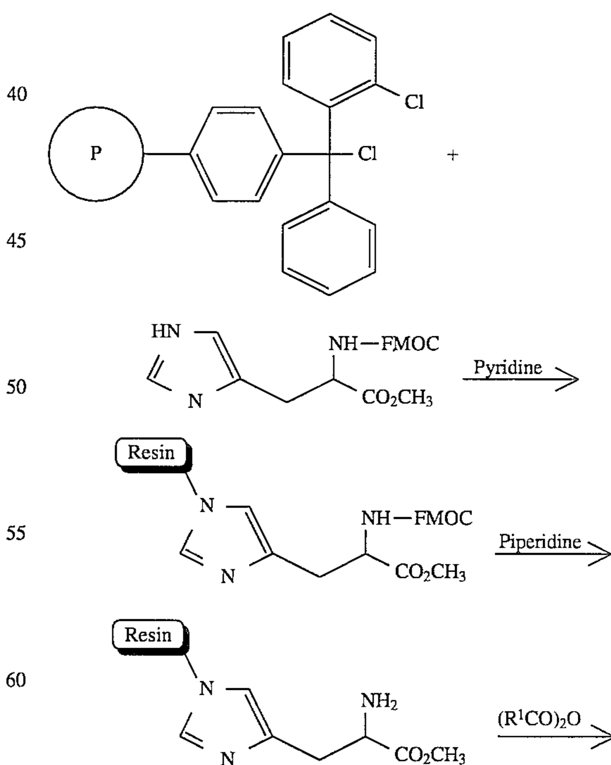
SCHEME 13
