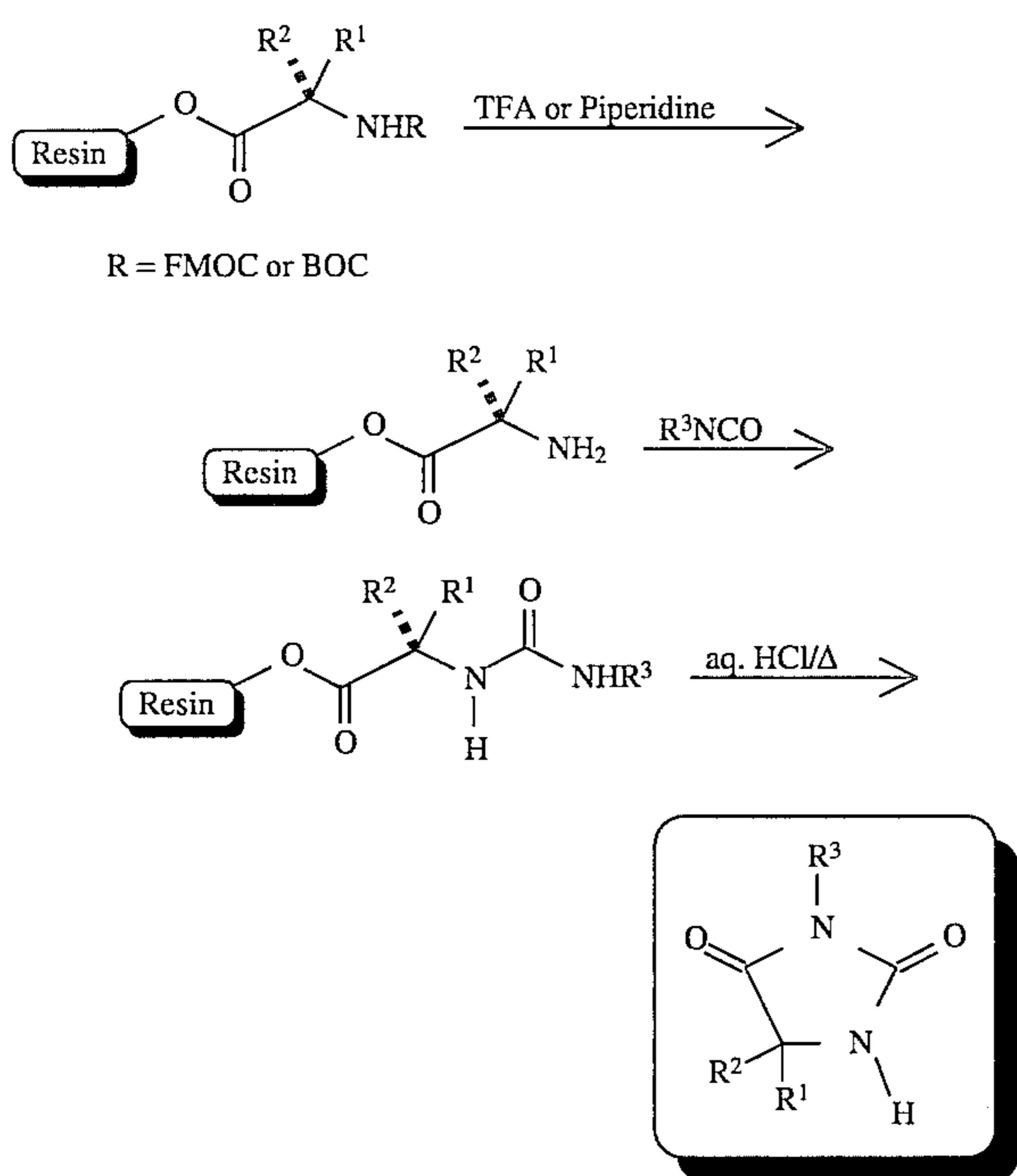
SCHEME 2
