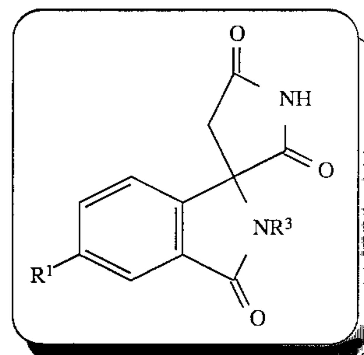
SCHEME 13
