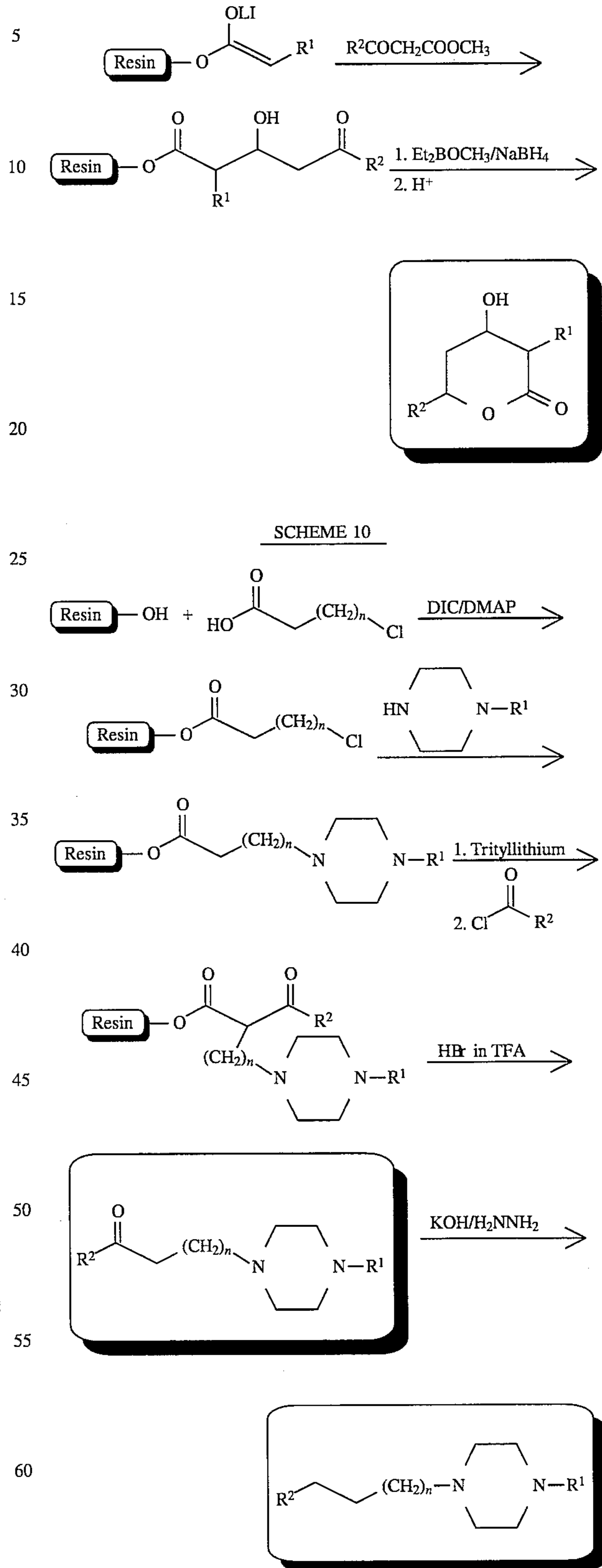
-continued SCHEME 9
