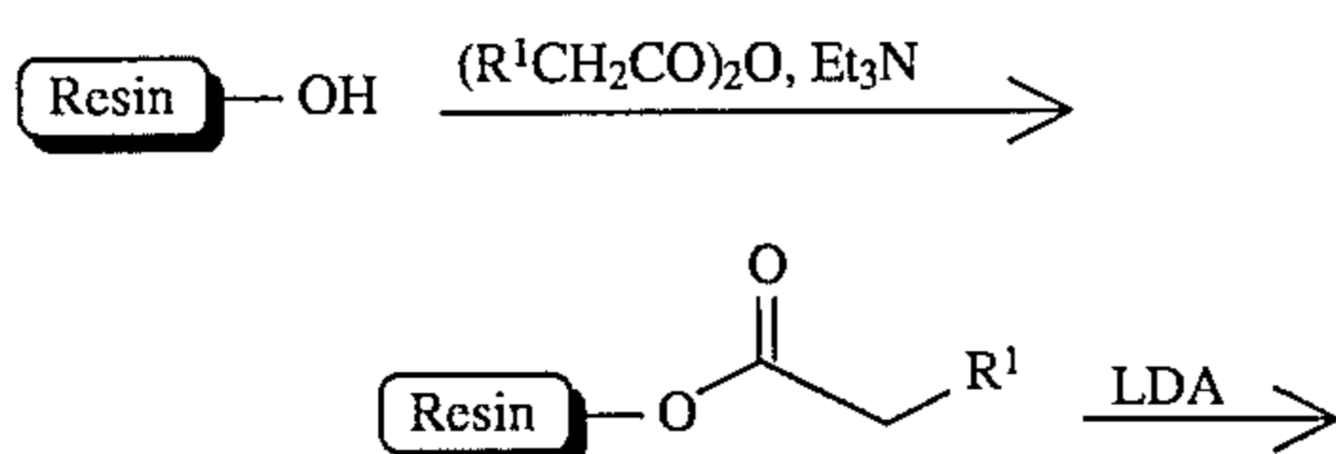
SCHEME 9
