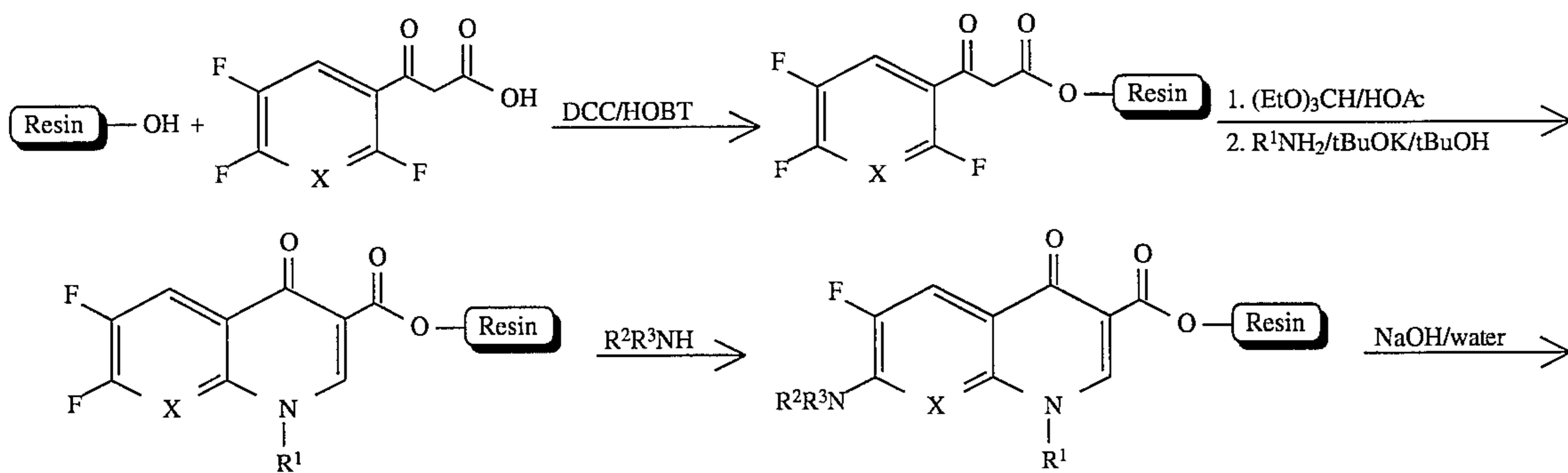
SCHEME 4
