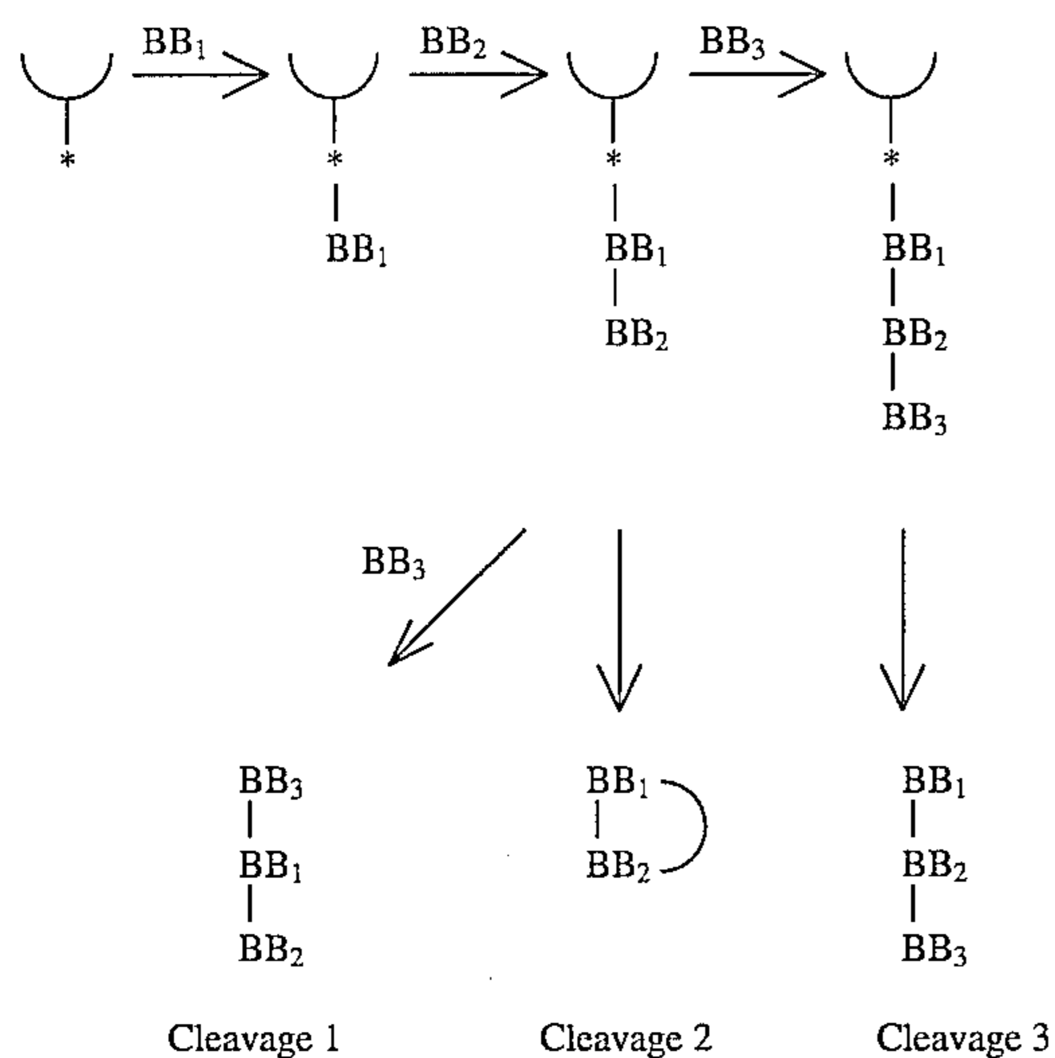
SCHEME 1
