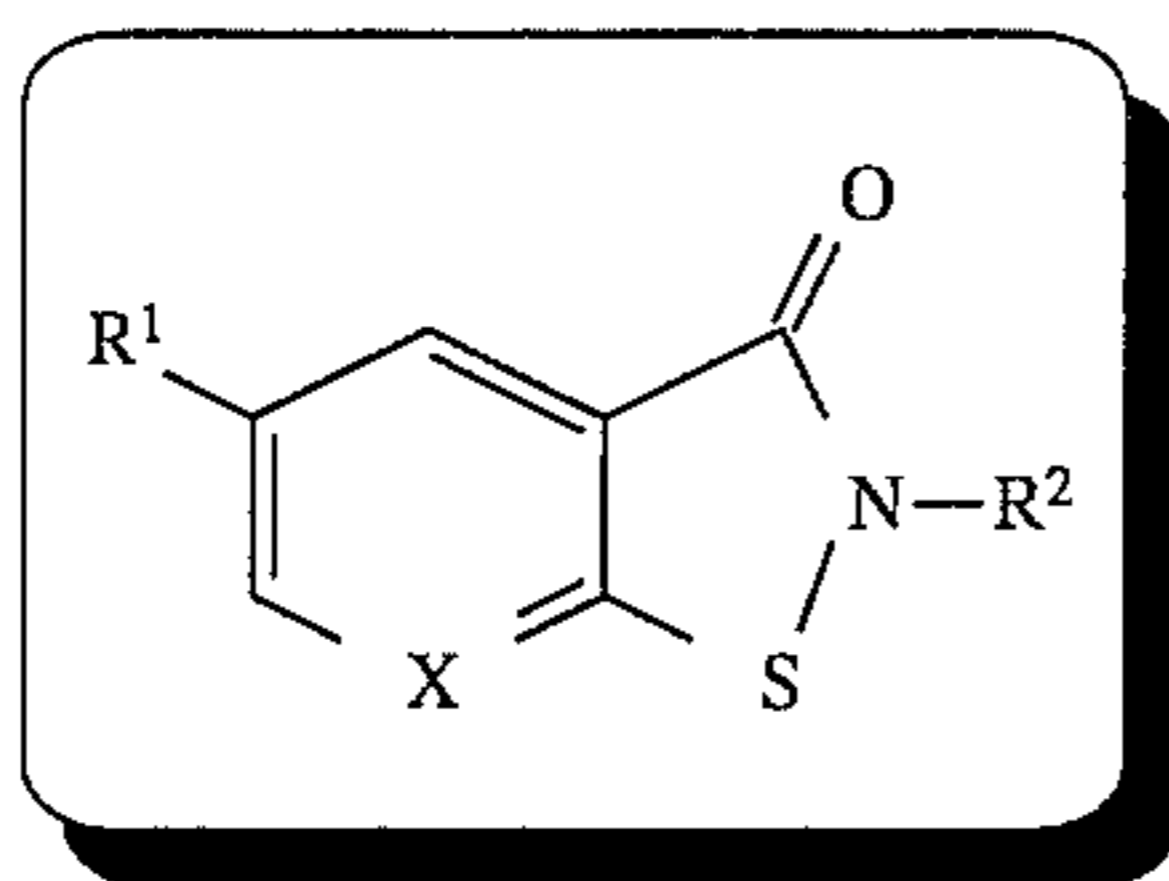
SCHEME 12
