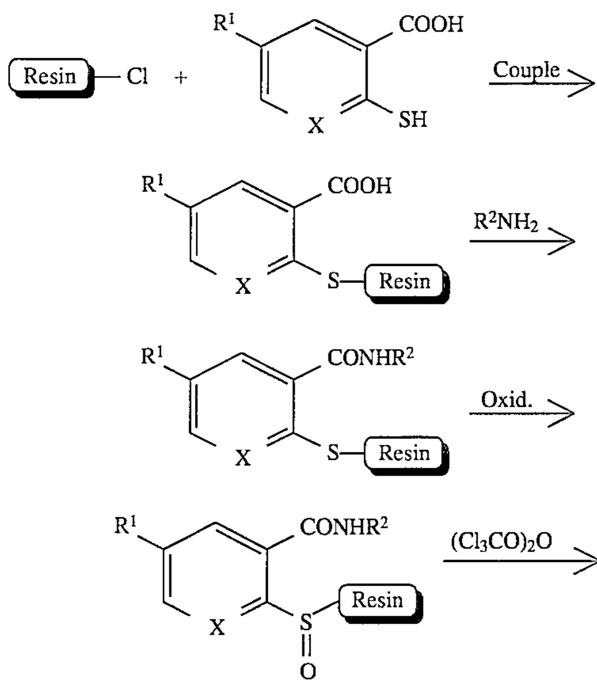
SCHEME 11
