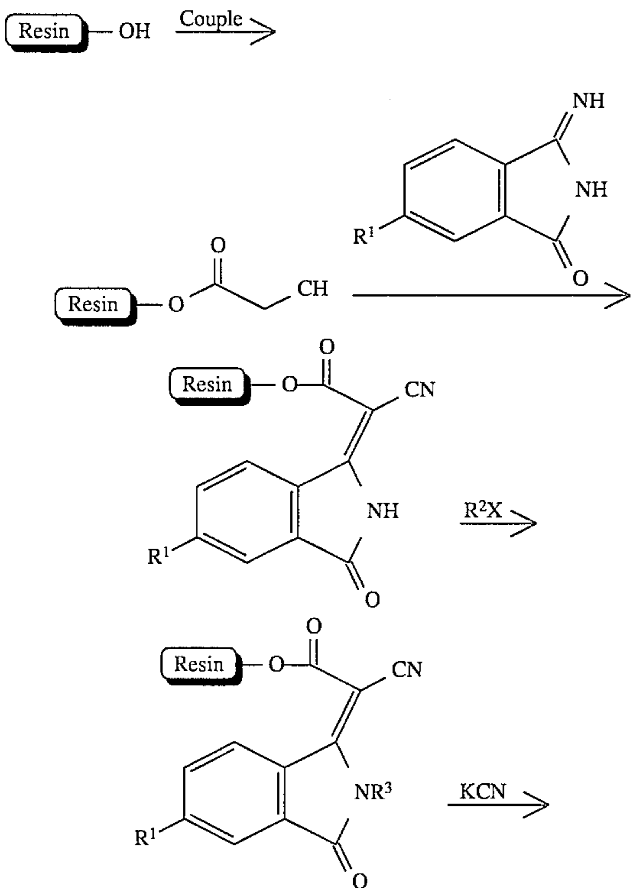
SCHEME 12
