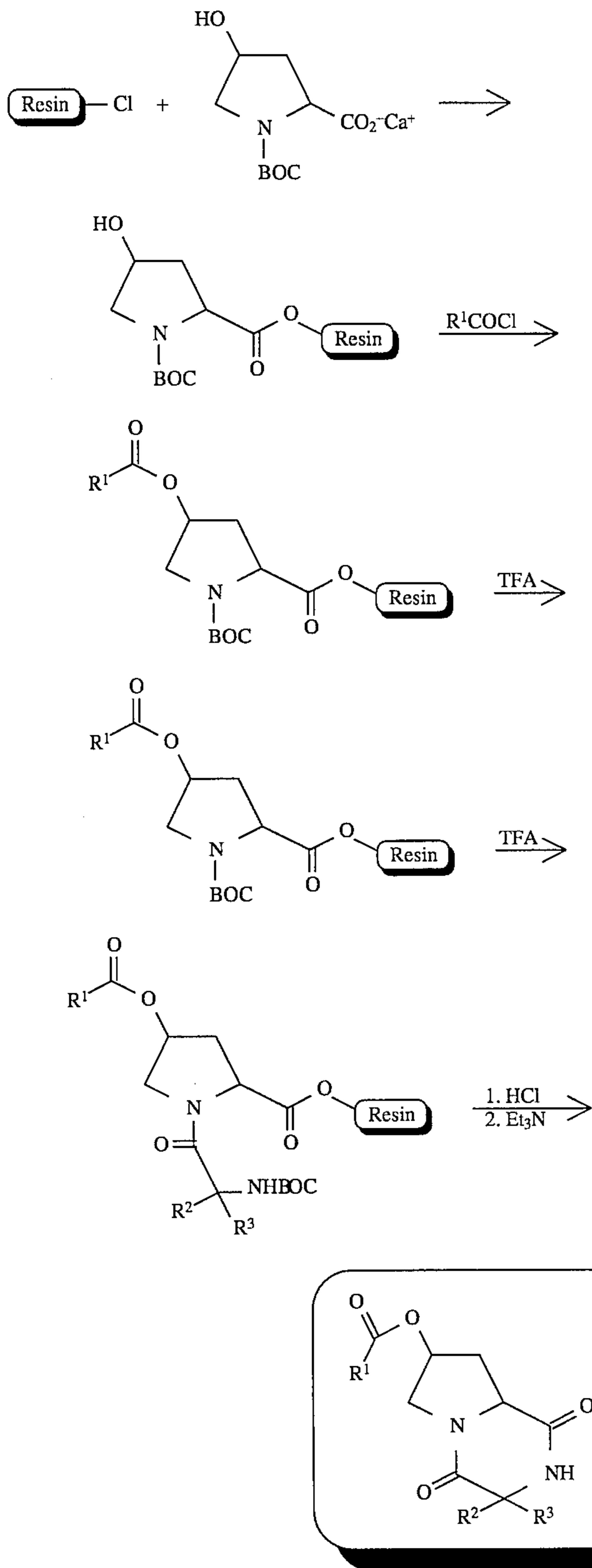
SCHEME 8
