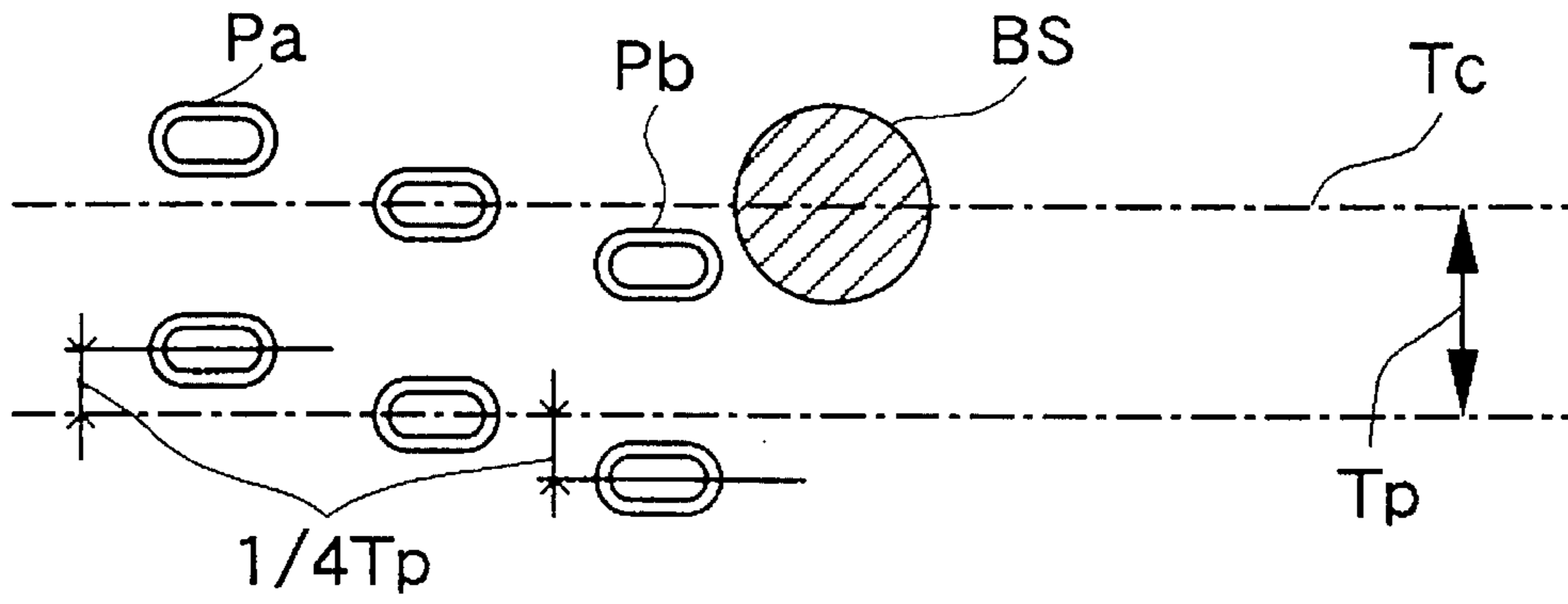
FIG.23 (PRIOR ART)
