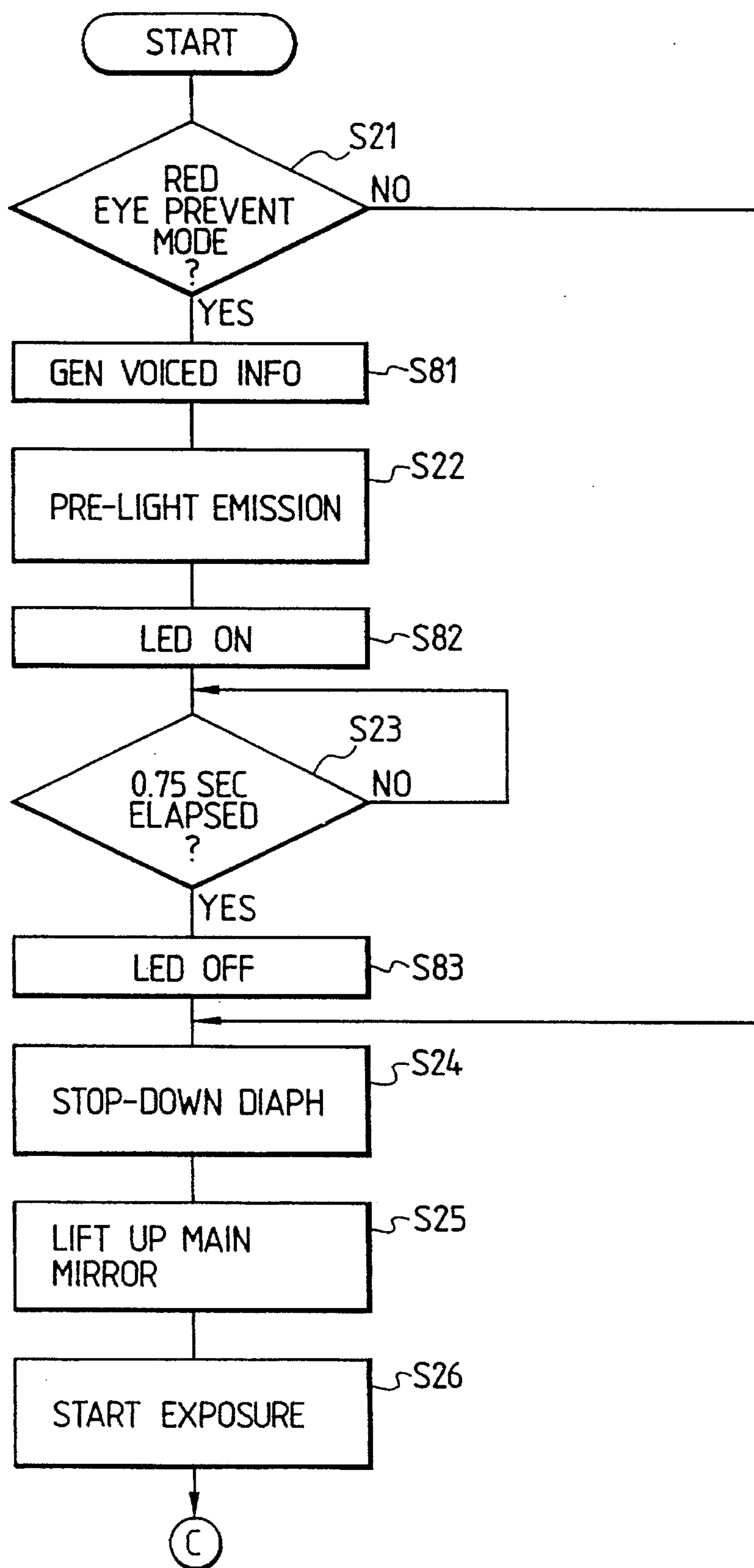
FIG. 12 INTERRUPT ROUTINE
