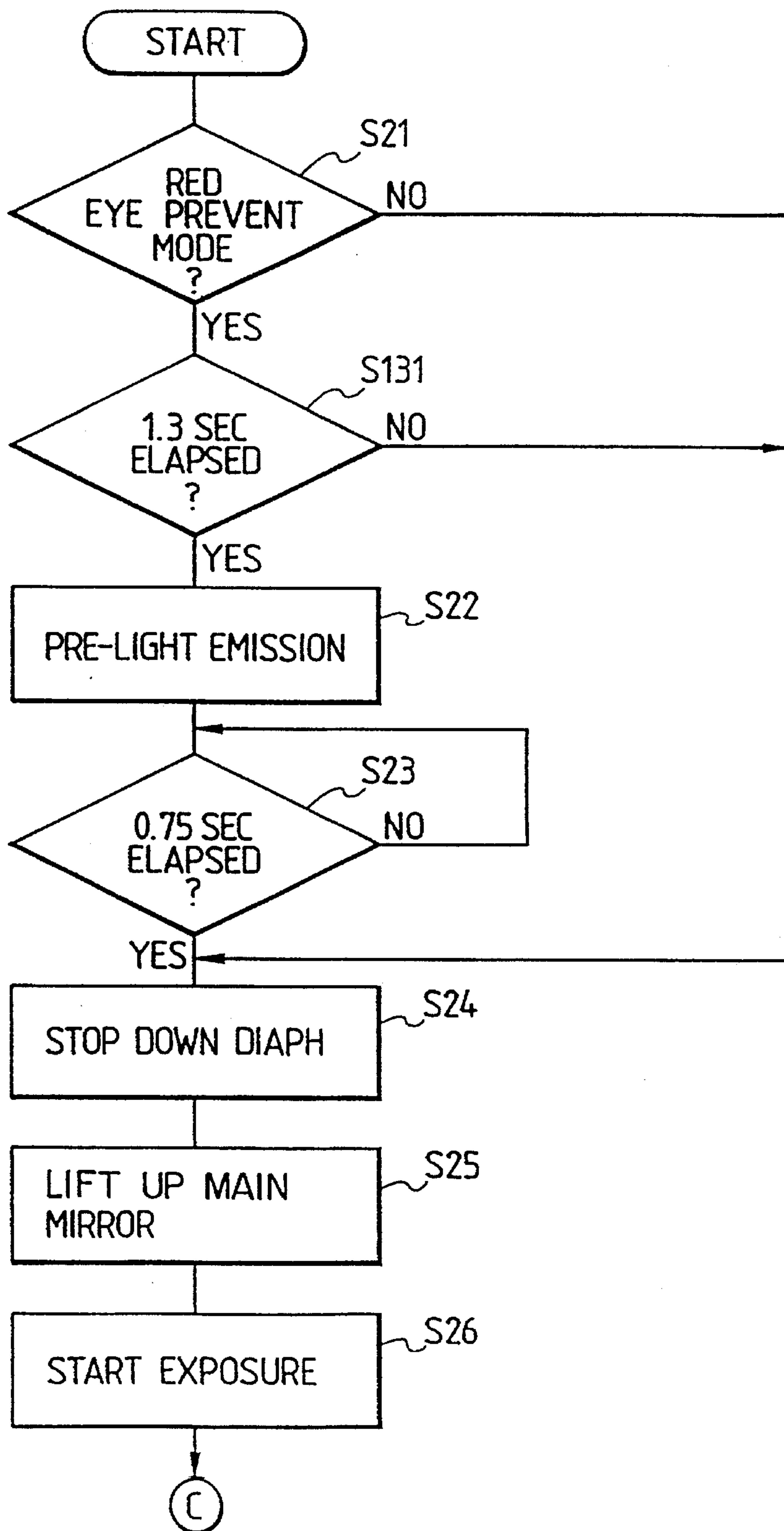
FIG. 20 INTERRUPT ROUTINE
