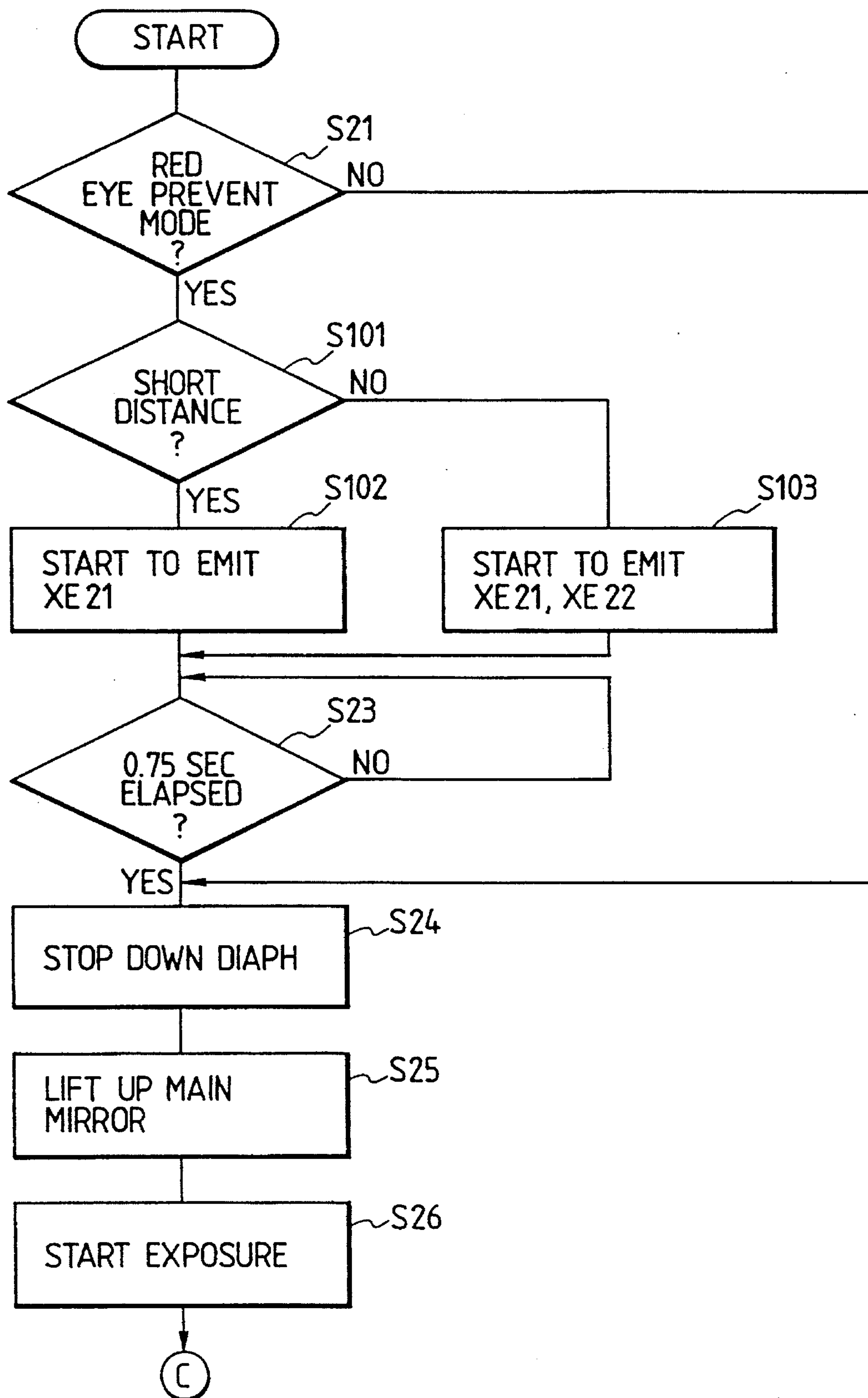
FIG. 16 INTERRUPT ROUTINE
