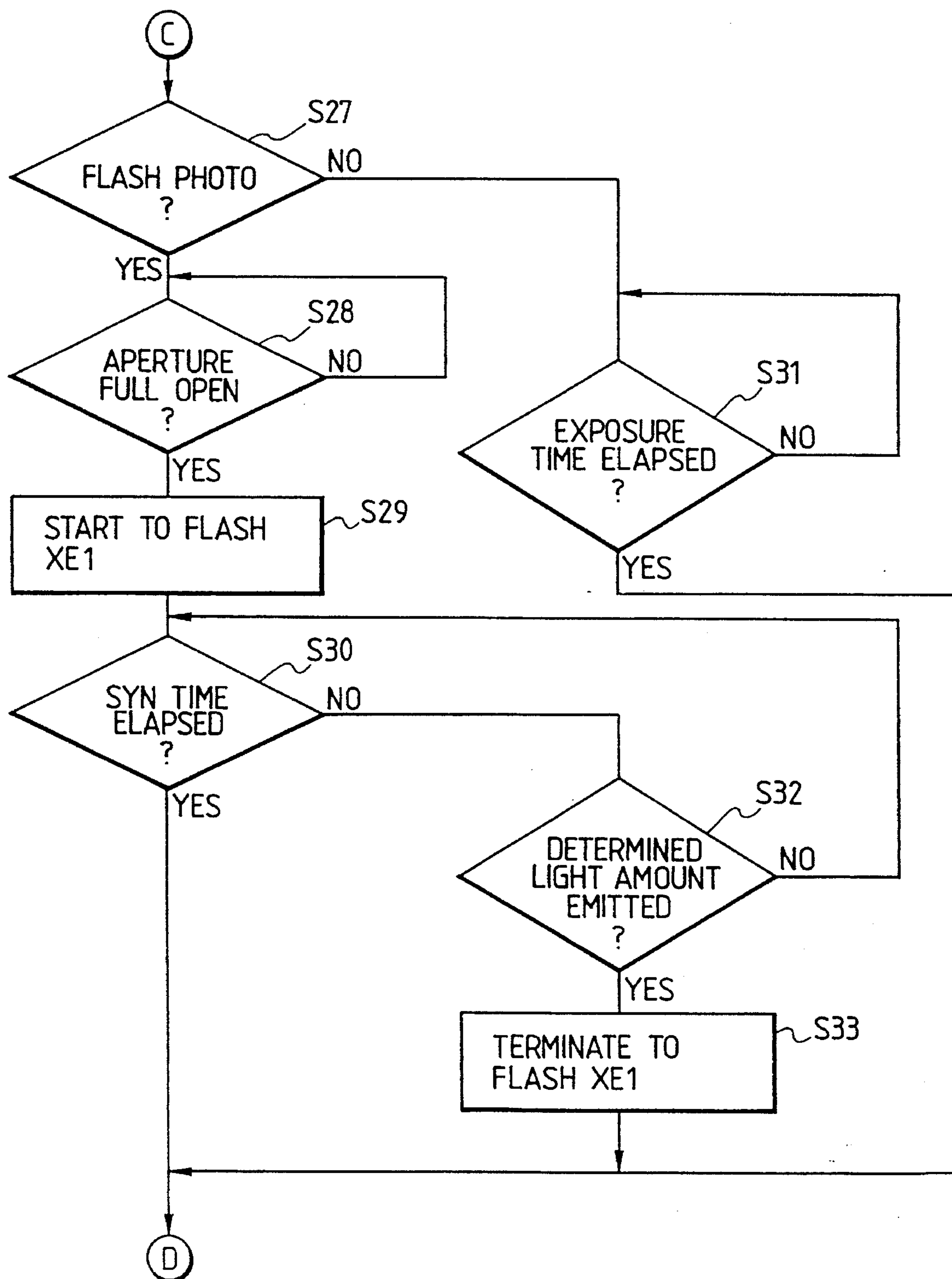
FIG. 6 INTERRUPT ROUTINE
