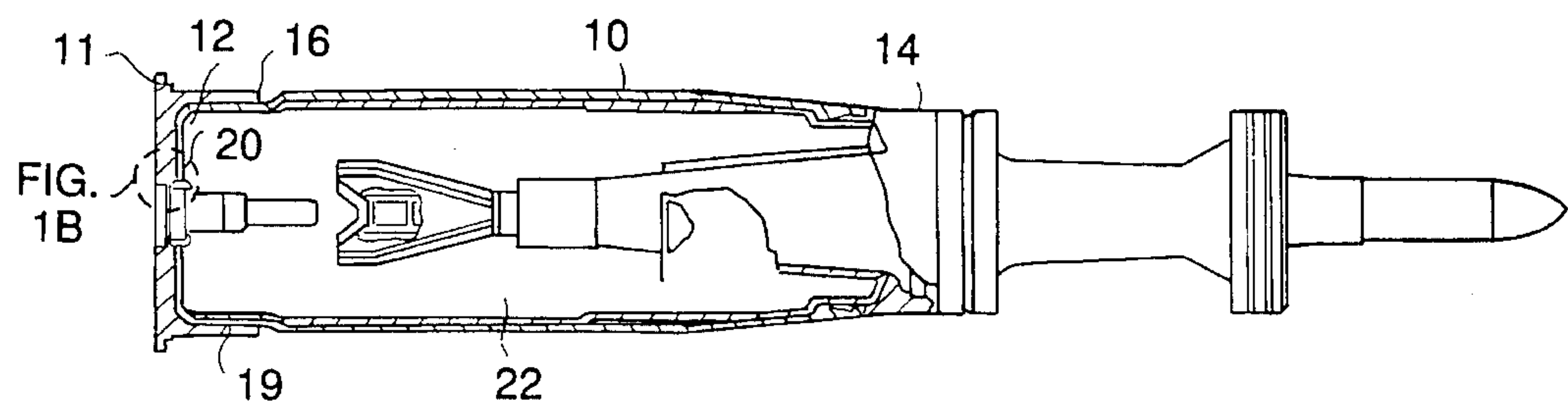
FIG. 1 (PRIOR ART)
