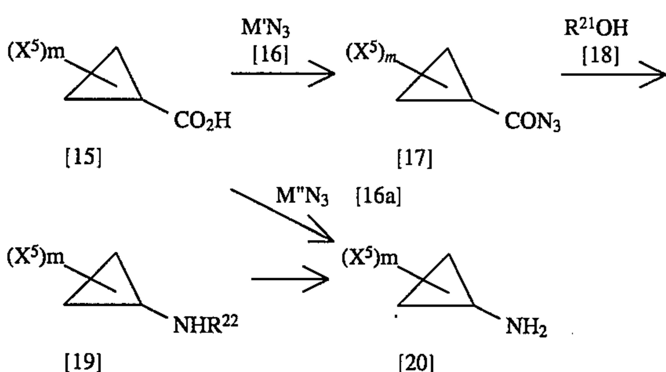
[Reaction scheme-VI]
