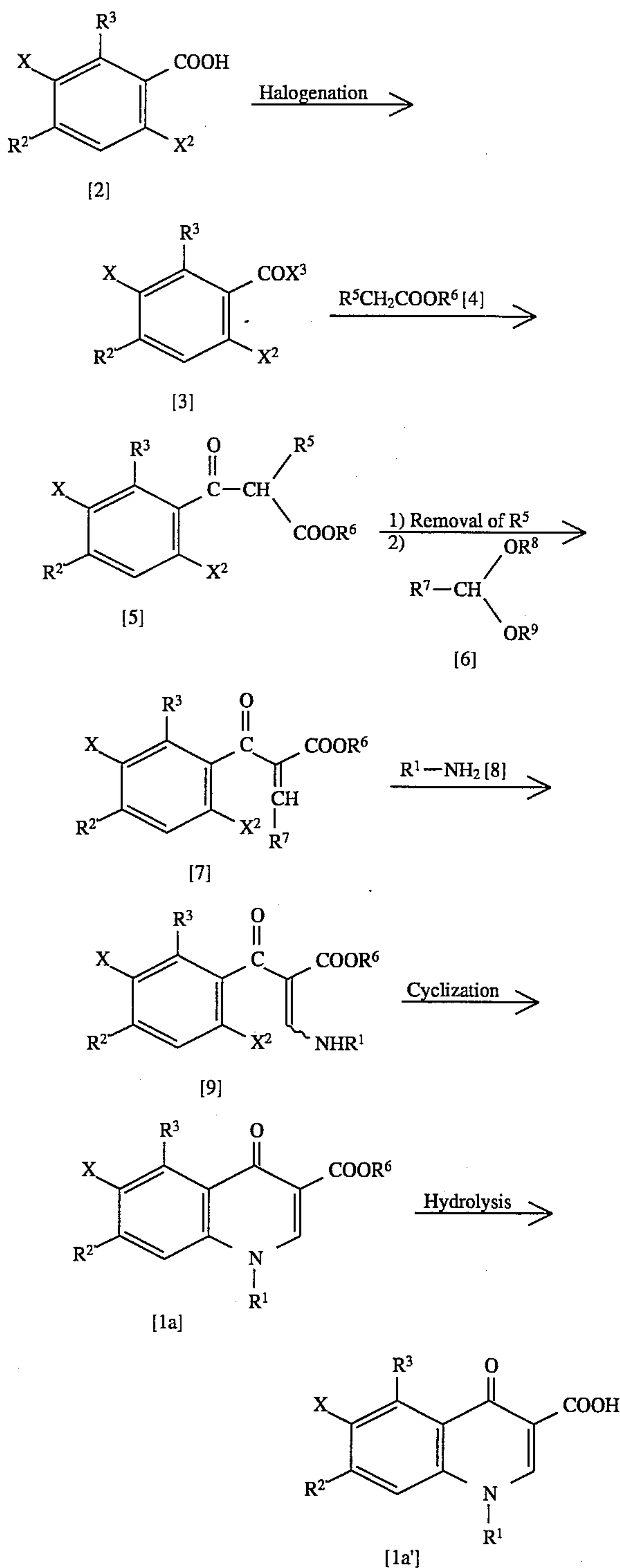
[Reaction scheme-I]
