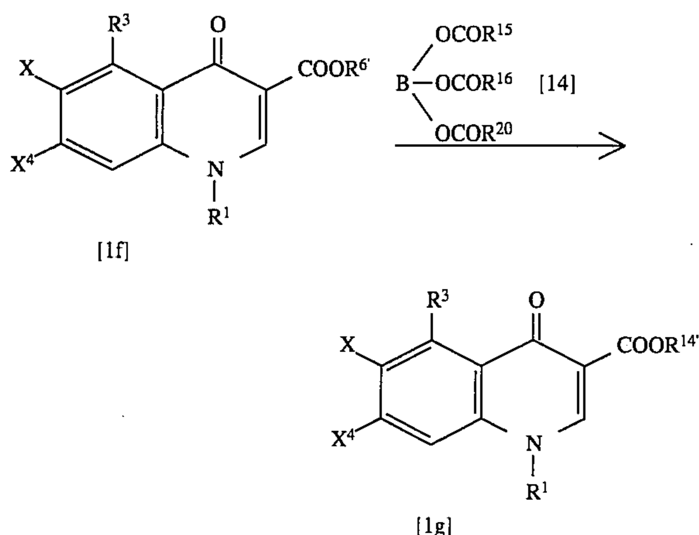
[Reaction scheme-V]
