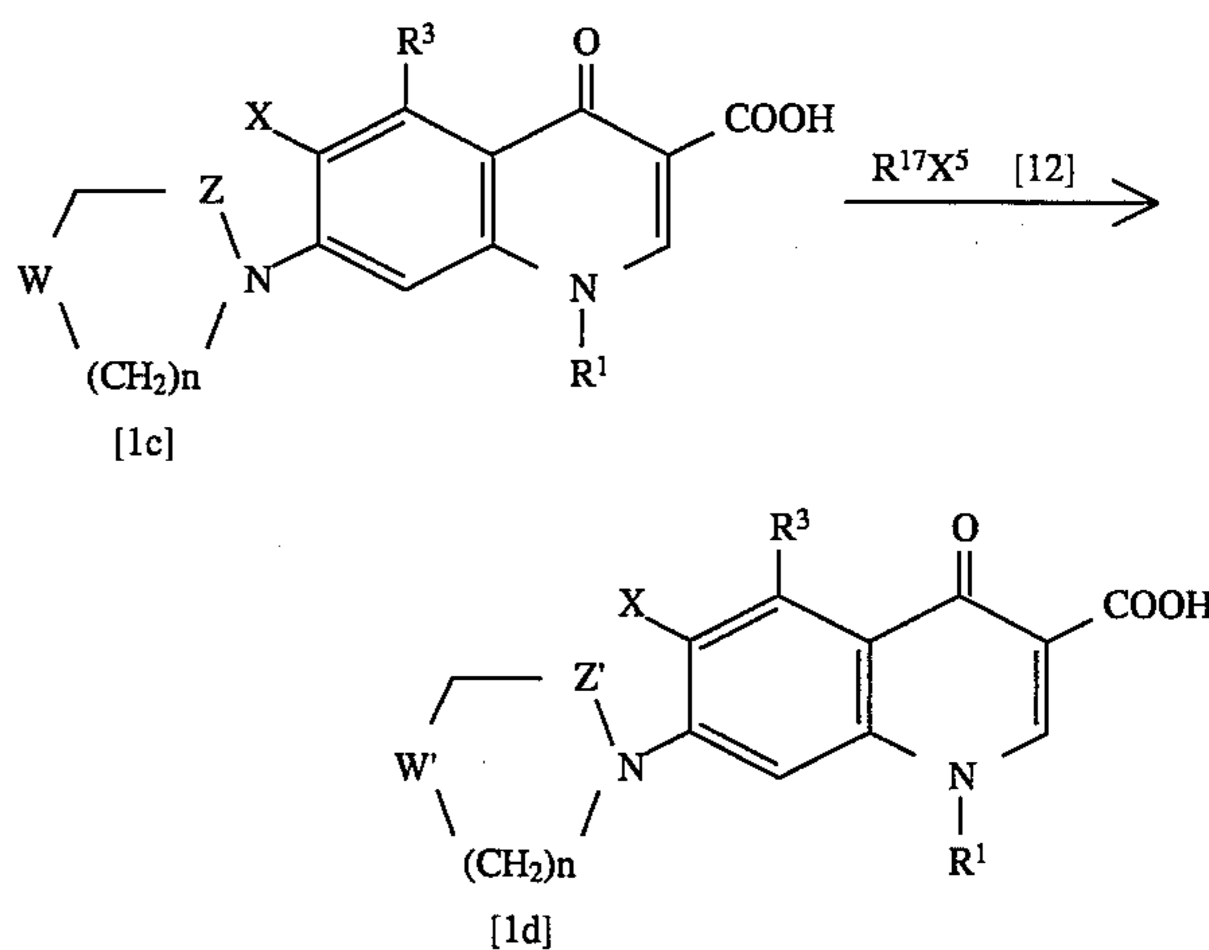
[Reaction scheme-III]
