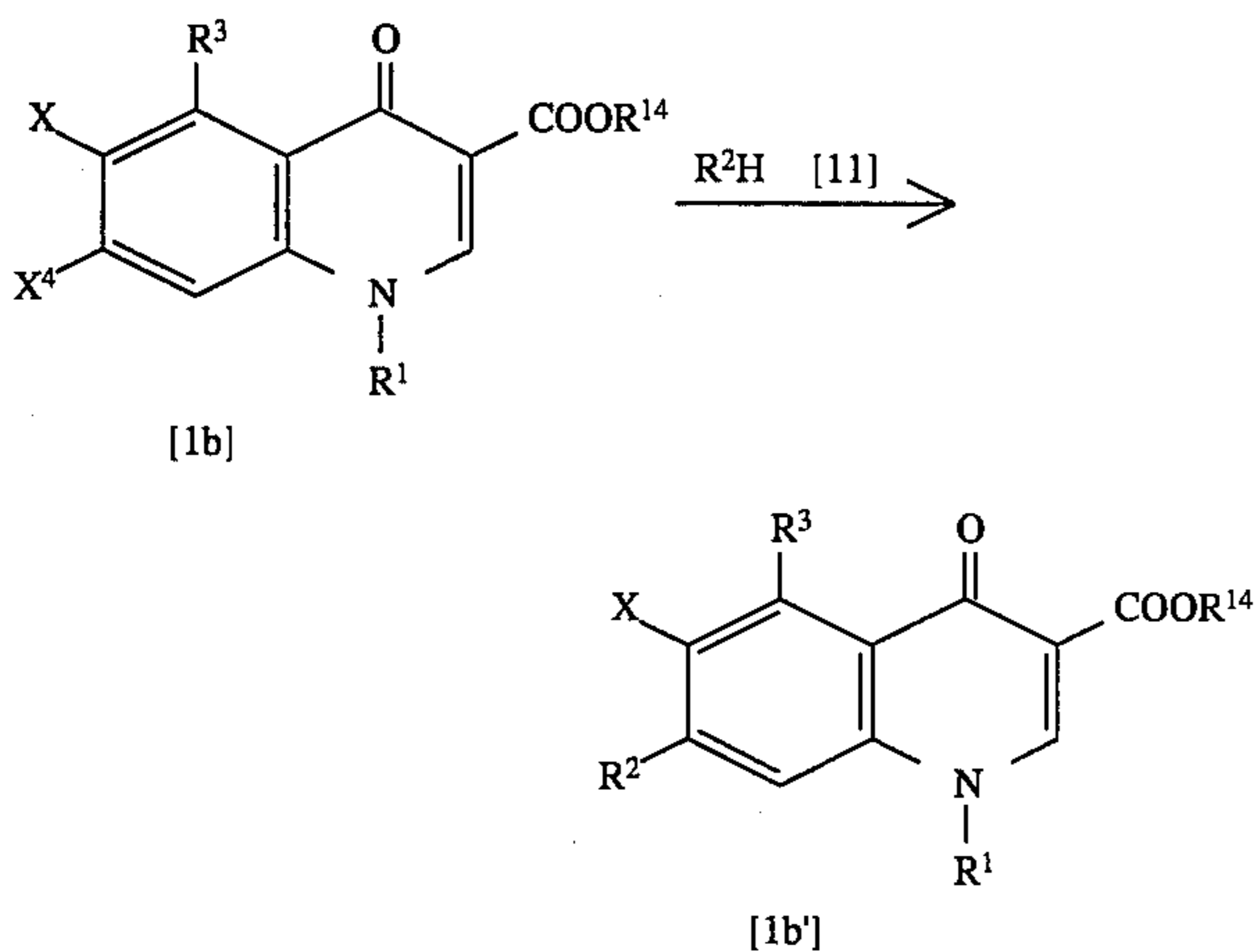
[Reaction Scheme-II]
