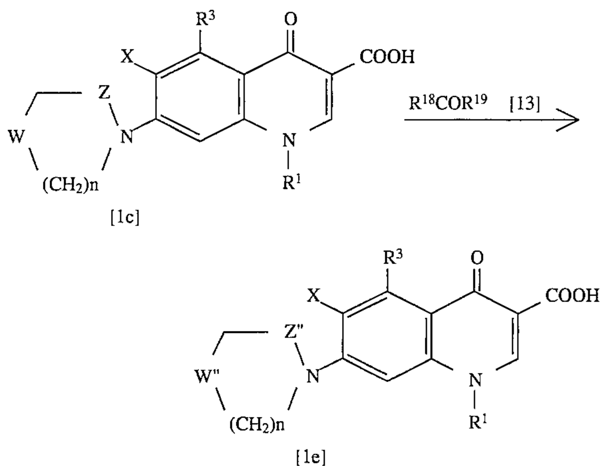
[Reaction scheme-IV]
