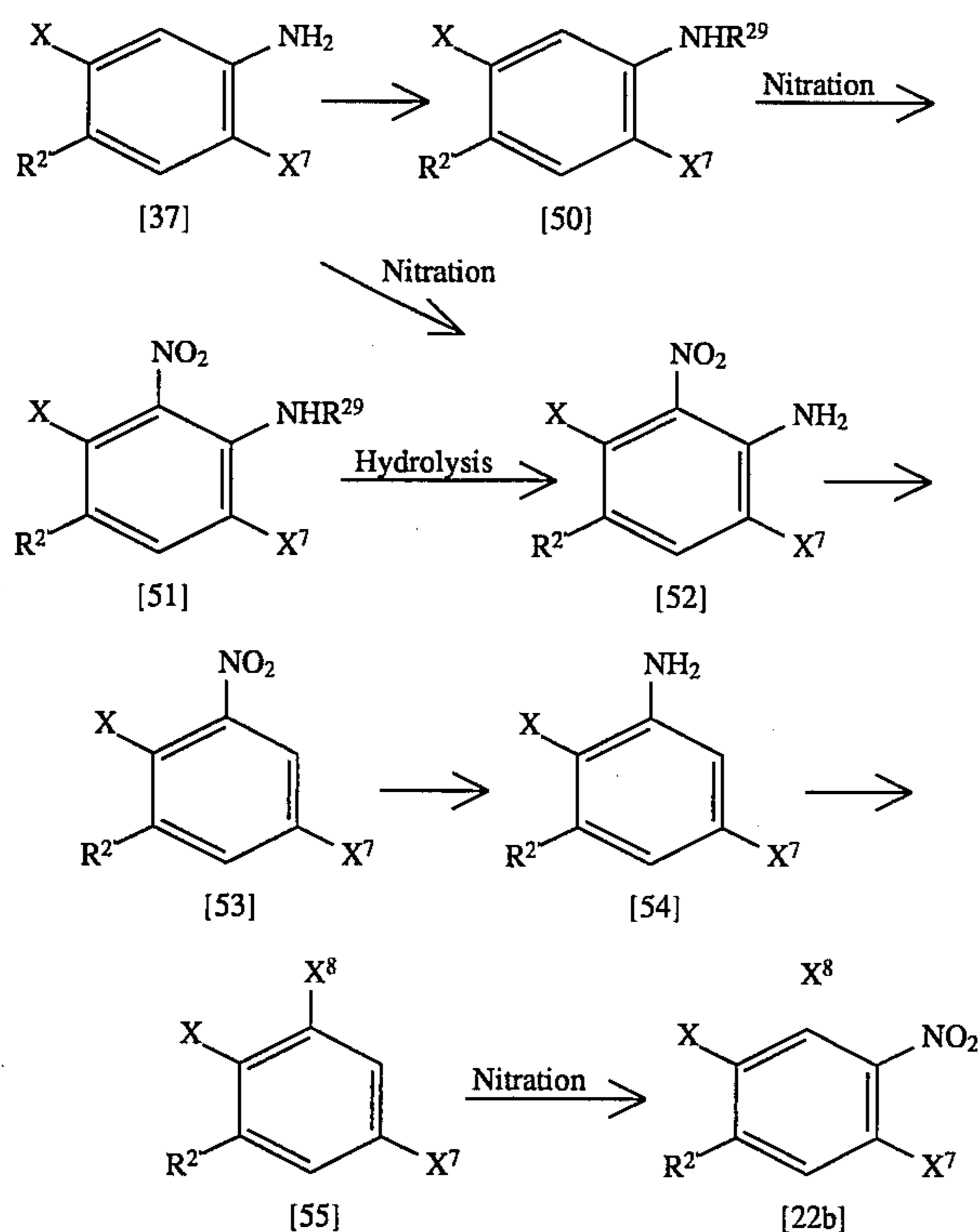
[Reaction scheme-XIII]
