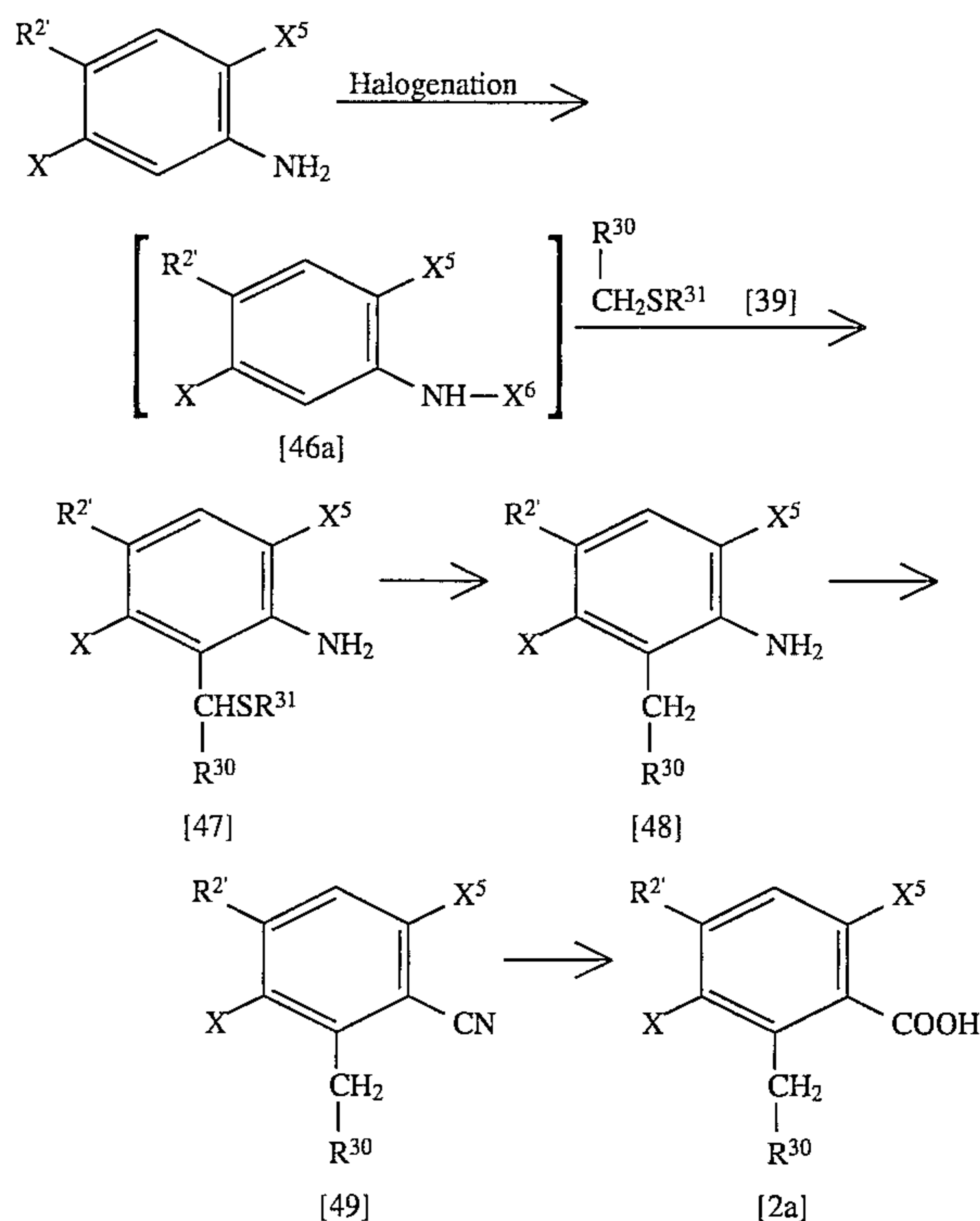
[Reaction scheme-XII]
