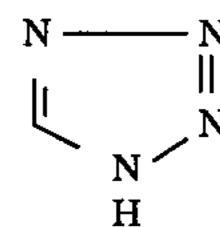
(c) 5-amino tetrazole monohydrate (Aldrich A8,060-2), of the formula
