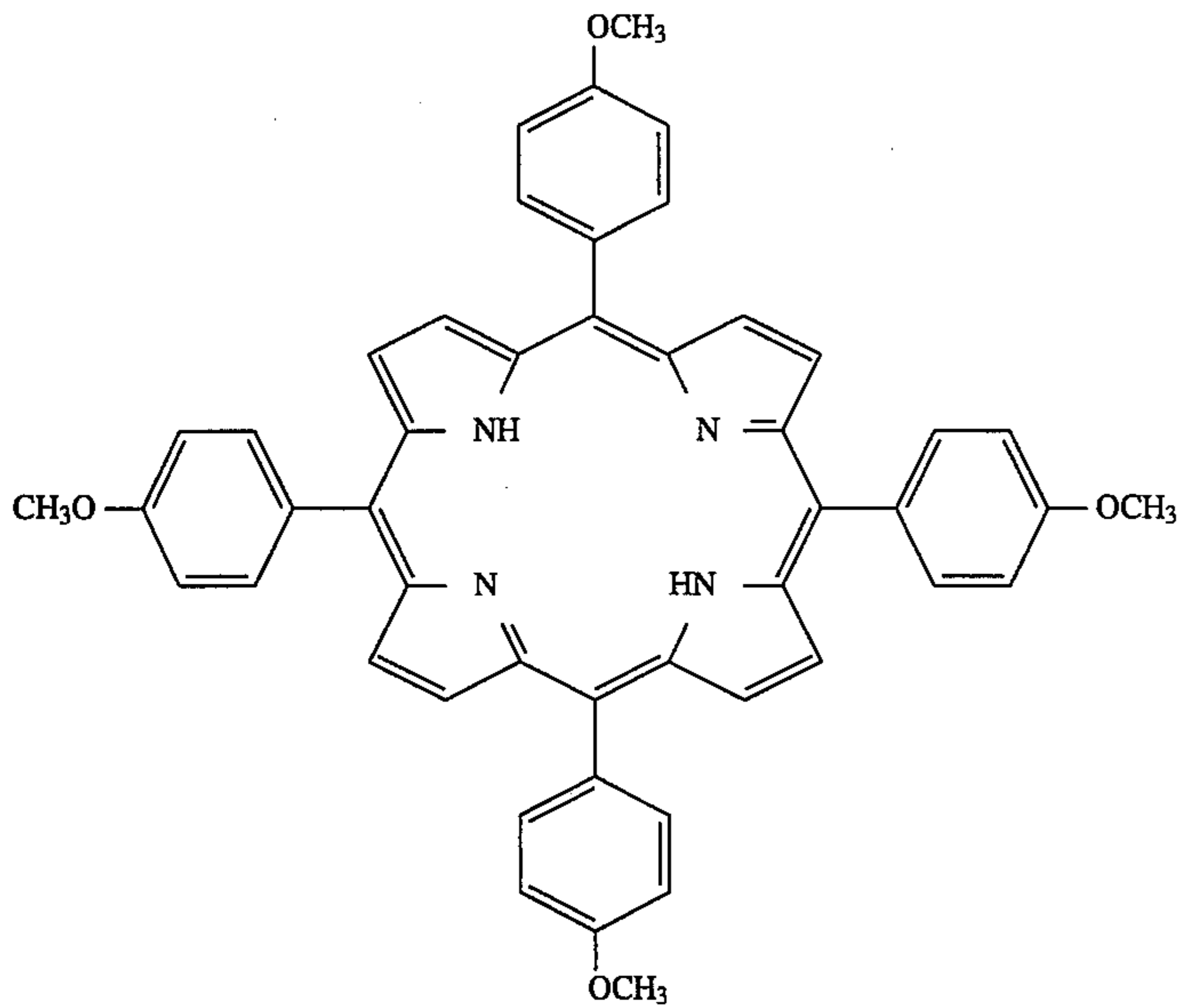
(f) 5,10,15,20-tetrakis(4-methoxyphenyl)-21H,23H-porphine (Aldrich 25,288-3), of the formula
