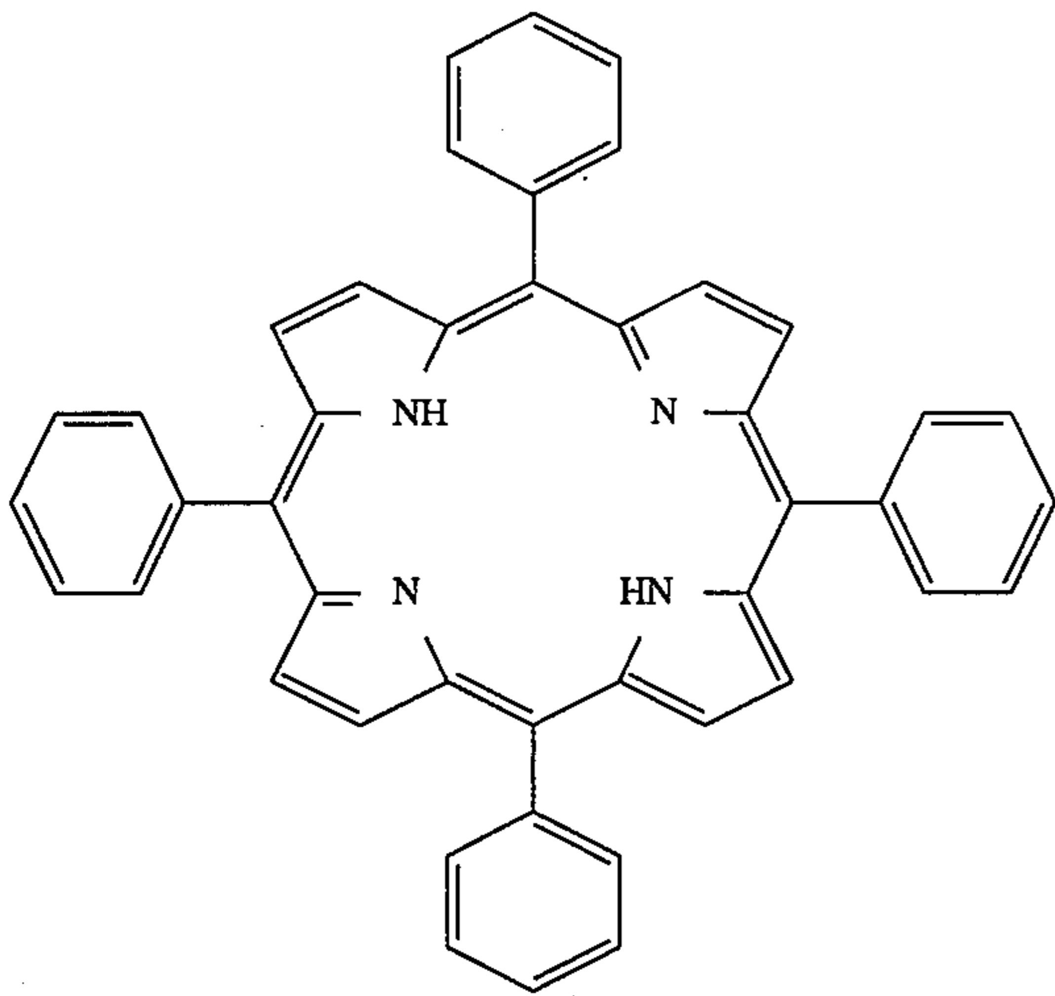
(e) 5,10,15,20-tetraphenyl-21H,23H-porphine (Aldrich 16,099-7), of the formula
