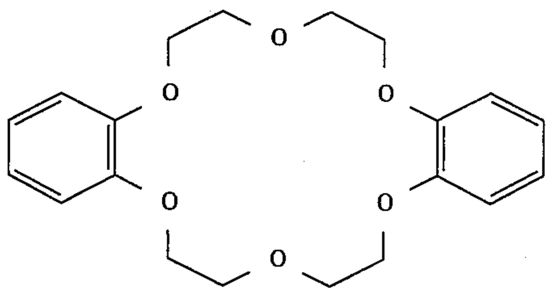
(18) di-tert-butyl-dibenzo-18-crown-6 (Aldrich 39,644-3), of the formula
