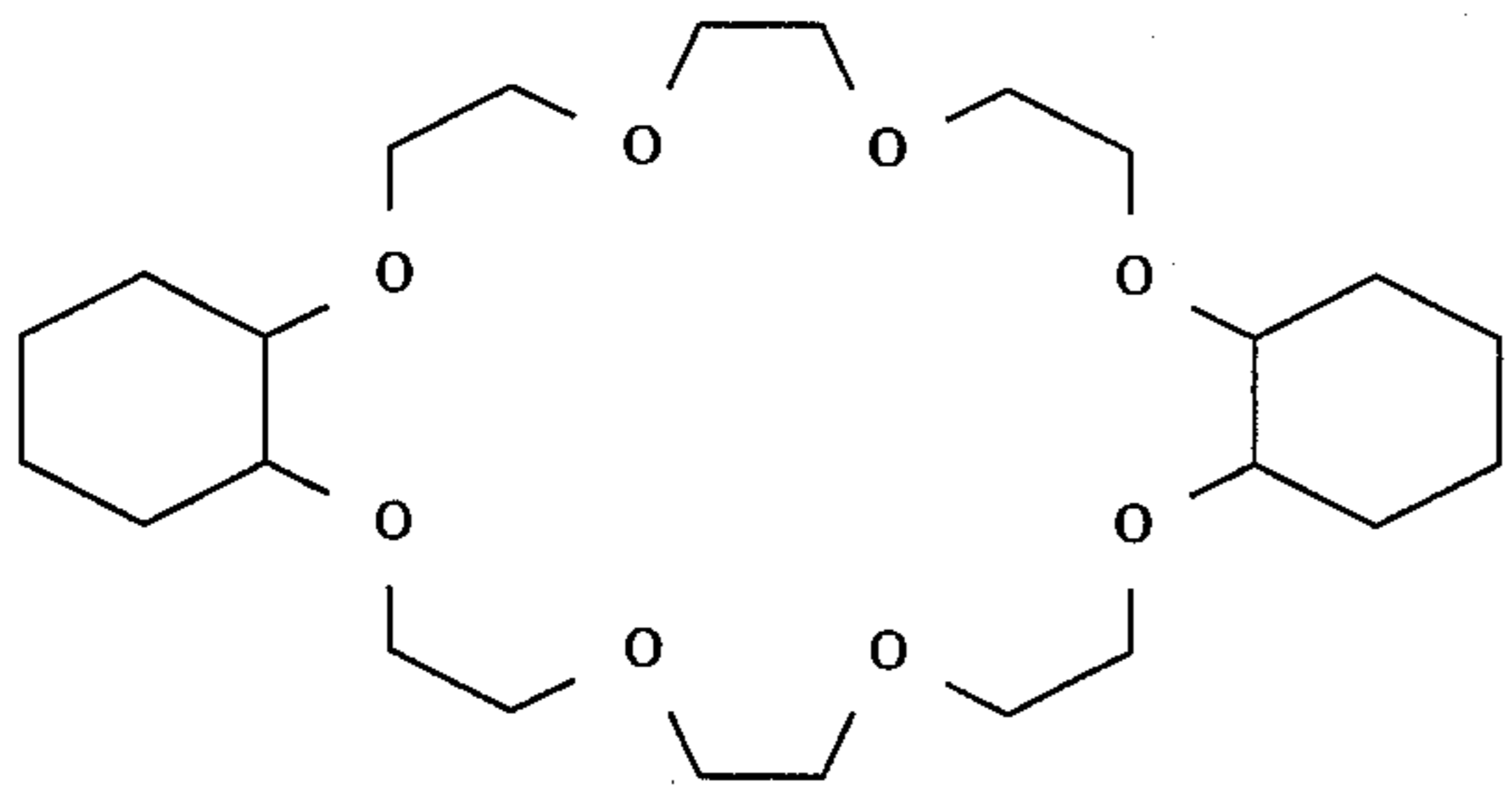
(22) dibenzo-30-crown-10,[2,3,17,18-dibenzo-1,4,7,10,13,16,19,22,25,28-decaoxacyclotriacontane-2,17-diene] (Aldrich
