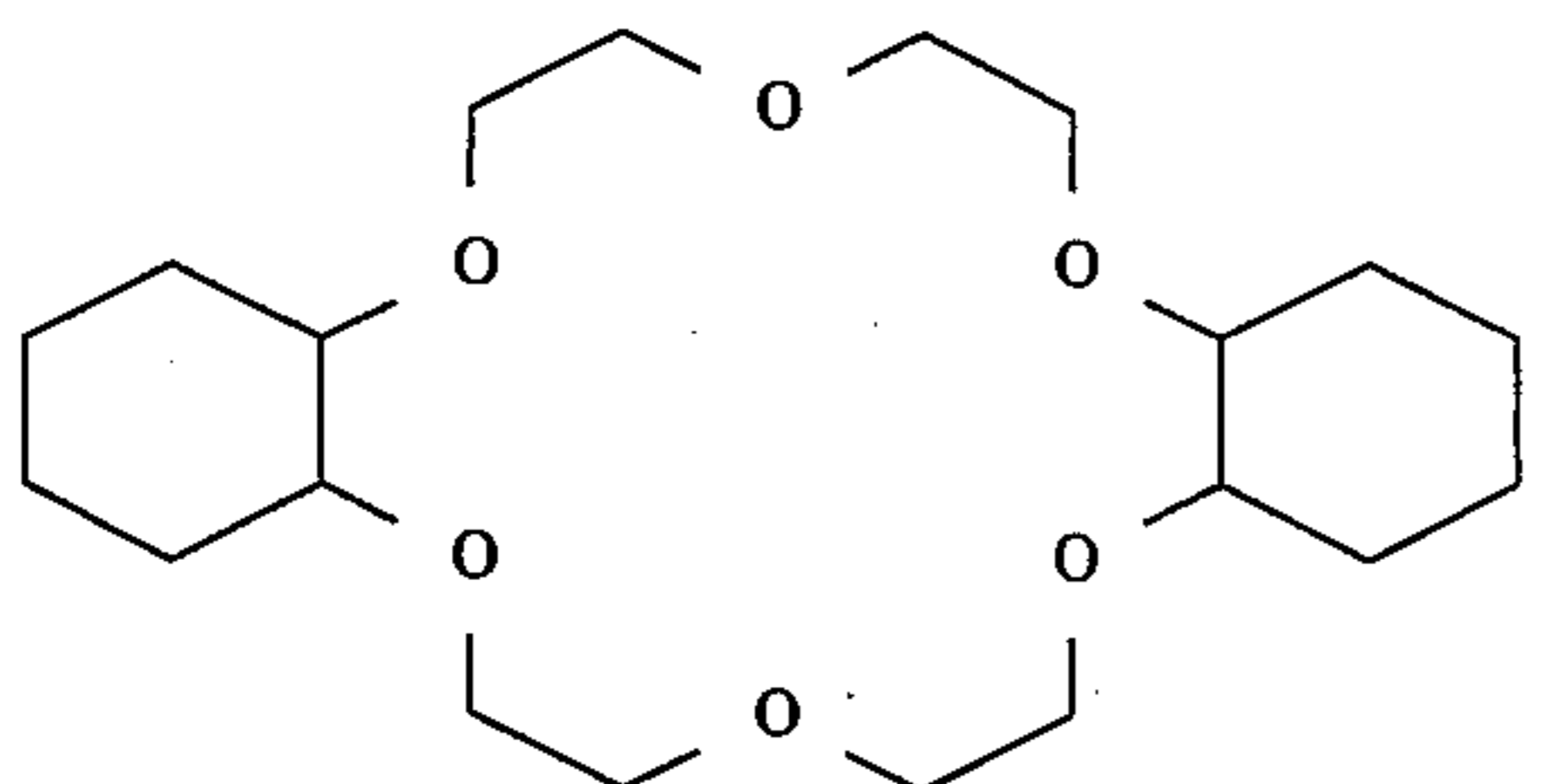
(20) dibenzo-24-crown-8[2,3,14,15-dibenzo-1,4,7,10,13,16,19,22-octaoxacyclotetracosane 2,14-diene] (Aldrich 25,319-7), of the formula
