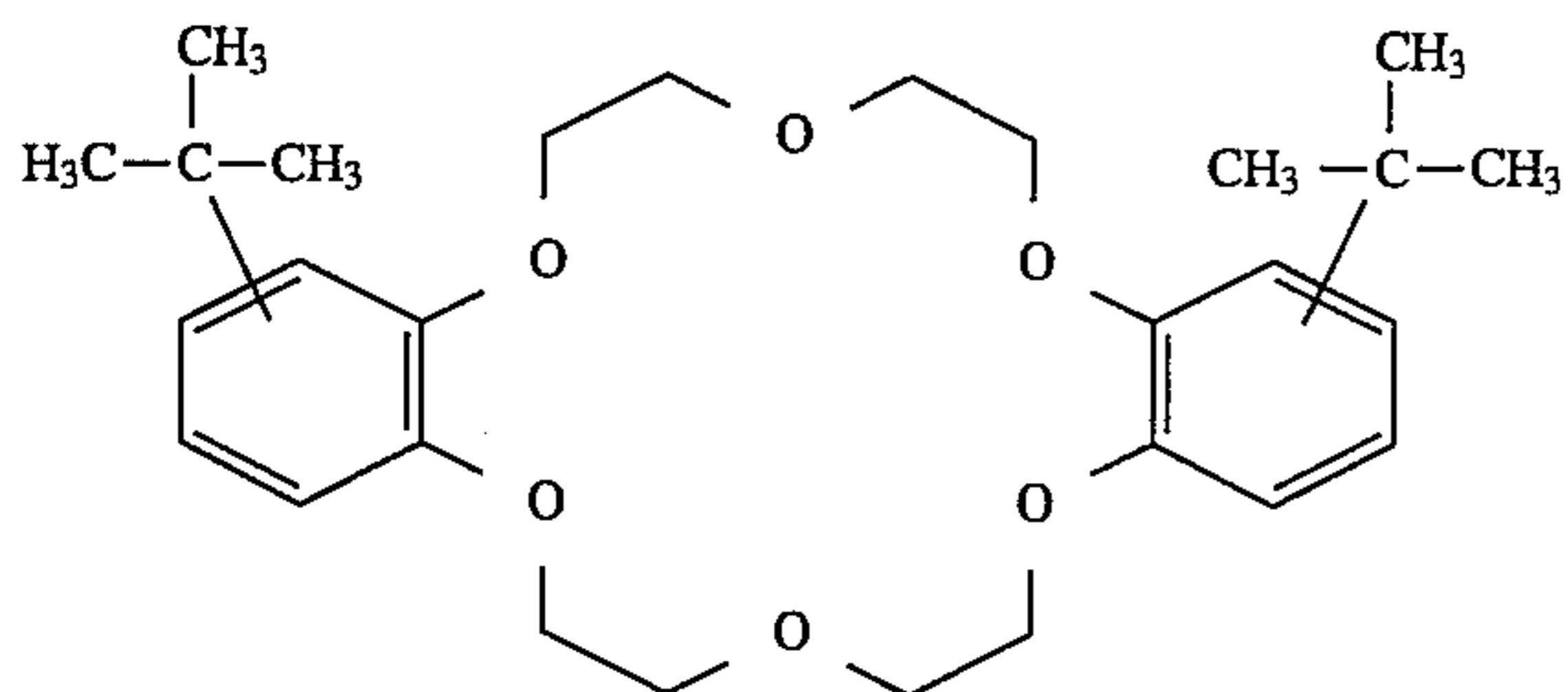
(19) cis-dicyclohexane-18-crown-6 (2,3,11,12-dicyclohexano-1,4,7,10,13,16-hexaoxacyclooctadecane) (Aldrich 15,840-2), of the formula
