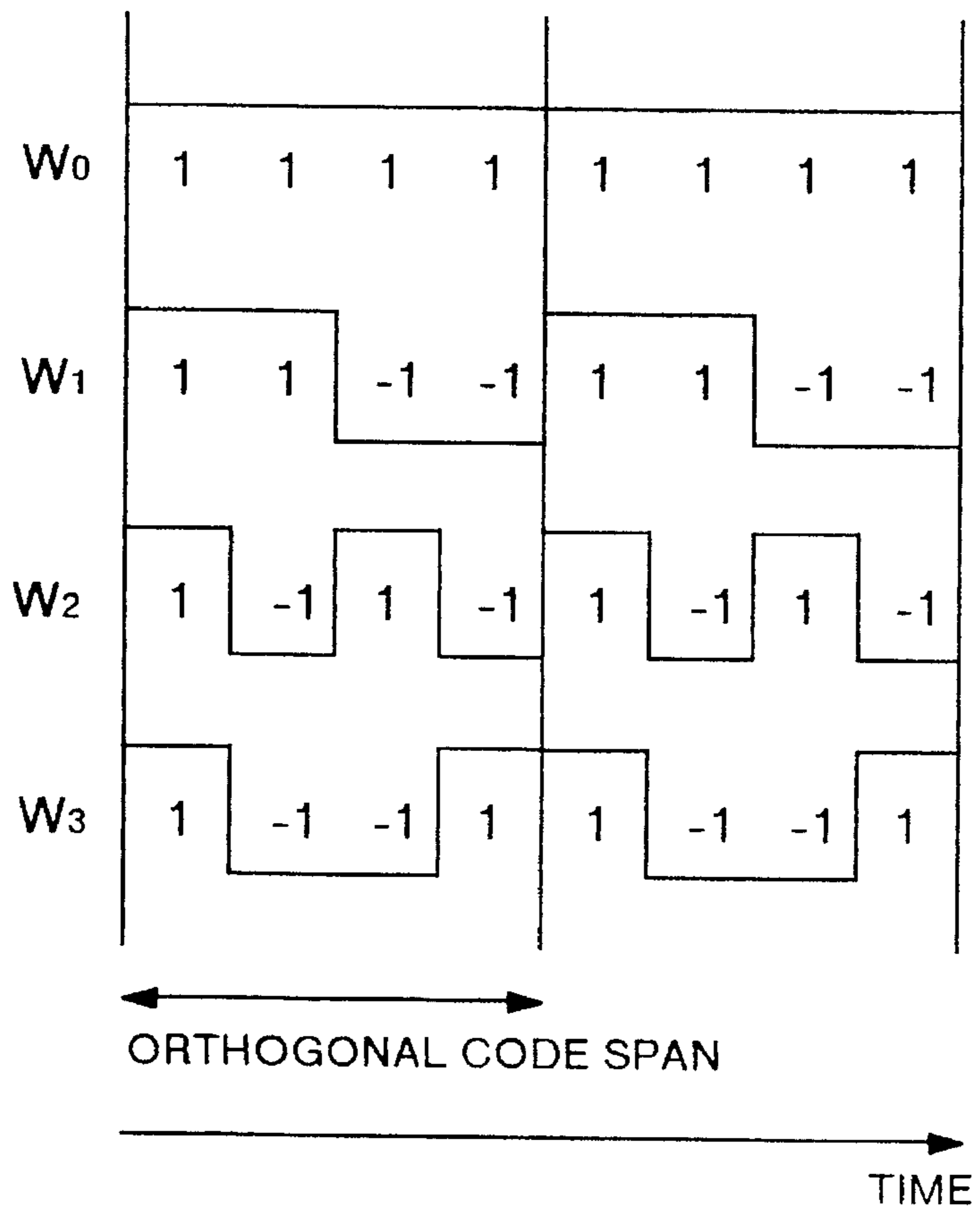
FIG.10 PRIOR ART
