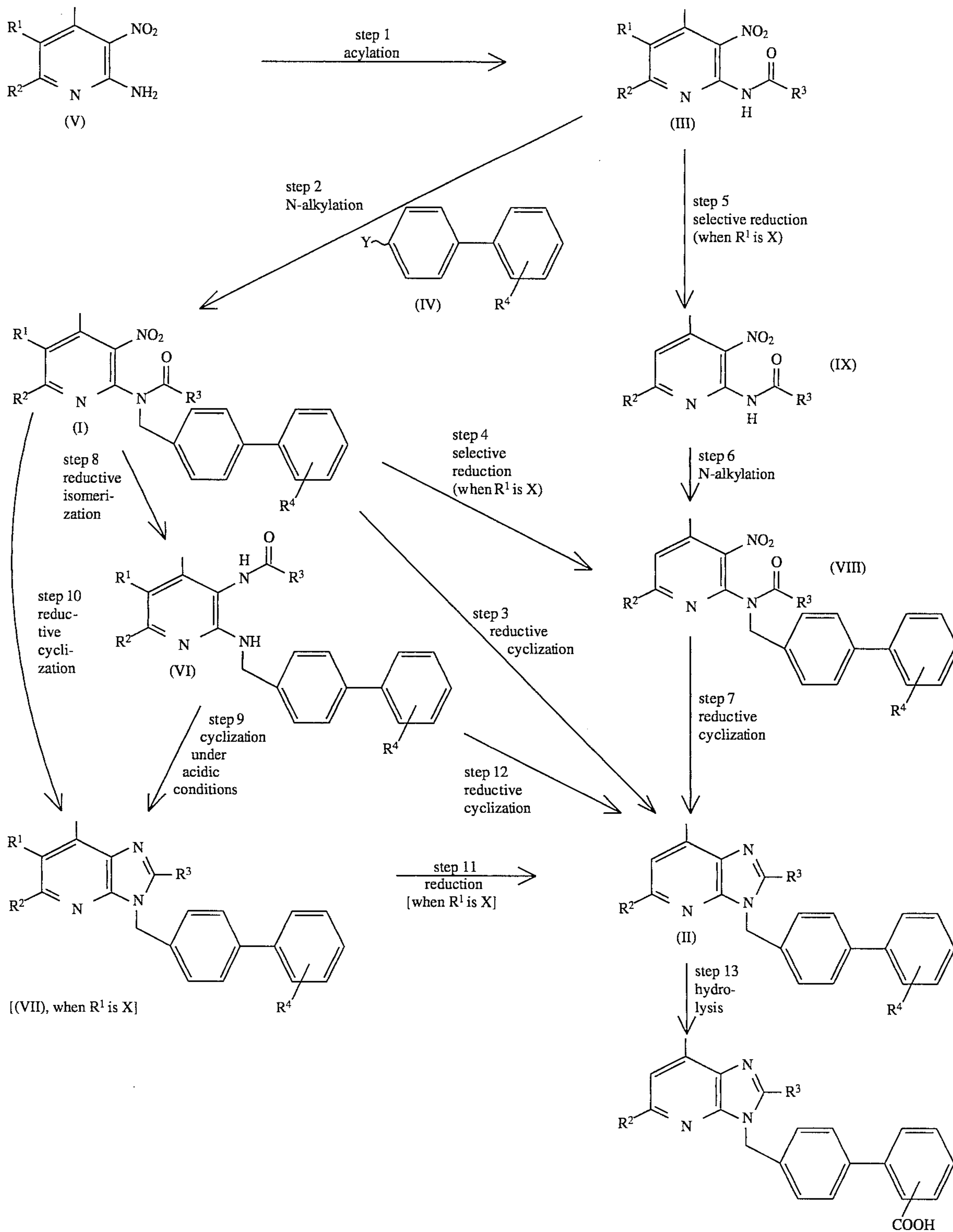
Reaction Scheme-4
