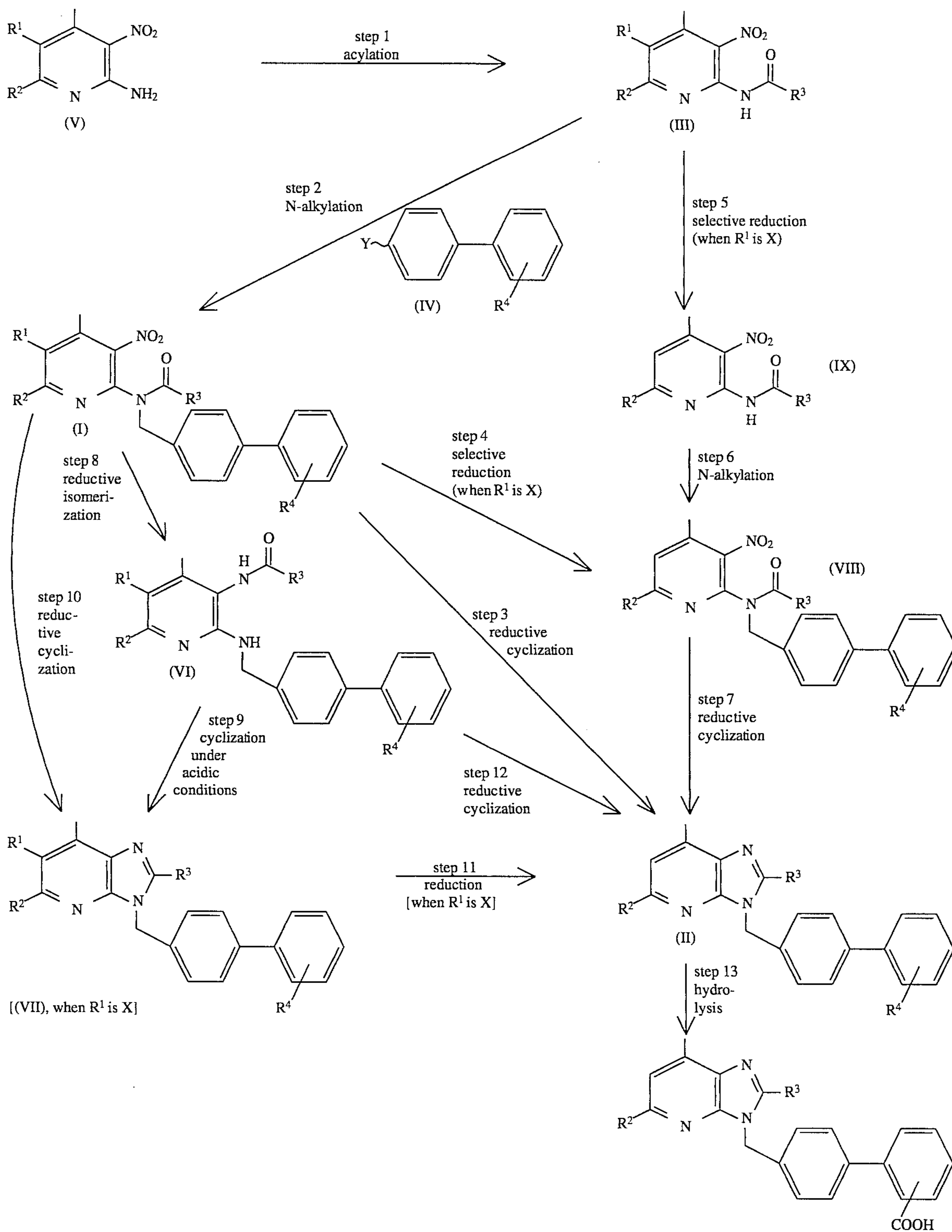
Reaction Scheme-4
