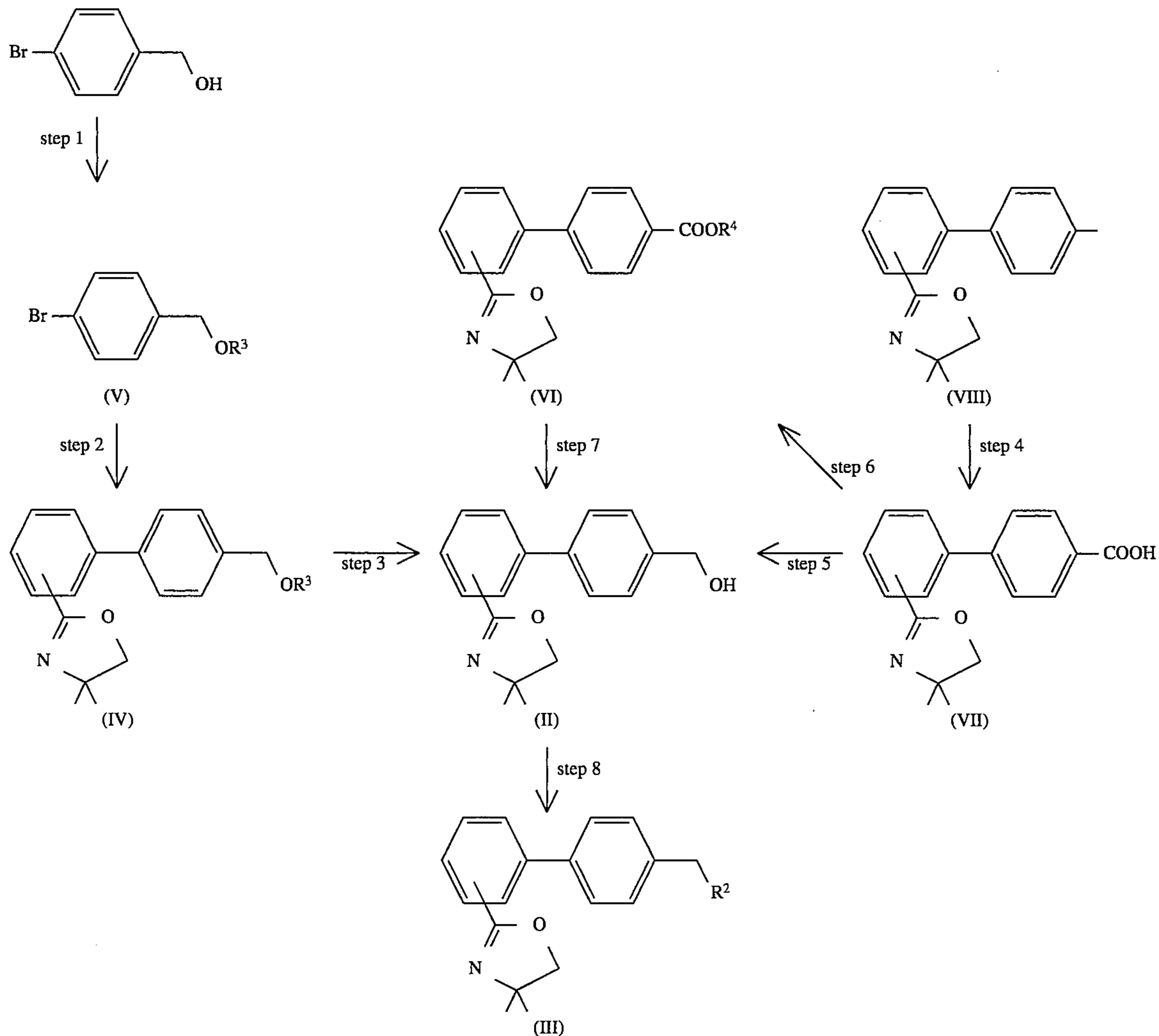
Reaction Scheme-6
