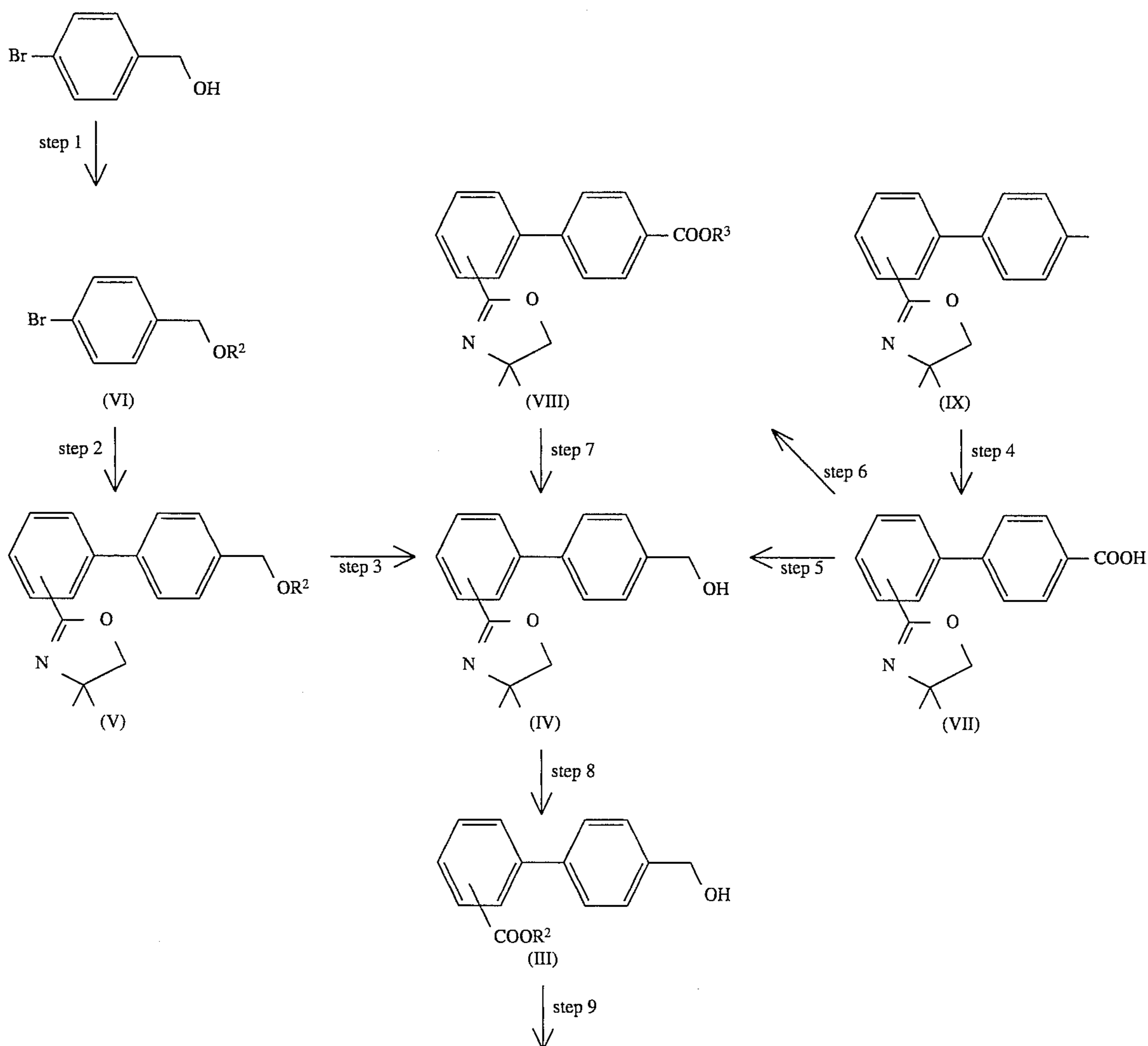
Reaction Scheme-7
