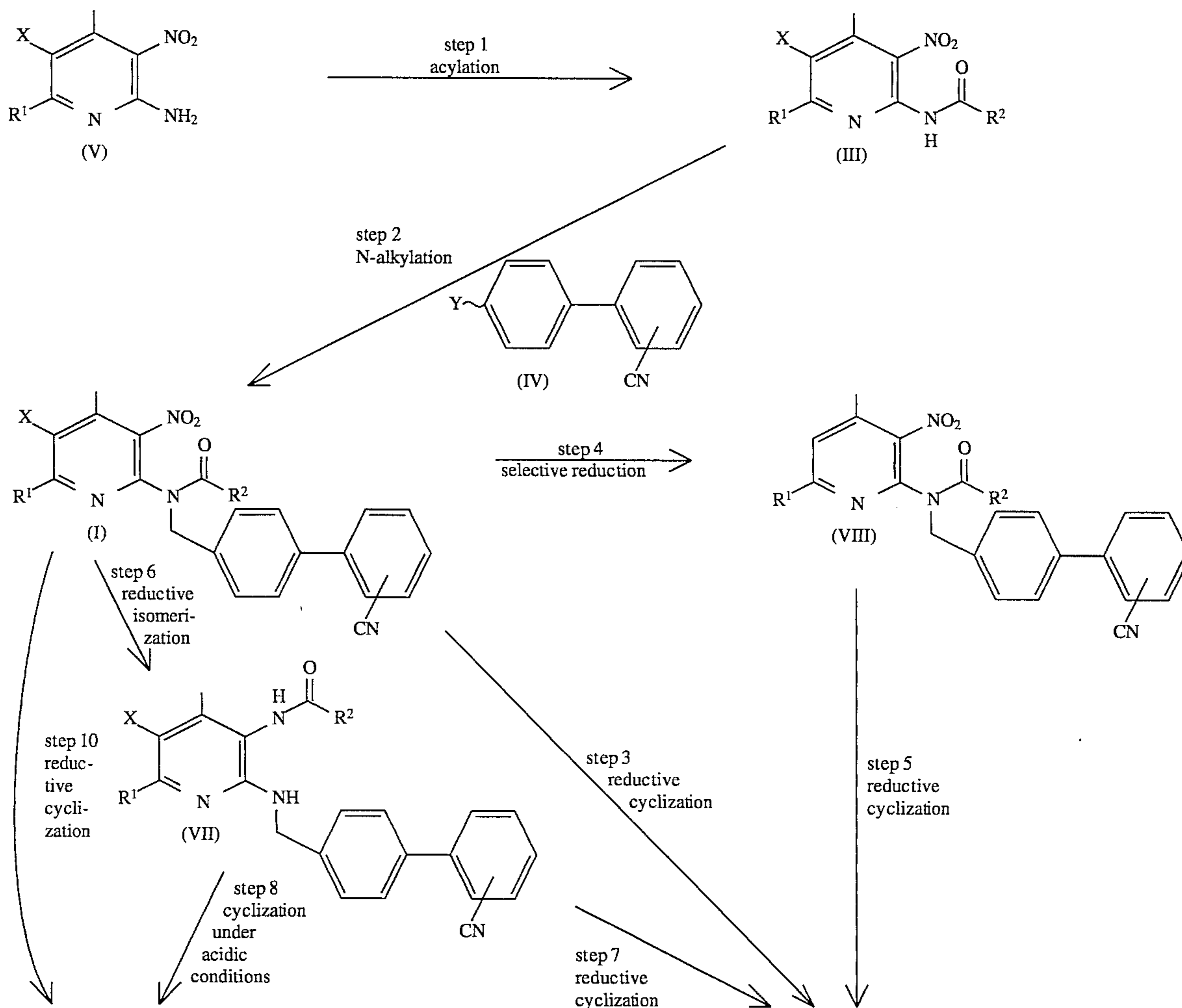
Reaction Scheme-5
