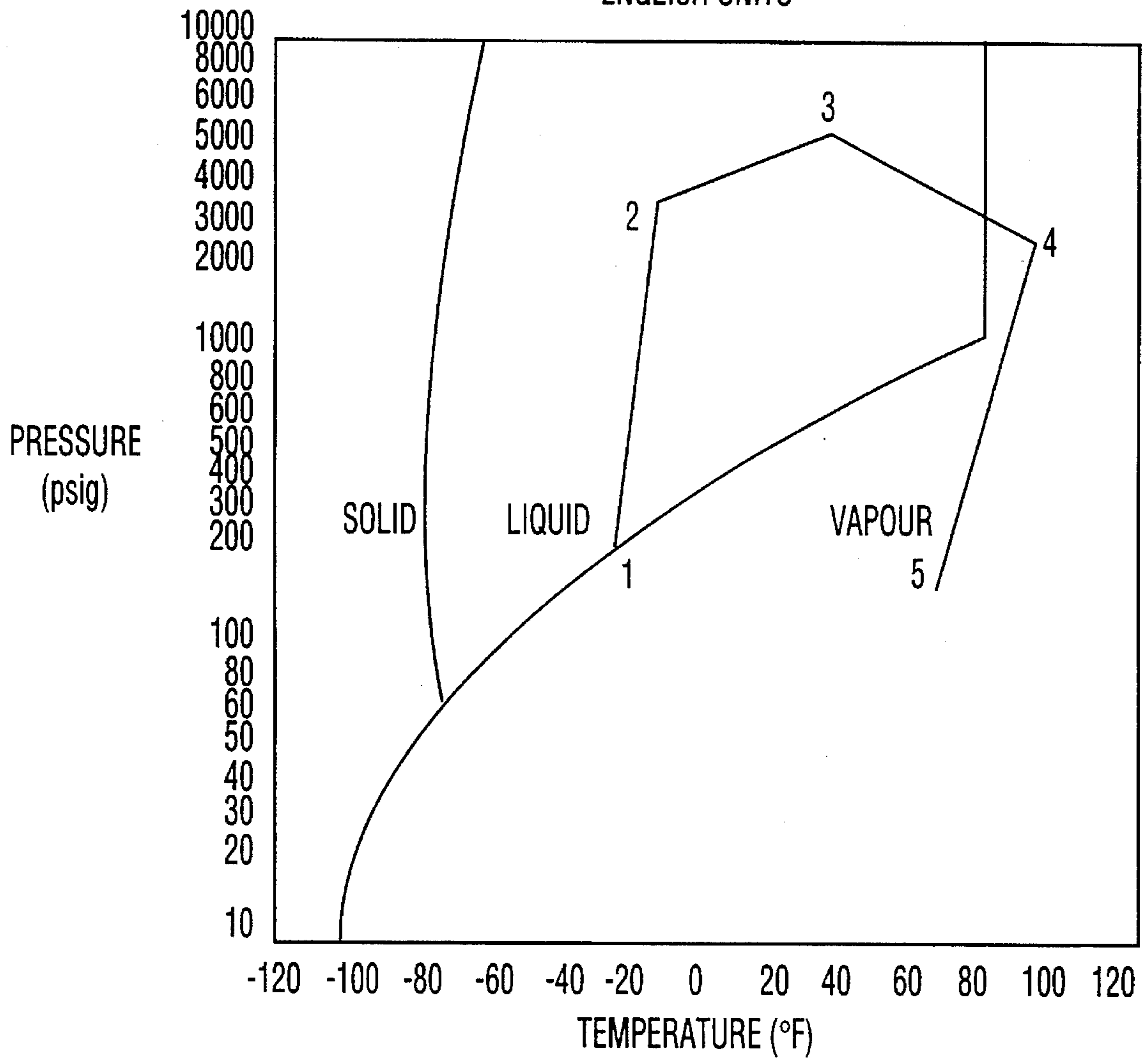
FIG. 2 (PRIOR ART)
