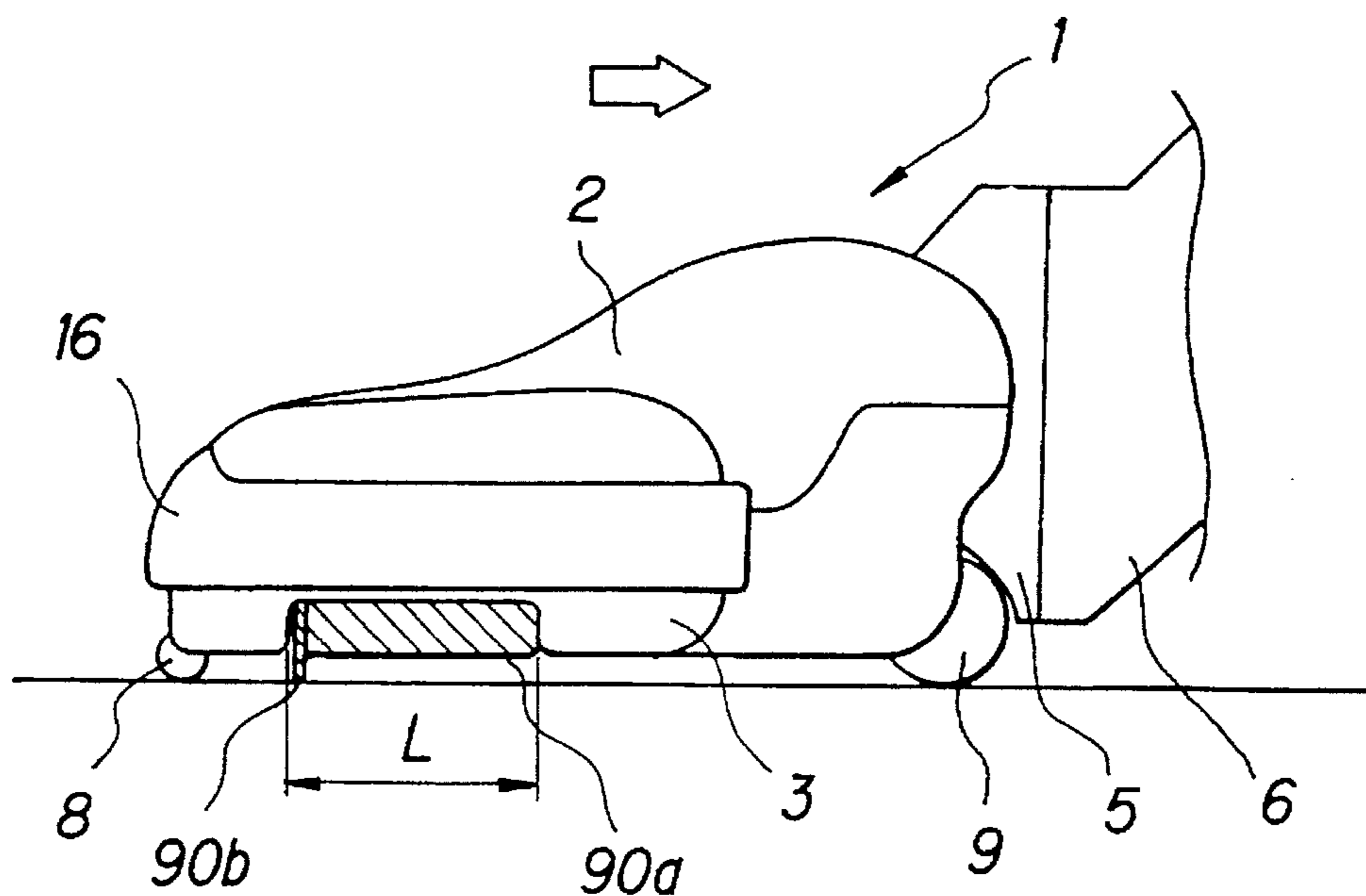
Nozzle Body Moving Backward
