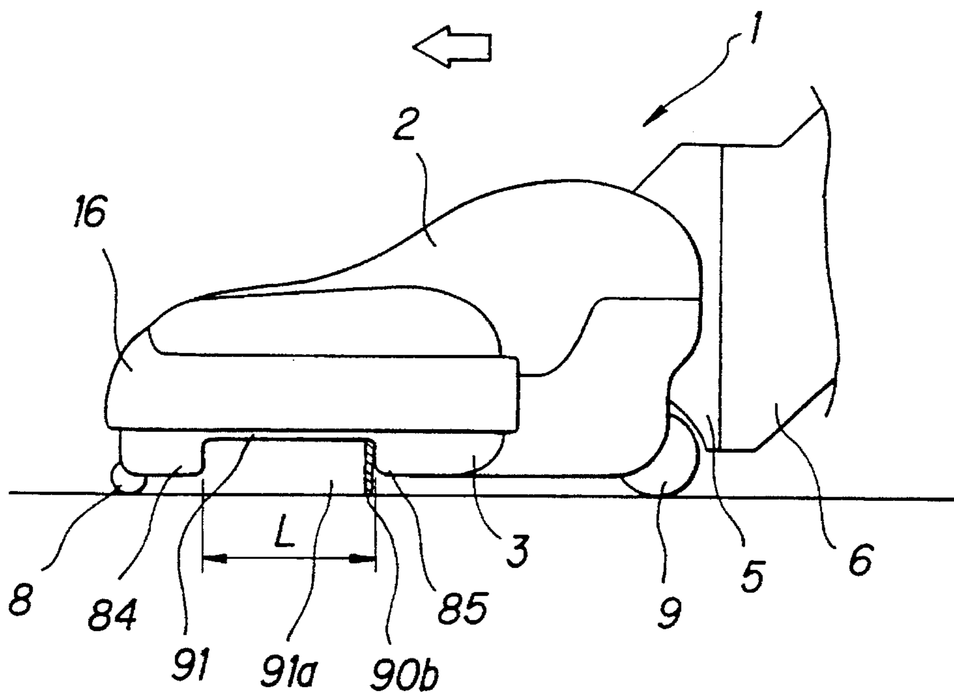
Nozzle Body Moving Forward
