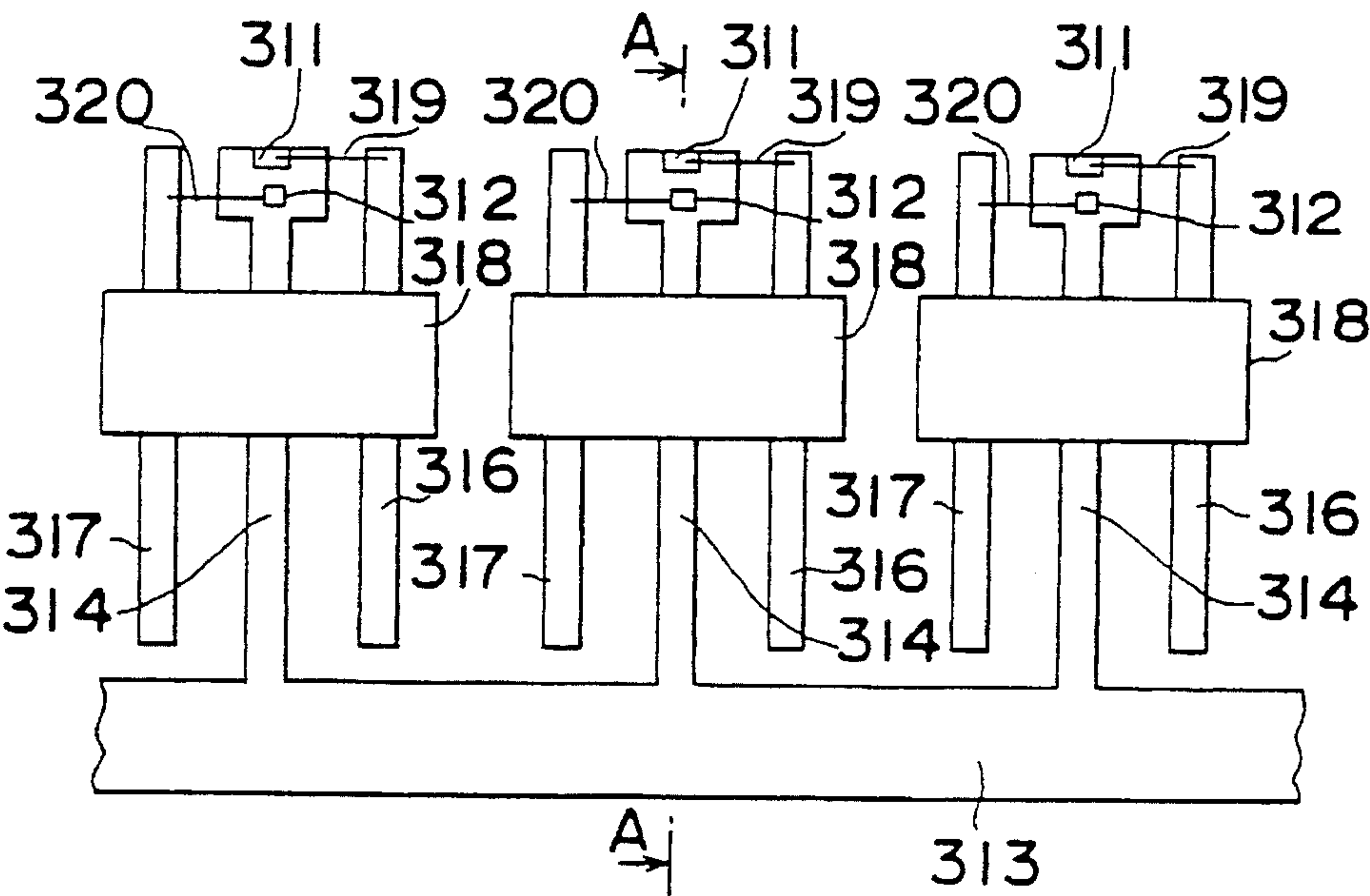
Fig. 49 Prior Art
