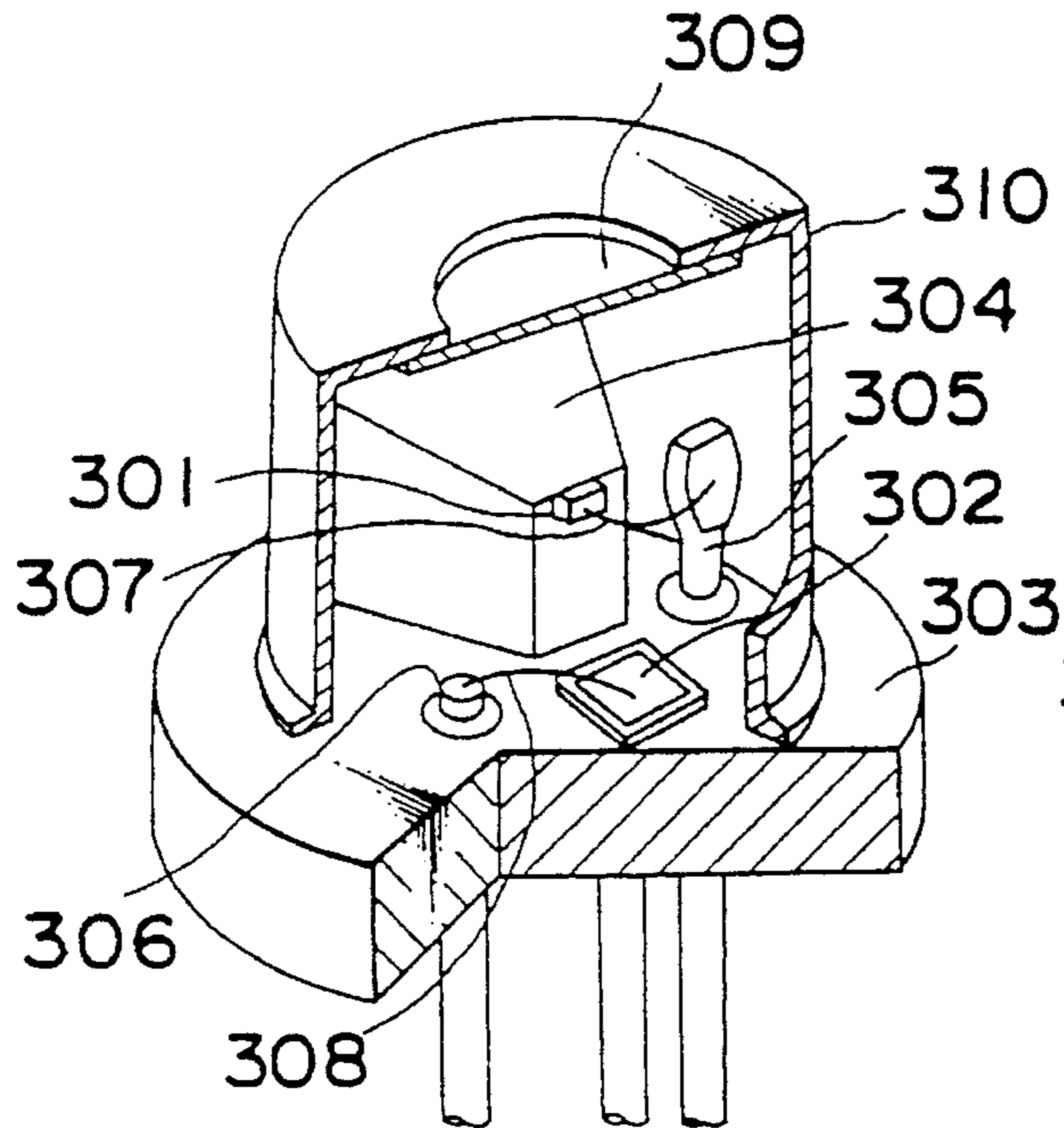
Fig. 47 Prior Art
