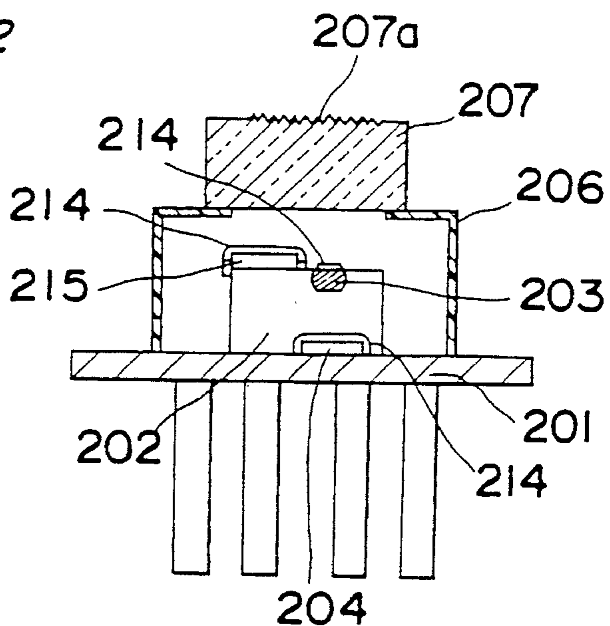
Fig. 43 Prior Art
