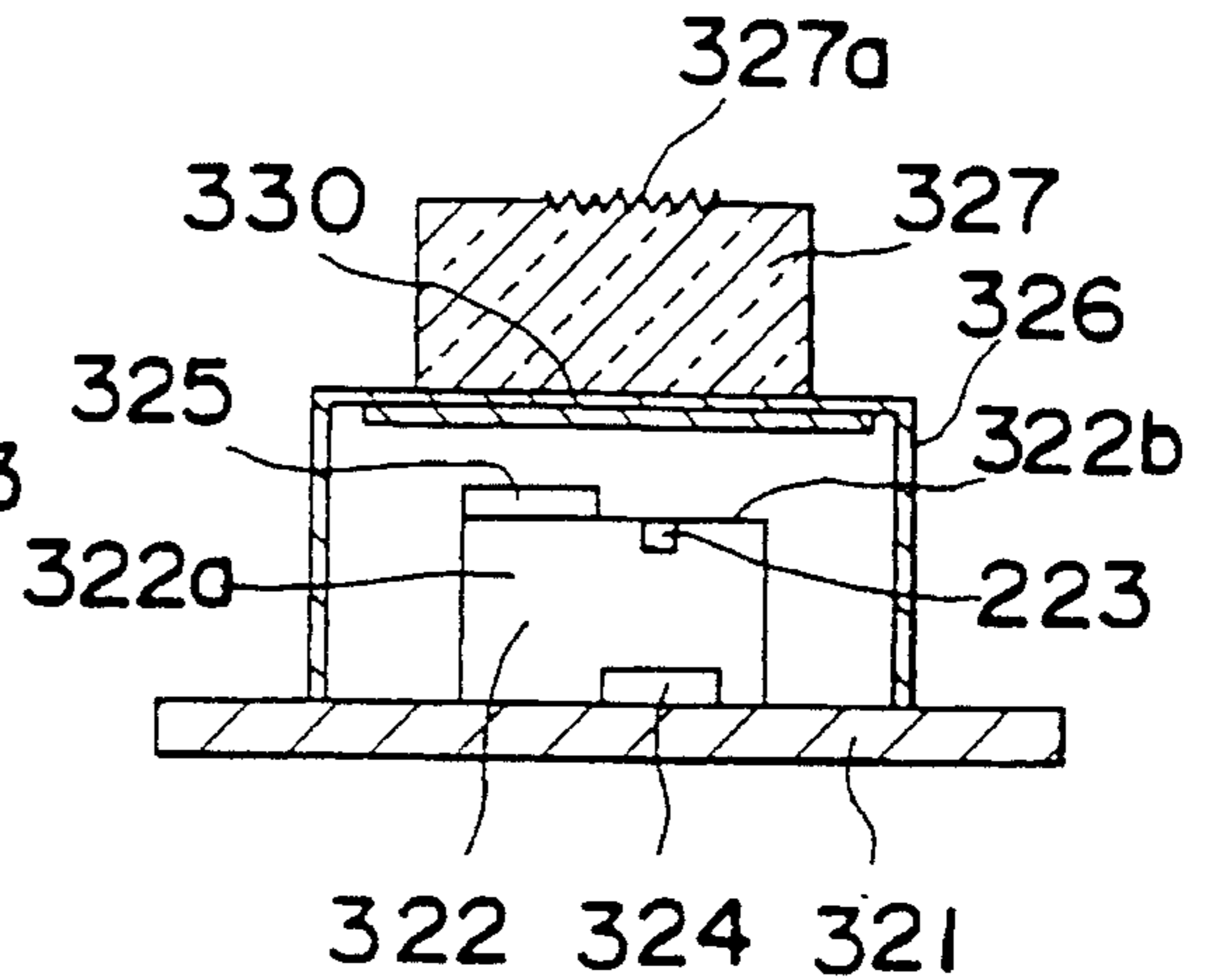
Fig. 50 Prior Art
