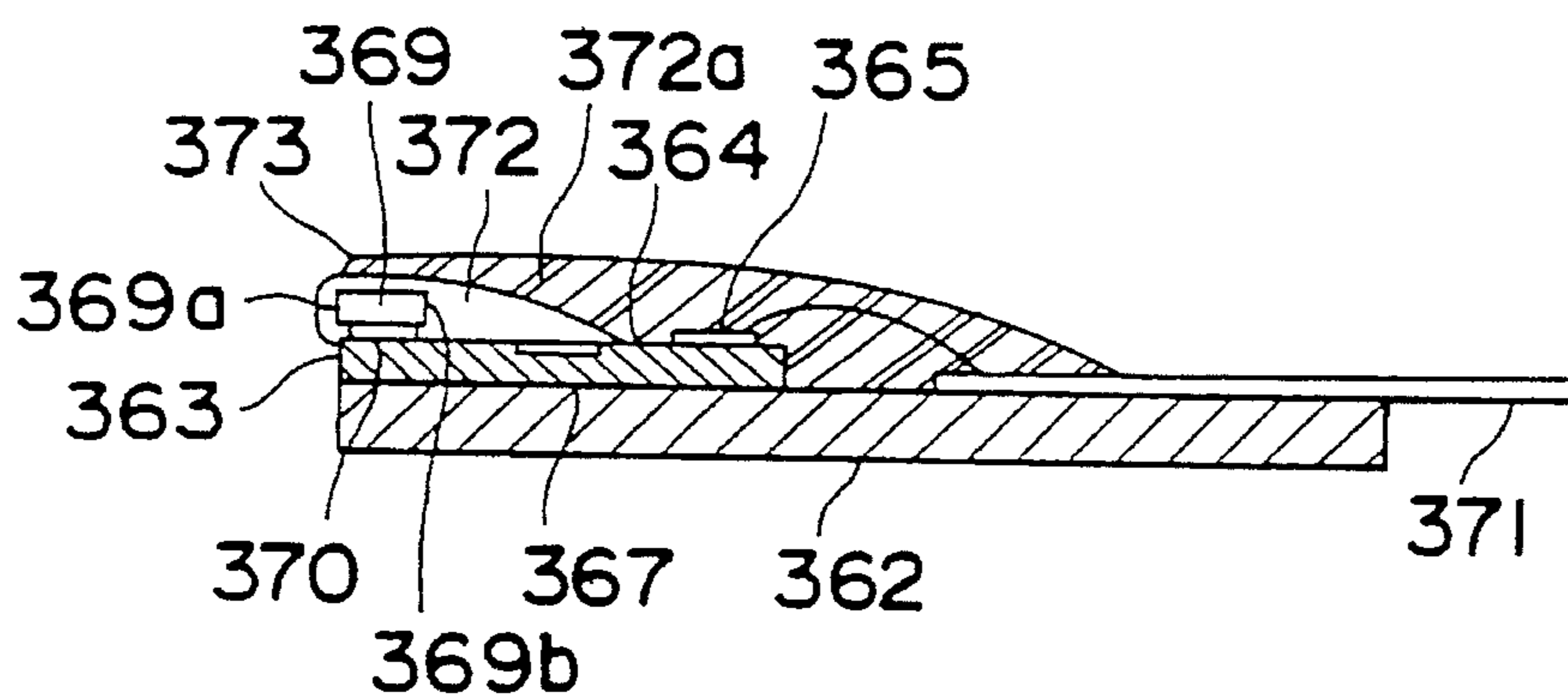
Fig. 43 Prior Art
