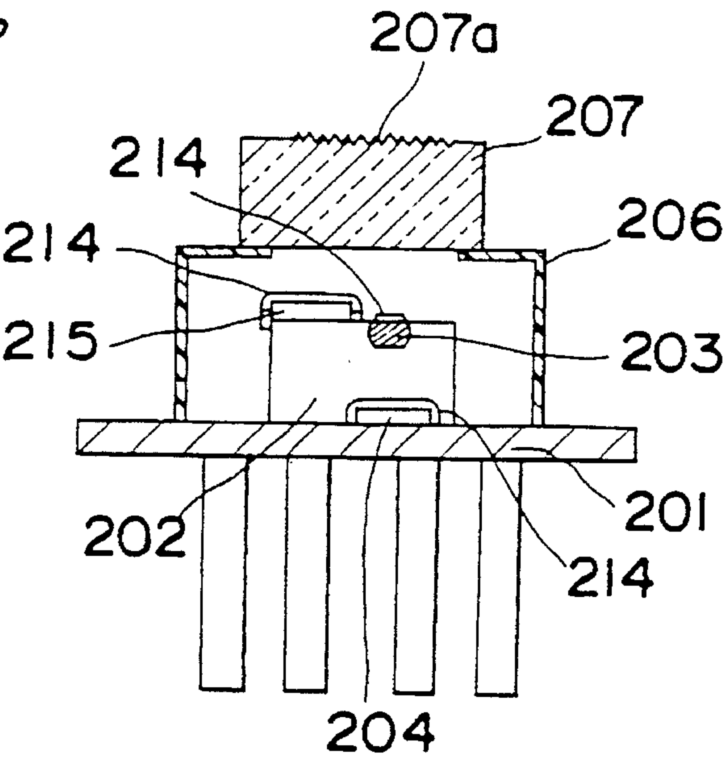
Fig. 43 Prior Art
