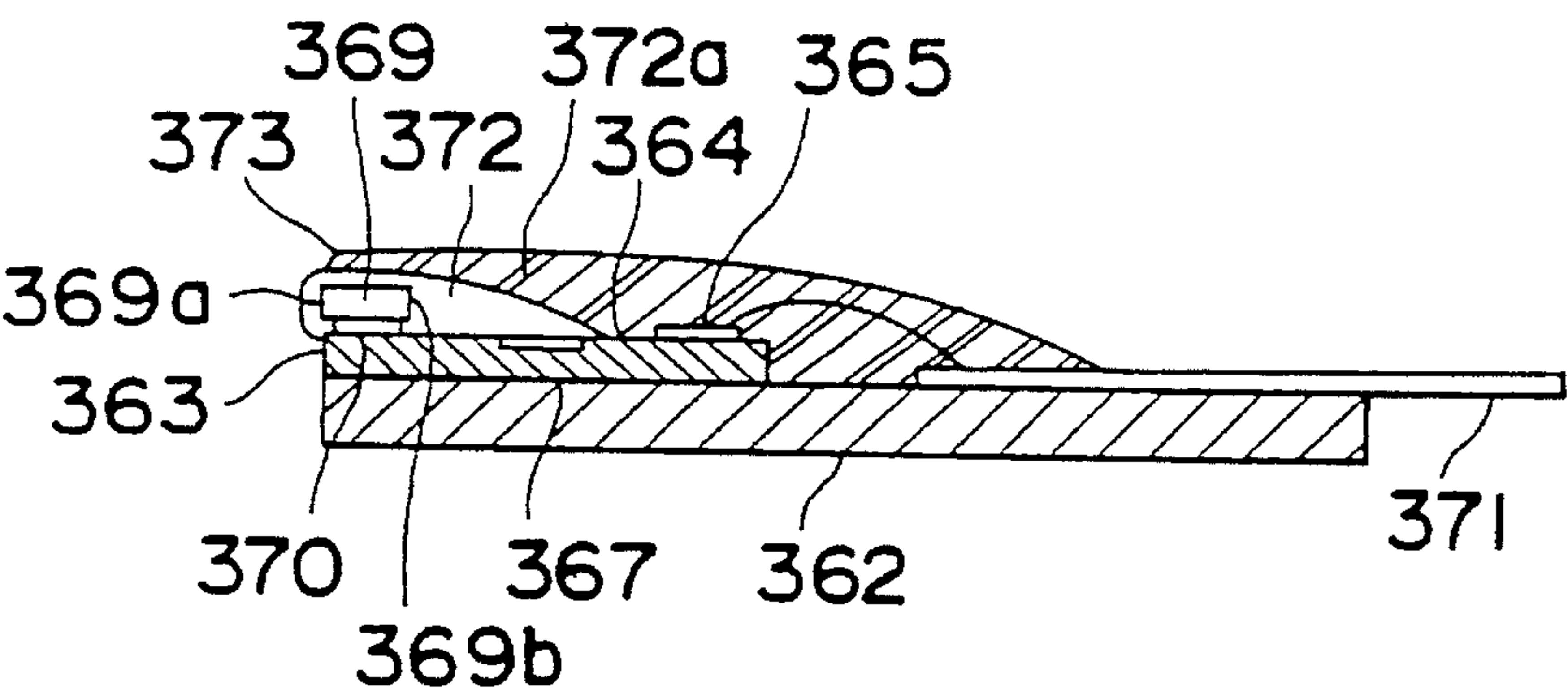
Fig. 43 Prior Art
