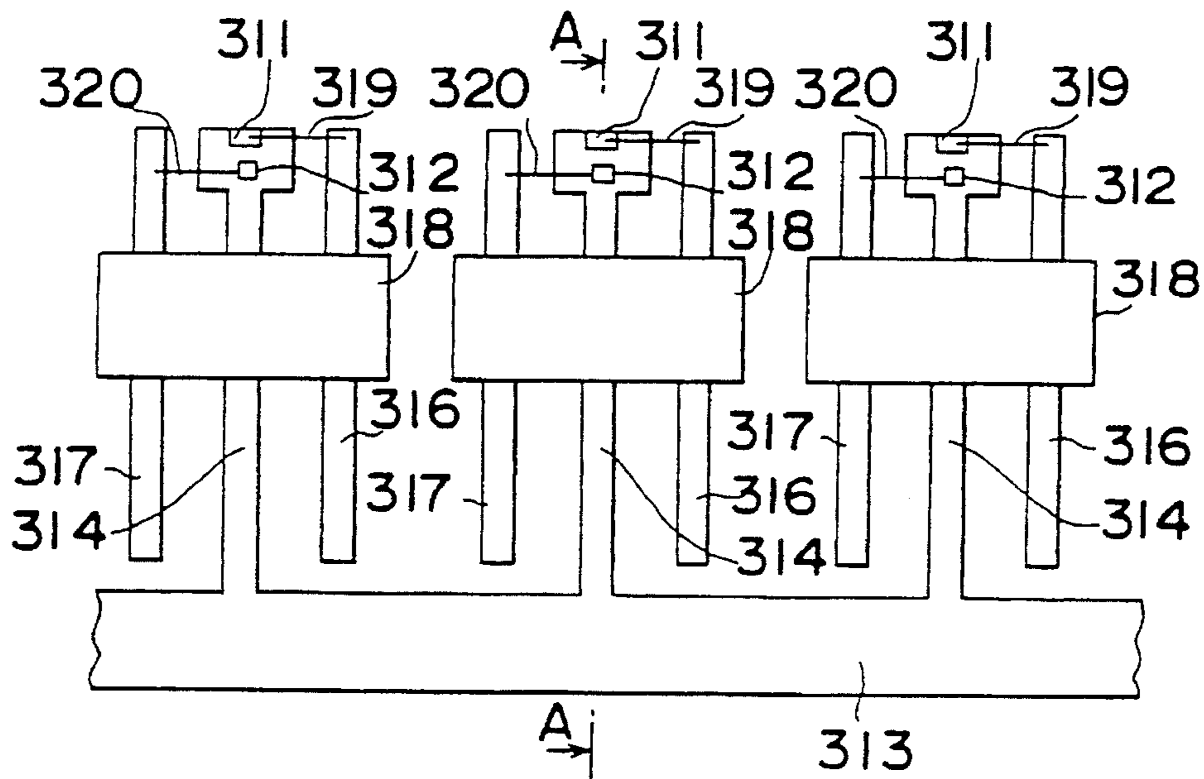
Fig. 49 Prior Art
