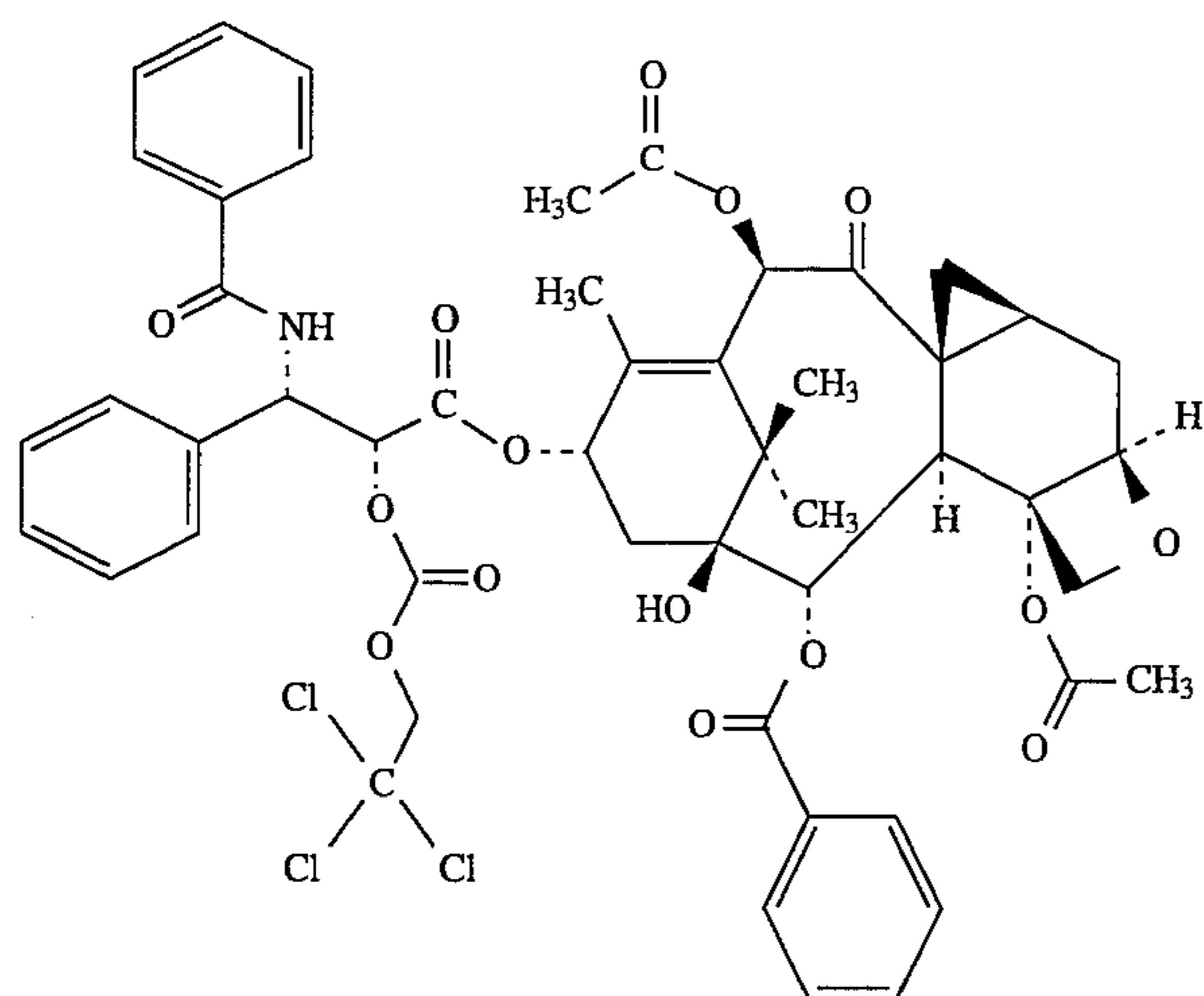
Compound IIa
