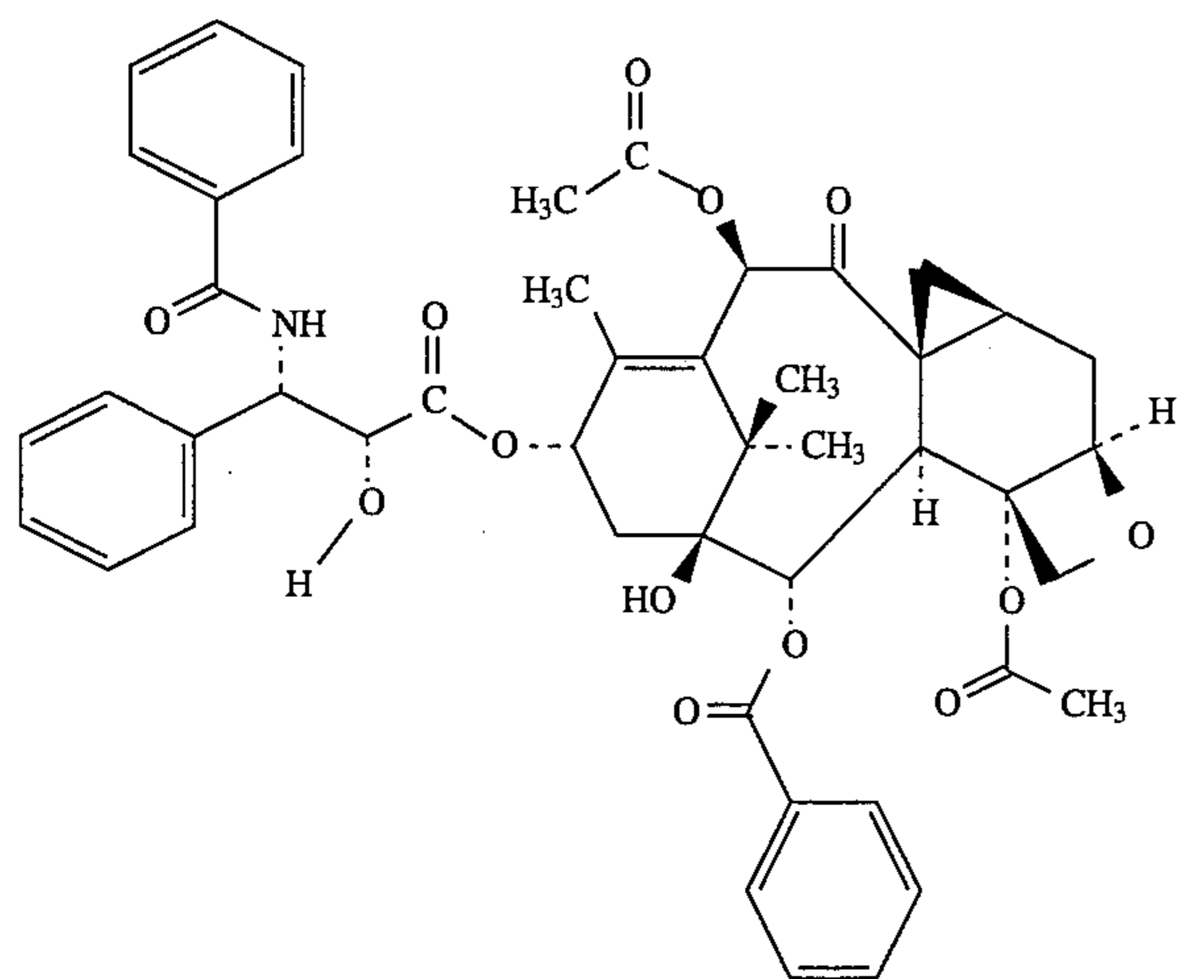
Compound IIb
