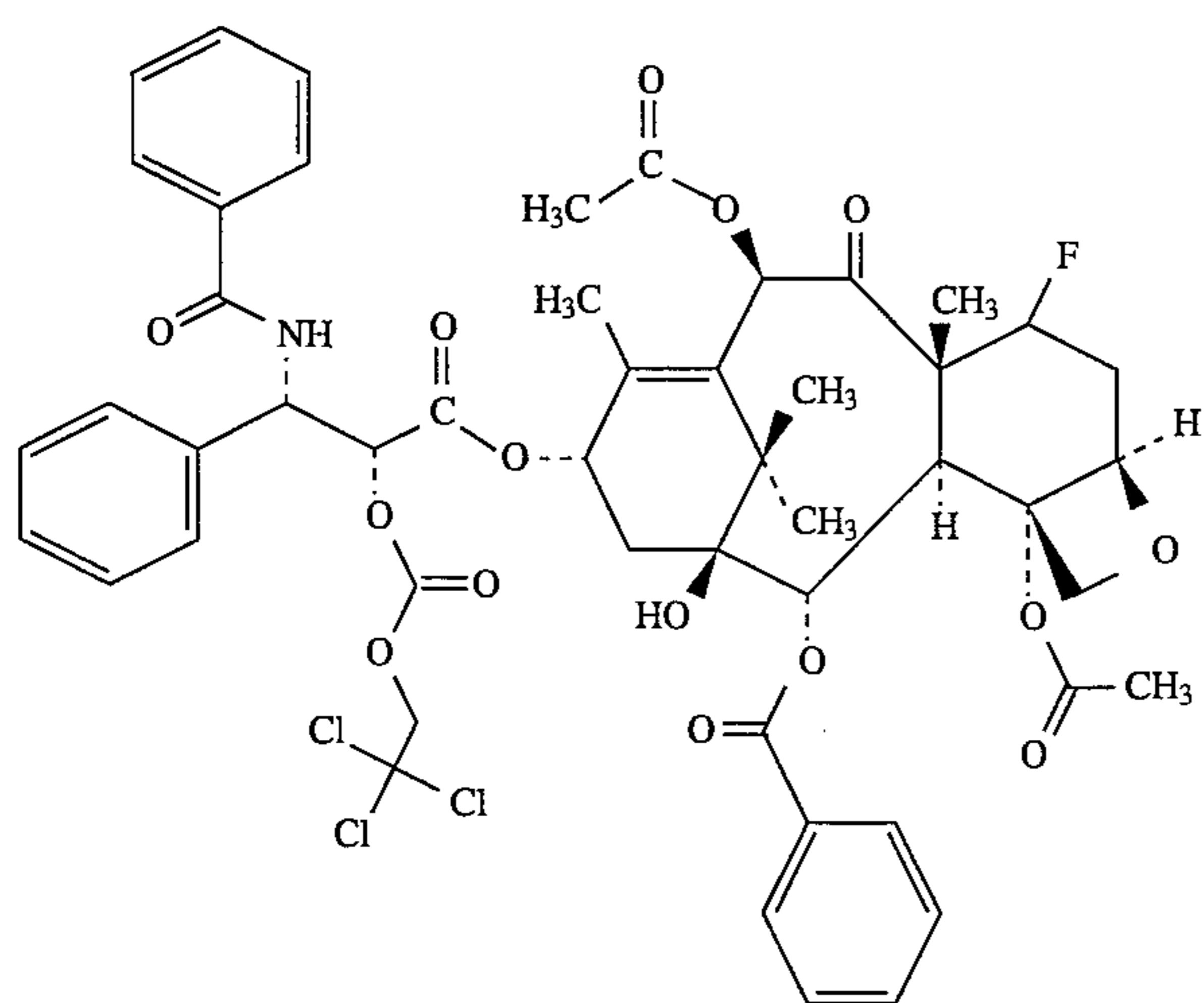
Compound IIIa
