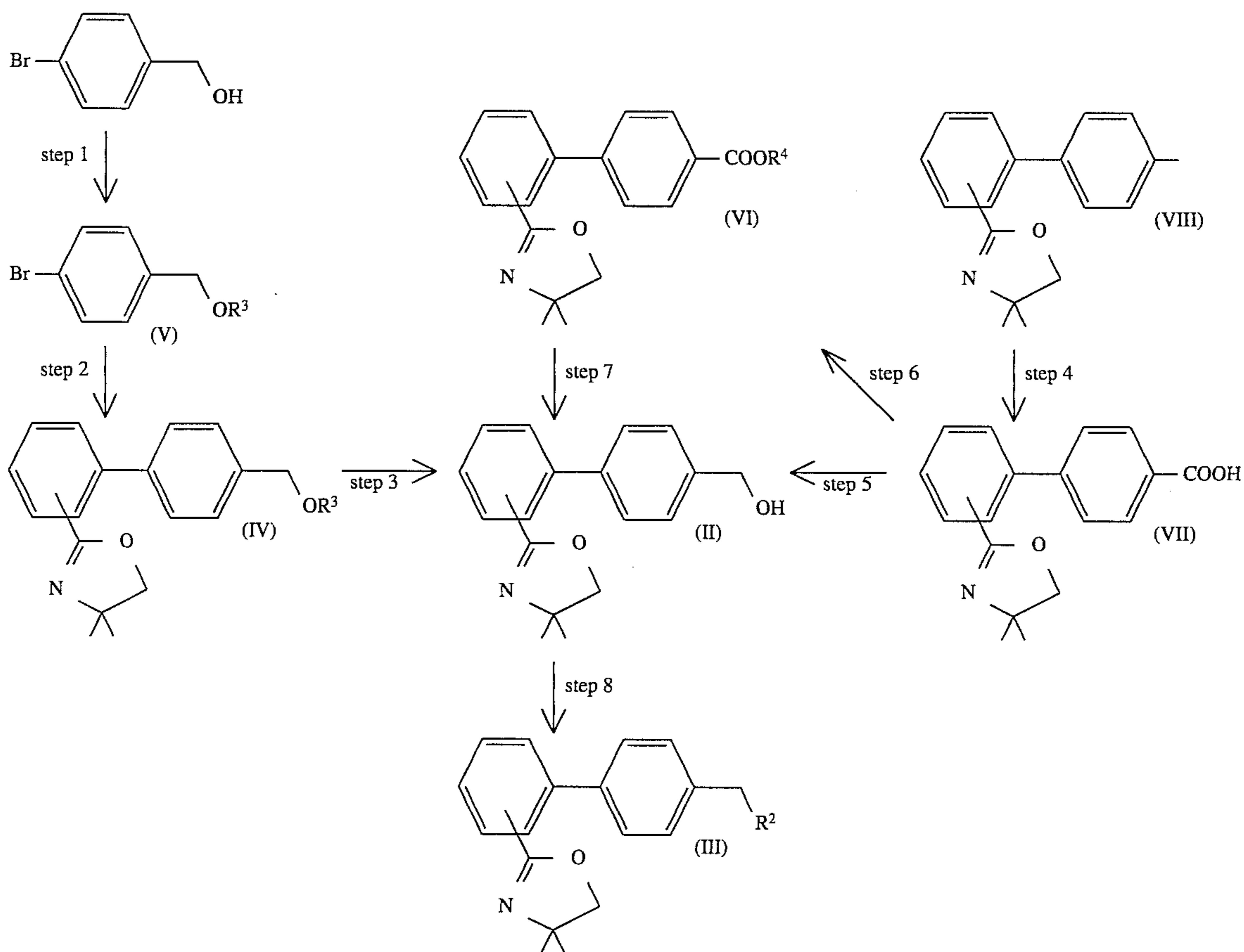
Reaction Scheme-6
