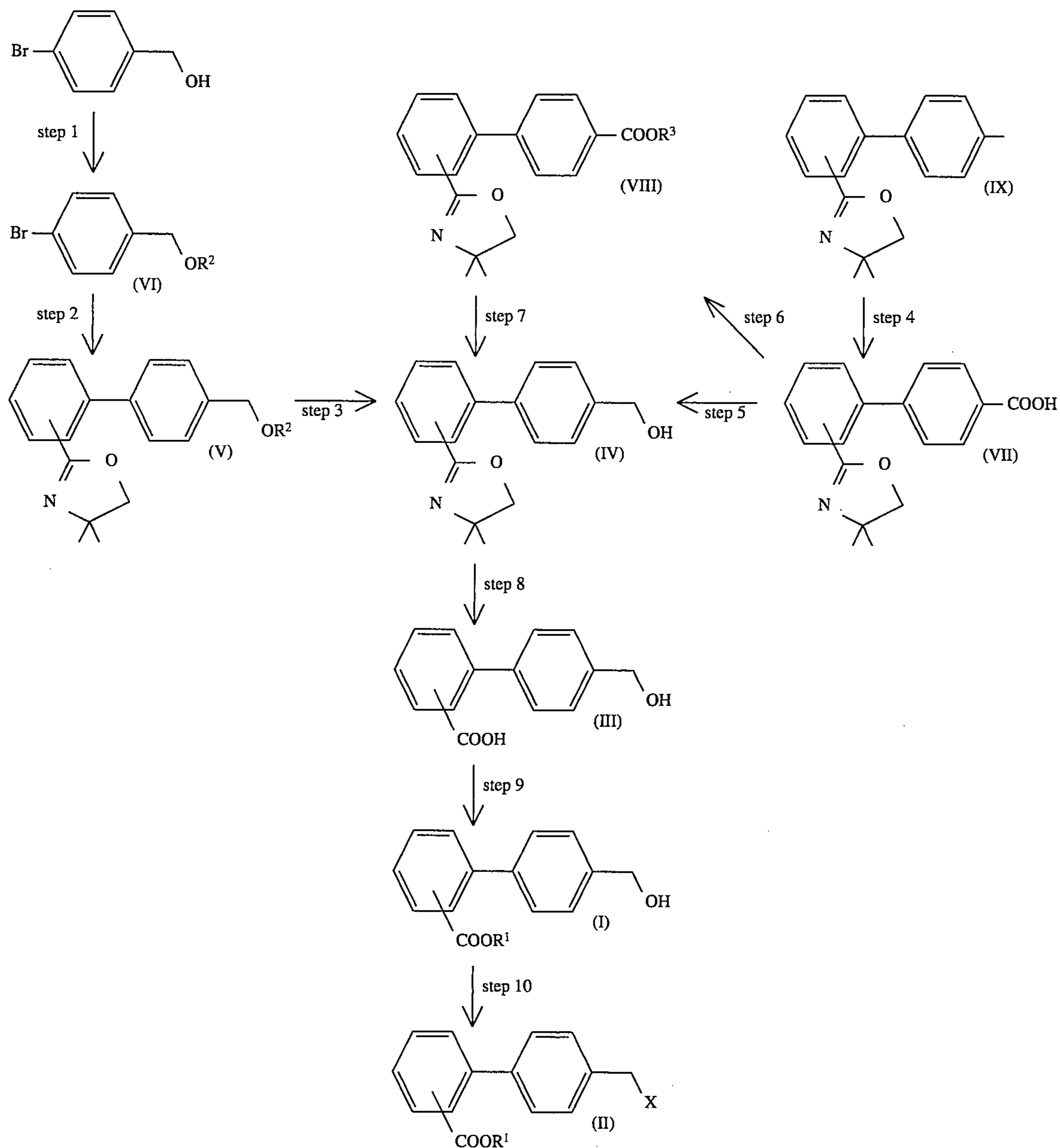
Reaction Scheme-8
