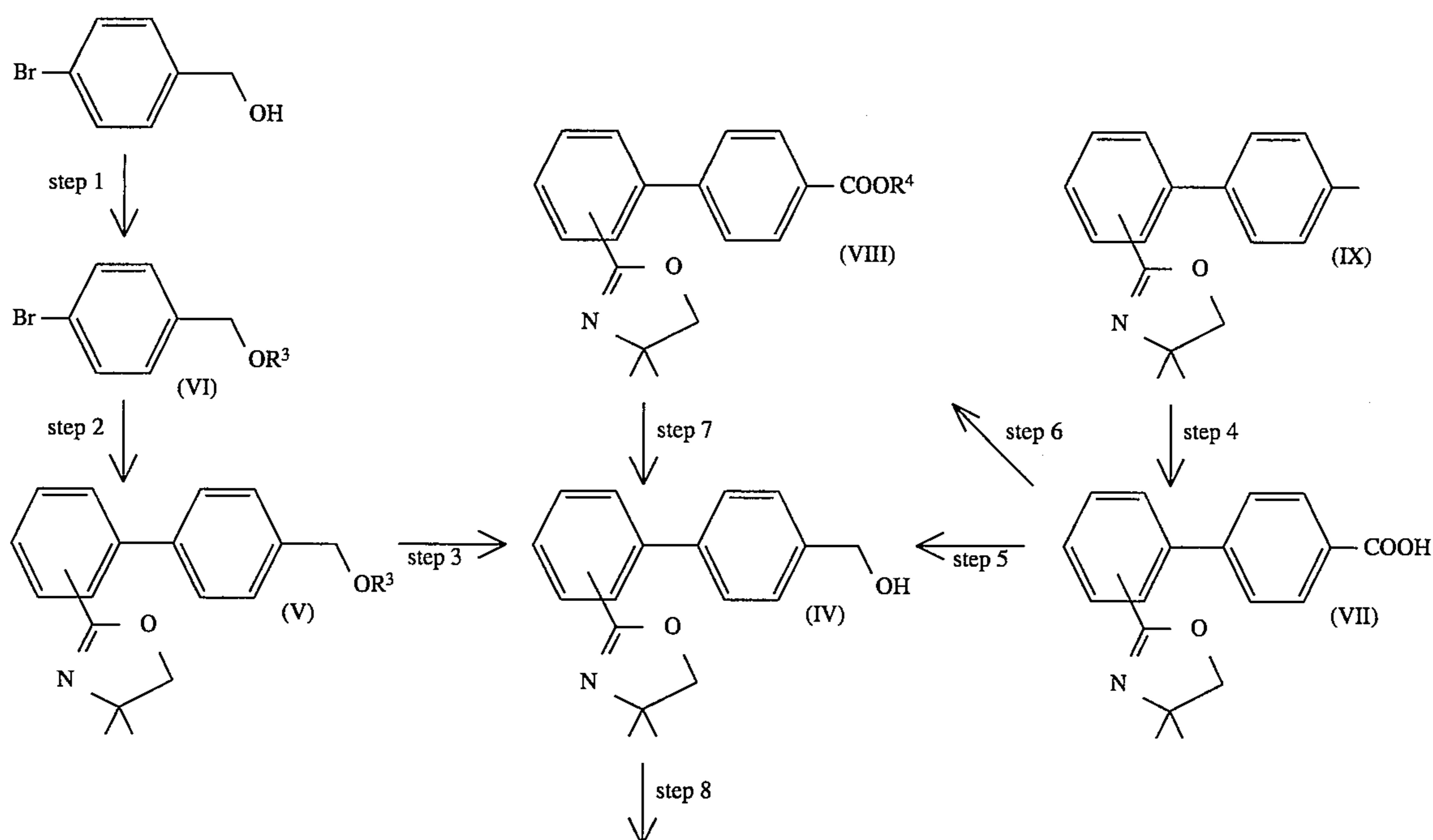
Reaction Scheme-7
