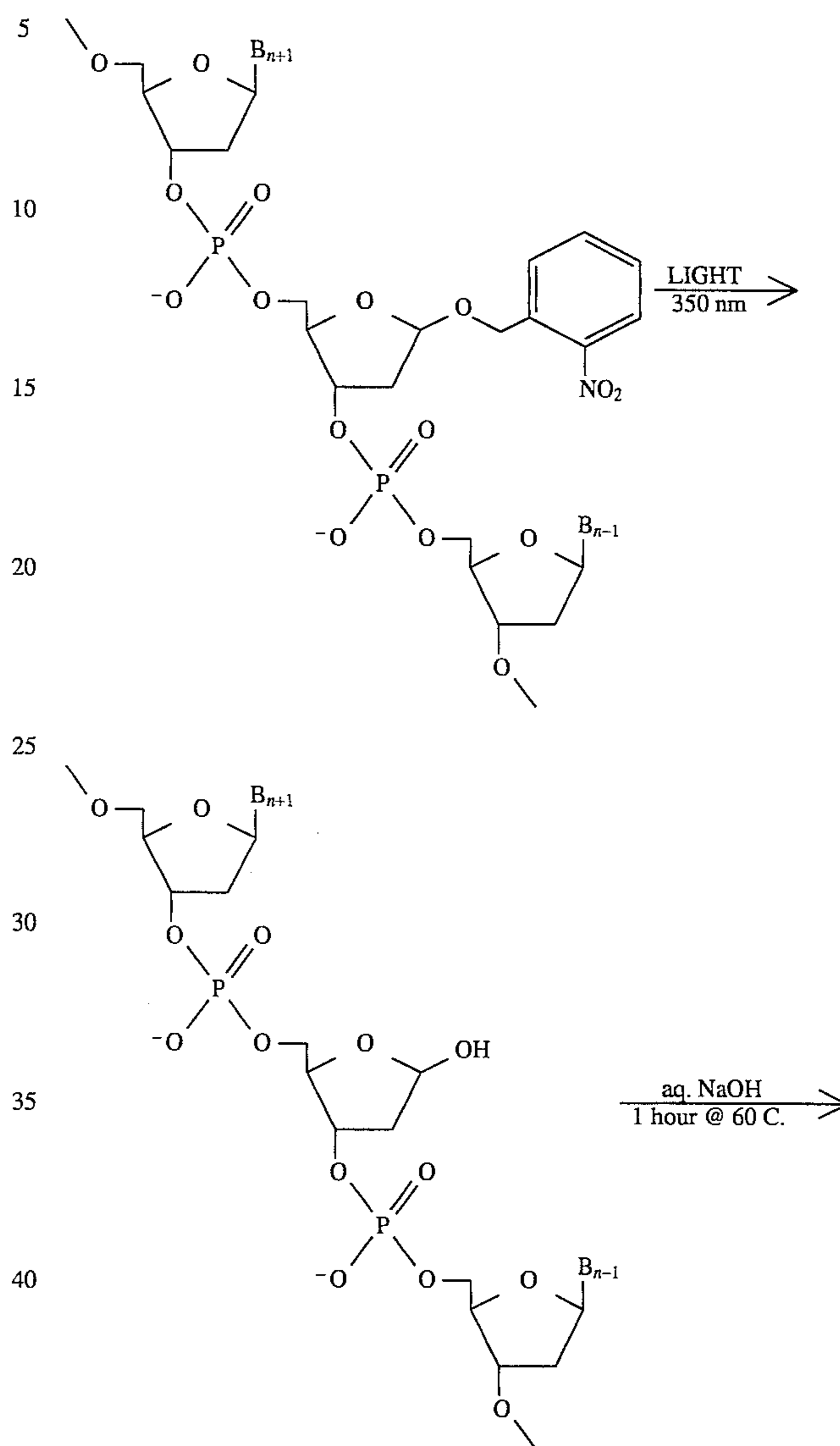
Scheme 6 CLEAVAGE OF 2-NITROBENZYL 2'-DEOXYRIBOSIDE LINKED DNA FRAGMENTS
