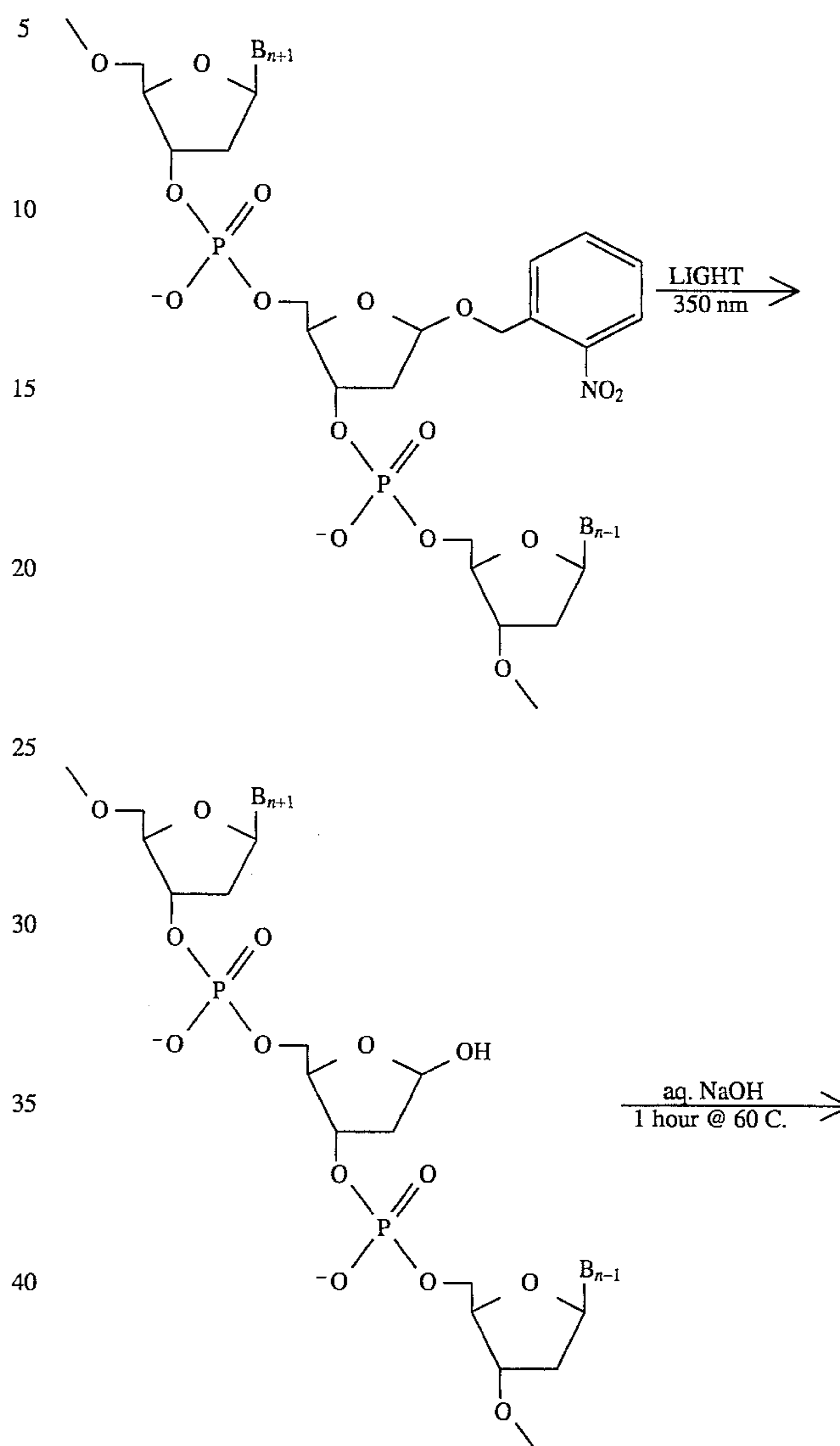
Scheme 6 CLEAVAGE OF 2-NITROBENZYL 2'-DEOXYRIBOSIDE LINKED DNA FRAGMENTS
