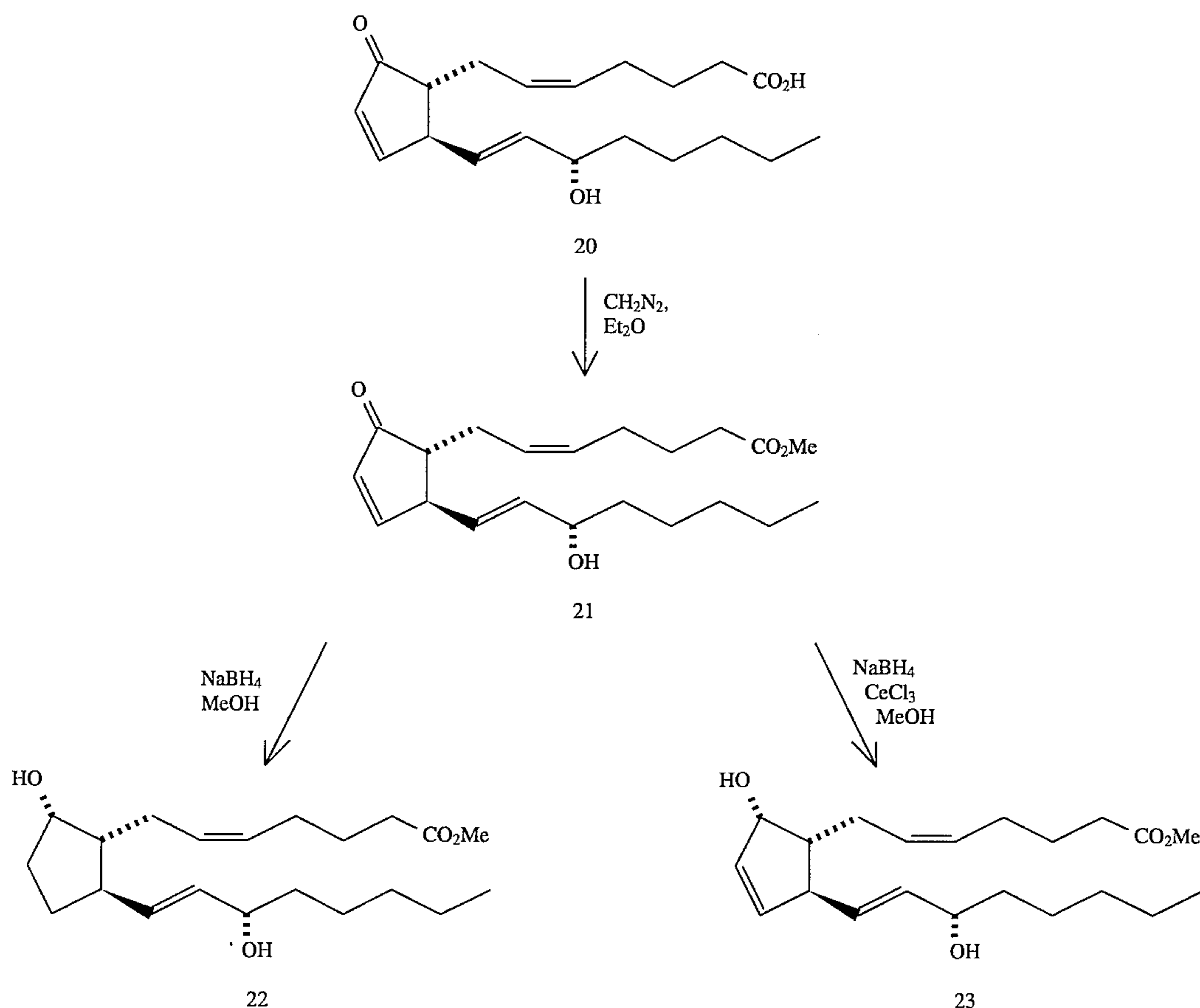
Reaction Scheme 1
