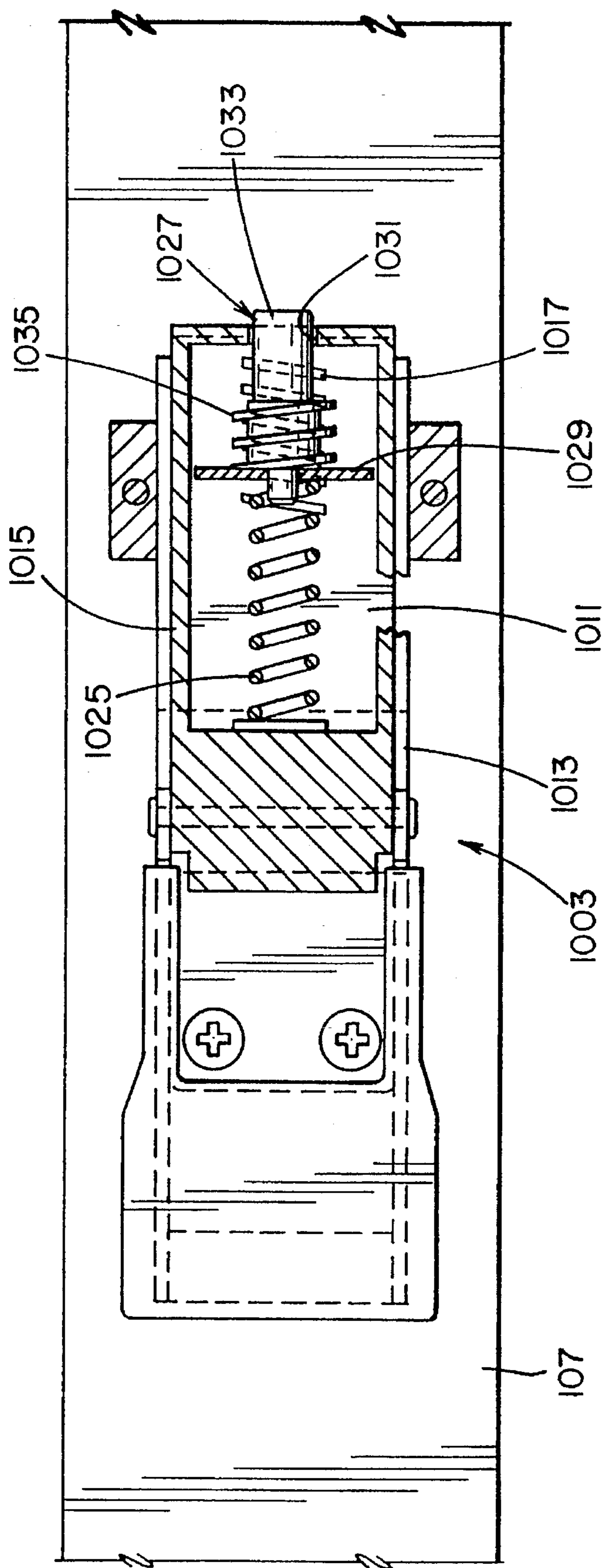
FIG. 29 (PRIOR ART)
