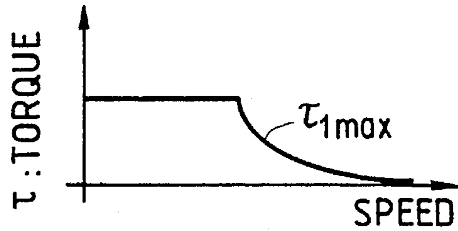
SPEED/TORQUE CHARACTERISTIC FOR LOW SPEED MOTOR
