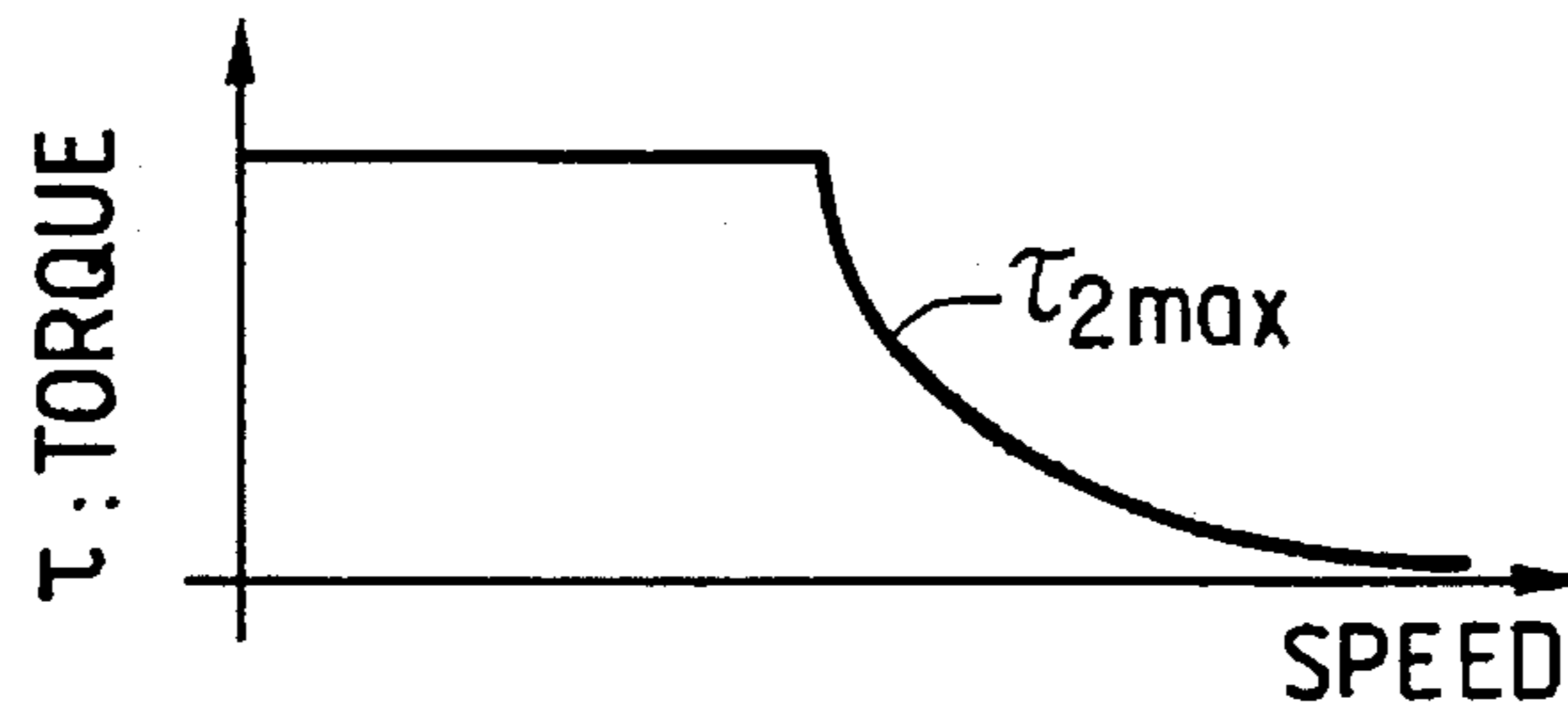
SPEED/TORQUE CHARACTERISTIC FOR HIGH SPEED MOTOR
