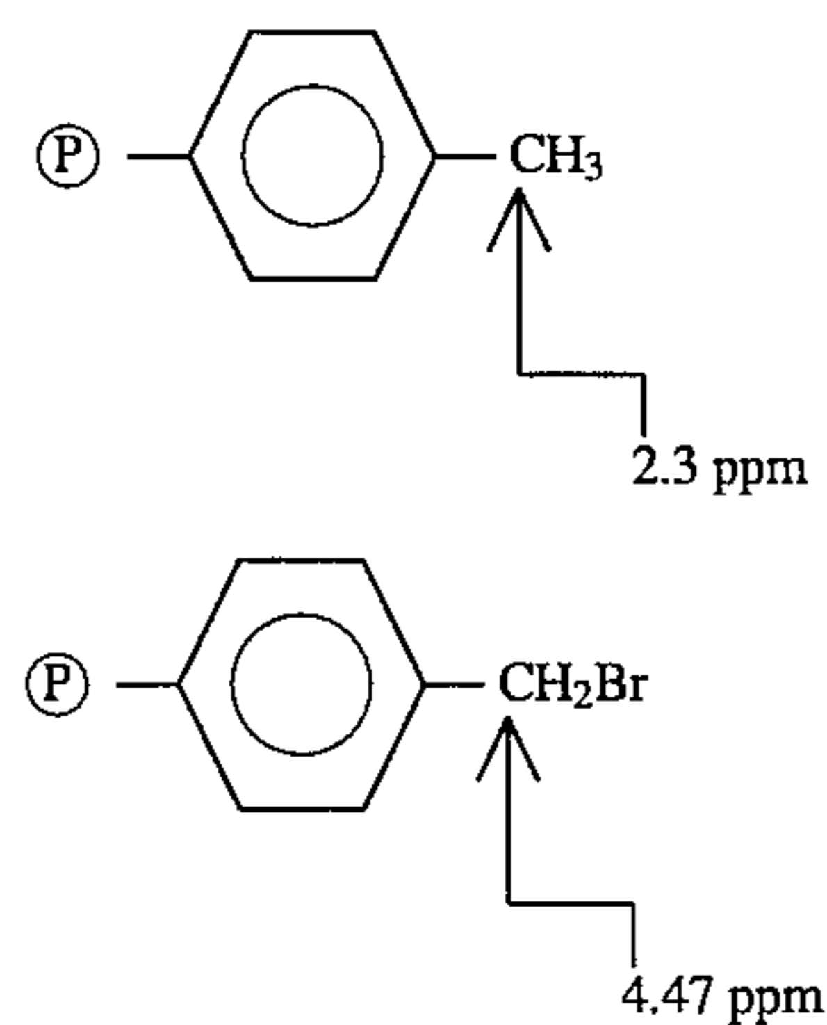
PROTON NMR RESONANCES FOR ENCHAINED "MER" UNITS
