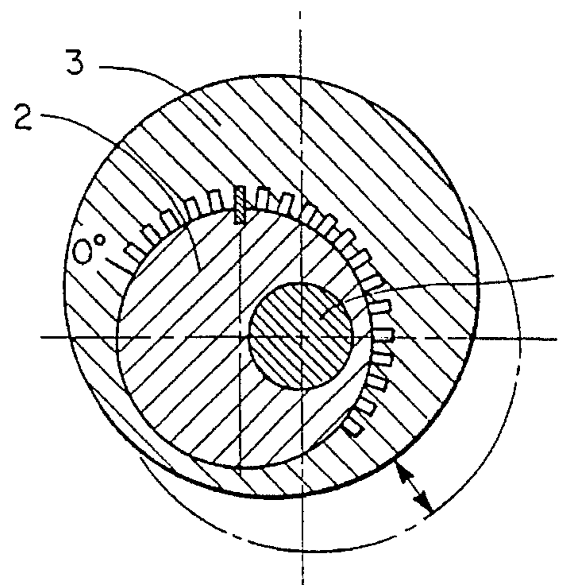
Fig. 29 INTERMEDIATE FIXED POSITION (WITH SPLINE KEY)
