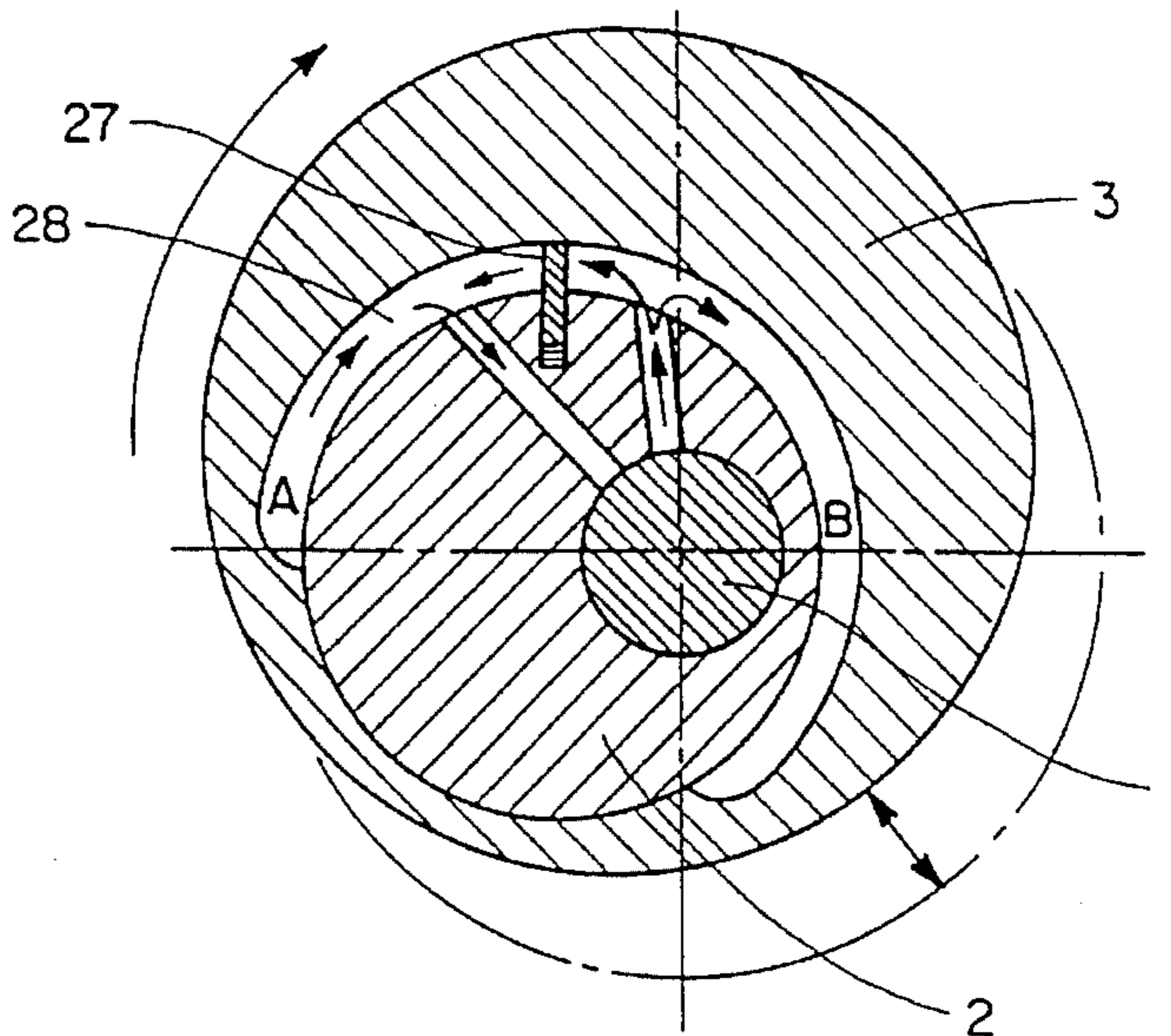
Fig. 17 INTERMEDIATE RETURN
