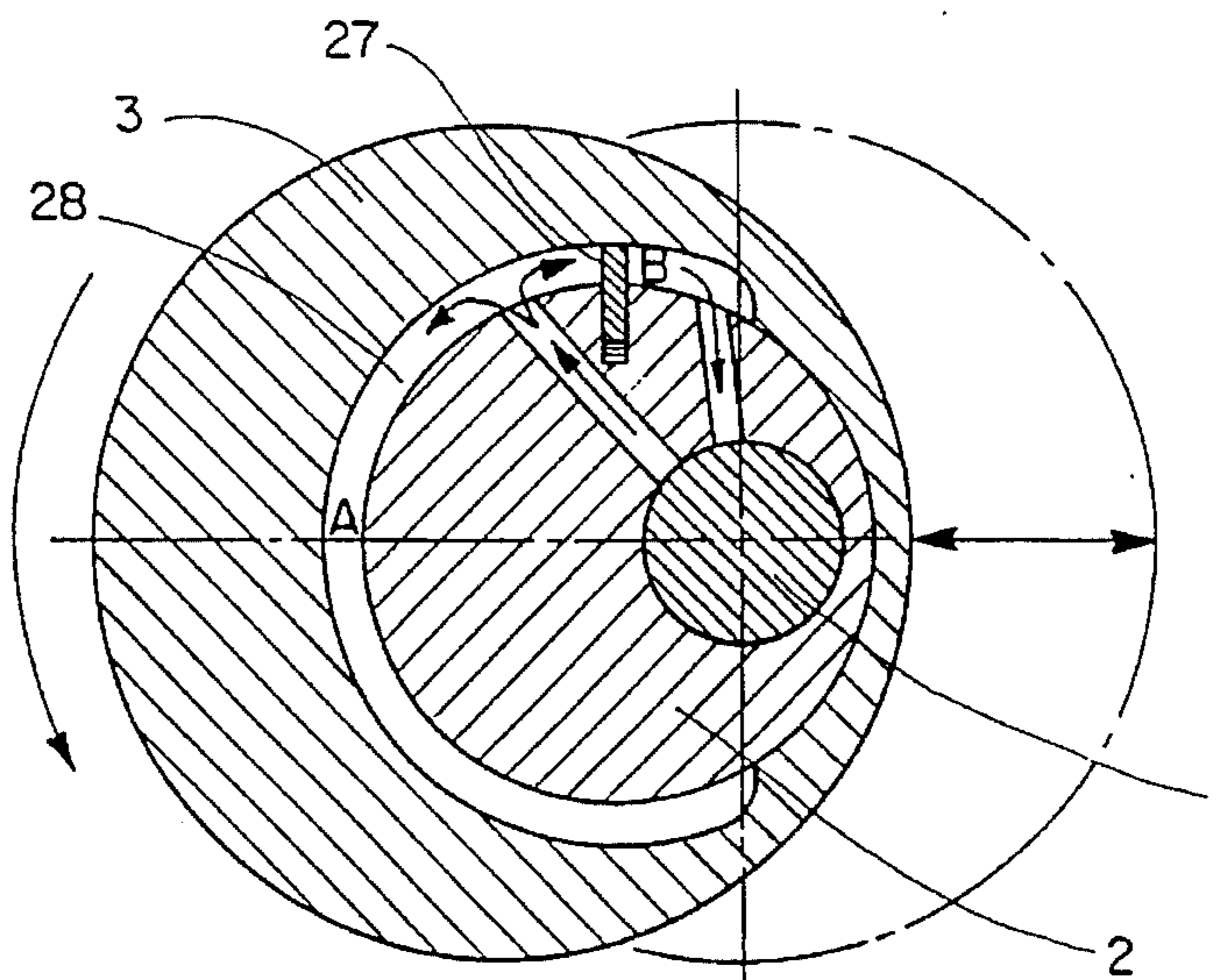
Fig. 16 MAX. OFFSET
