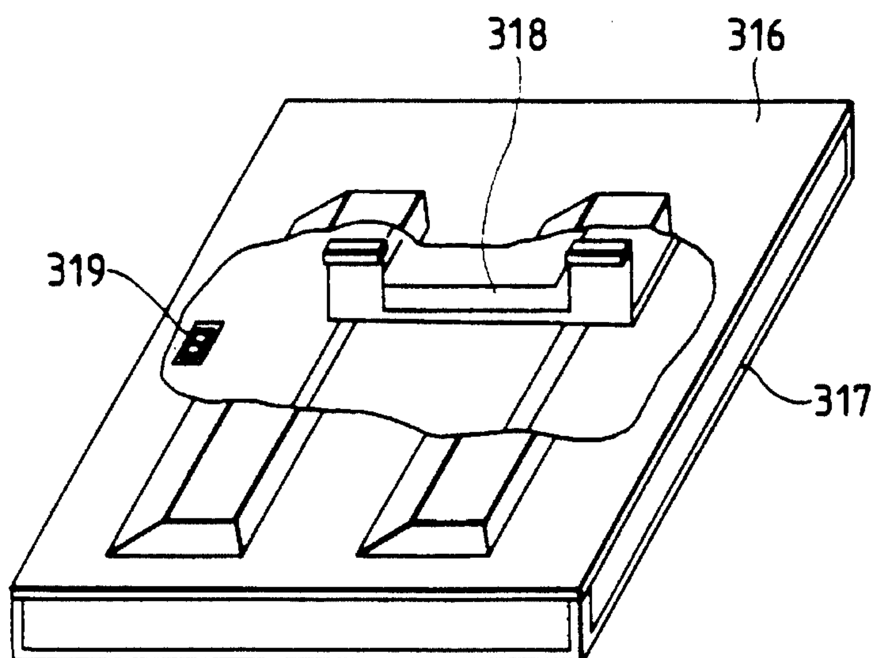
FIG. 15 PRIOR ART
