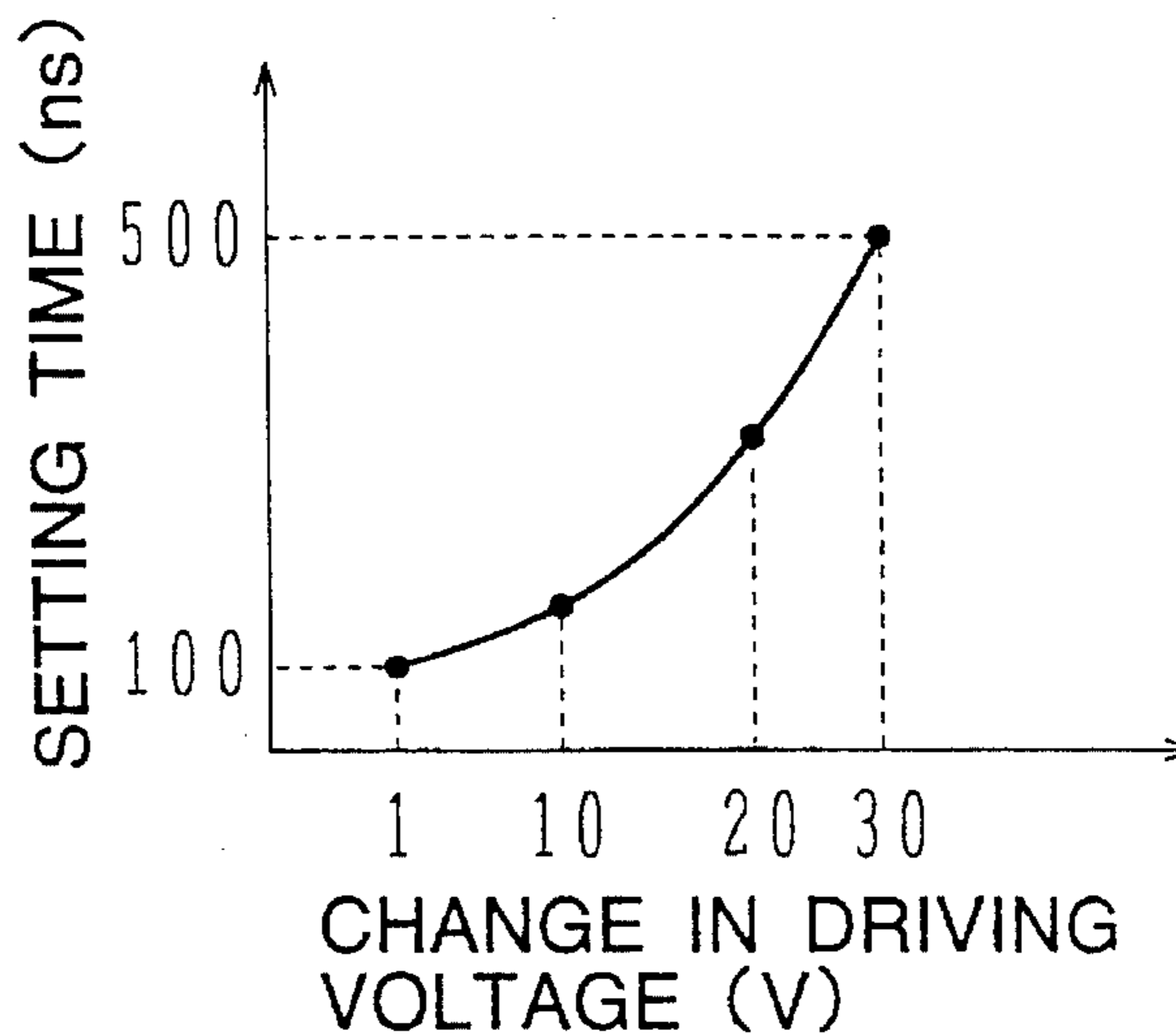
FIG.16C (PRIOR ART)
