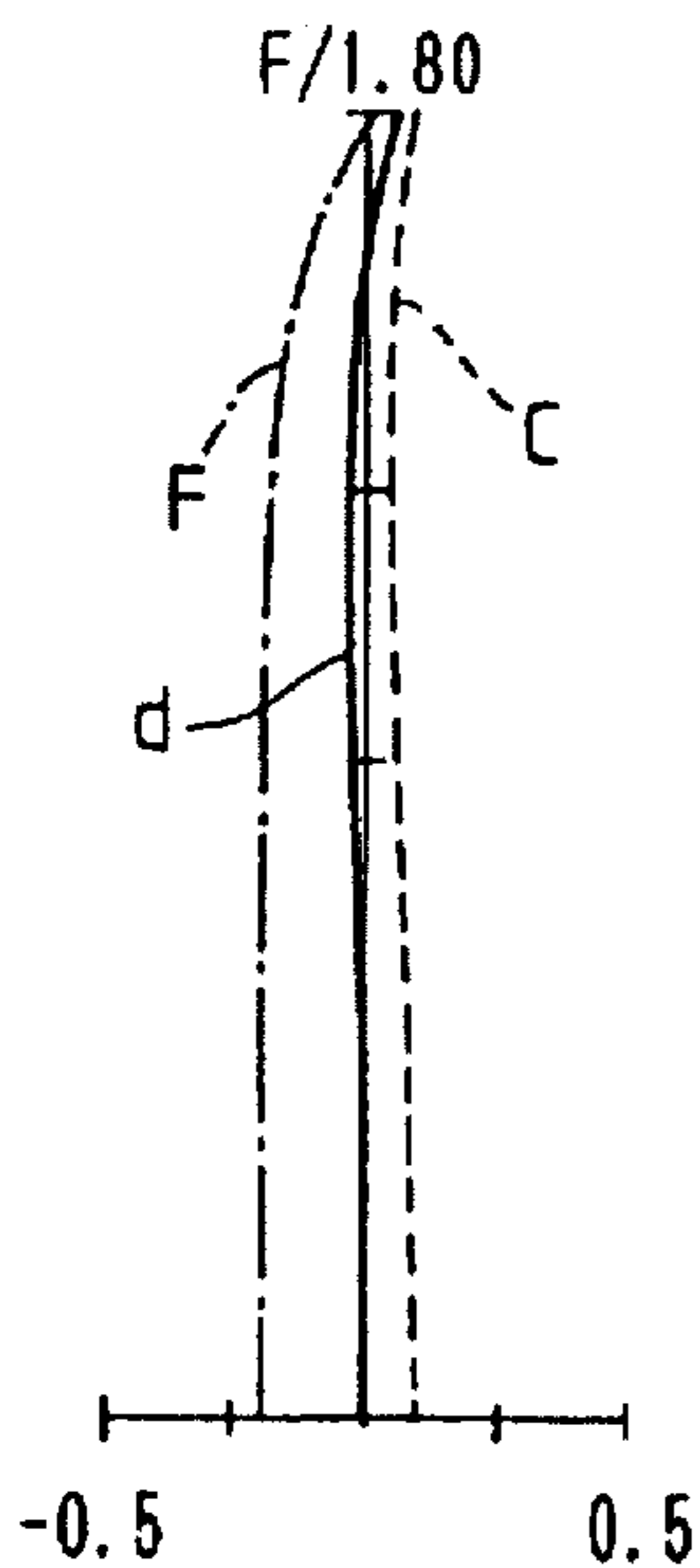
FIG. 14A SPHERICAL ABERRATION
