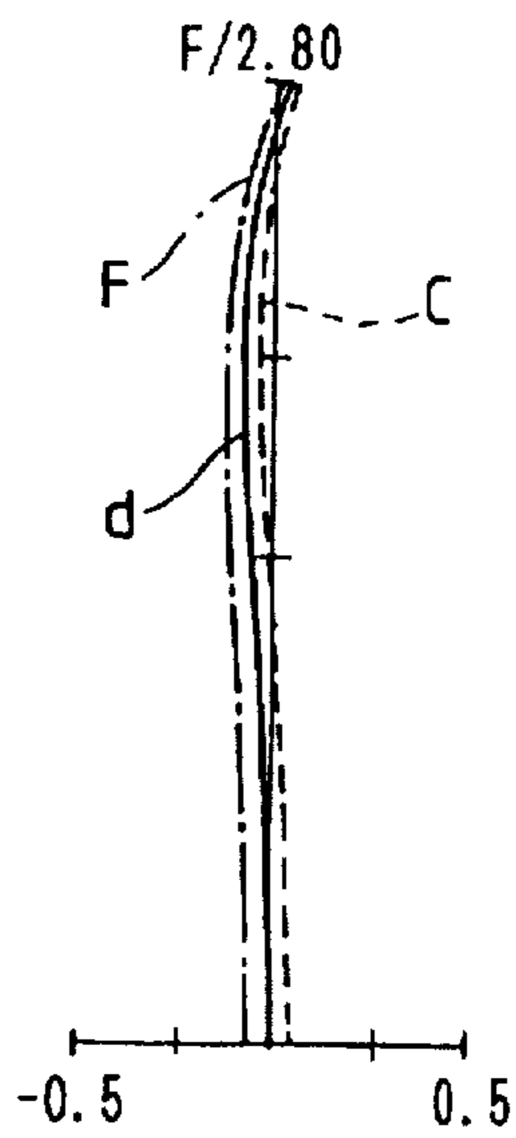
FIG. 6A SPHERICAL ABERRATION
