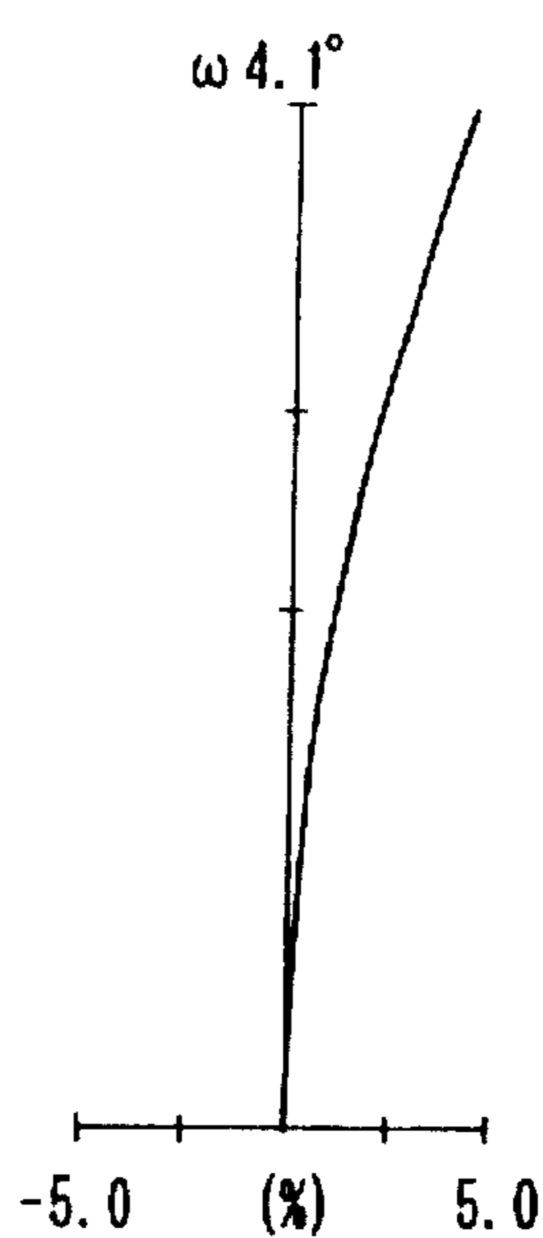
FIG. 11C DISTORTION
