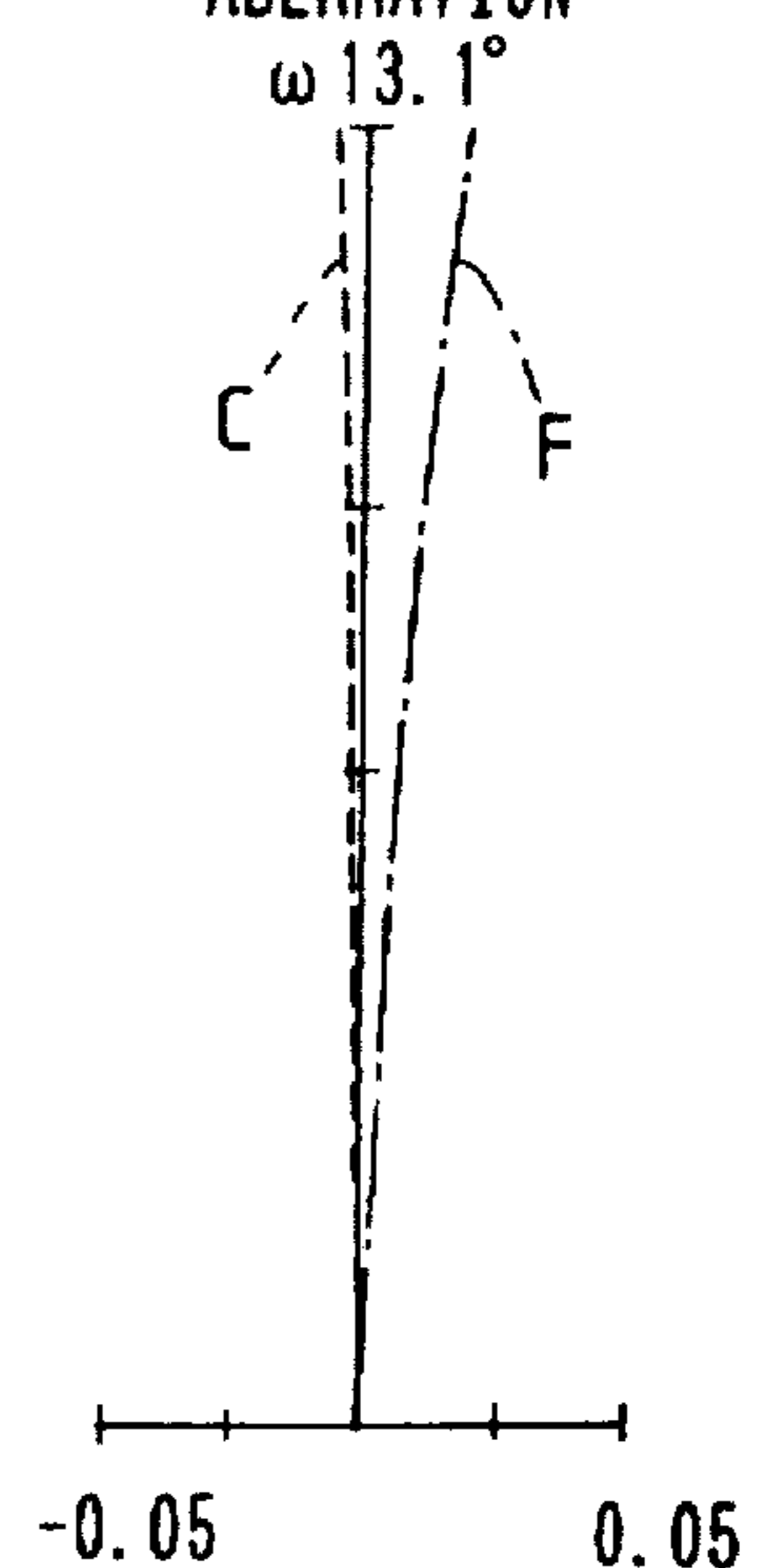
FIG. 13D LATERAL CHROMATIC ABERRATION
