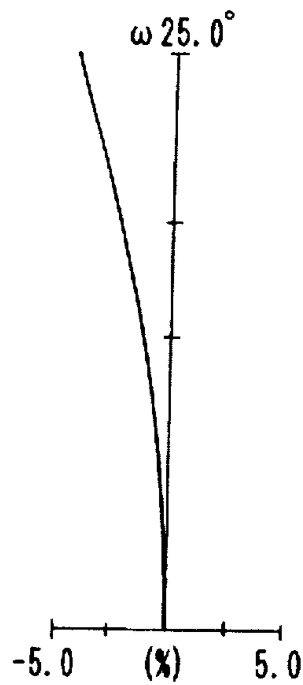
FIG. 5C DISTORTION
