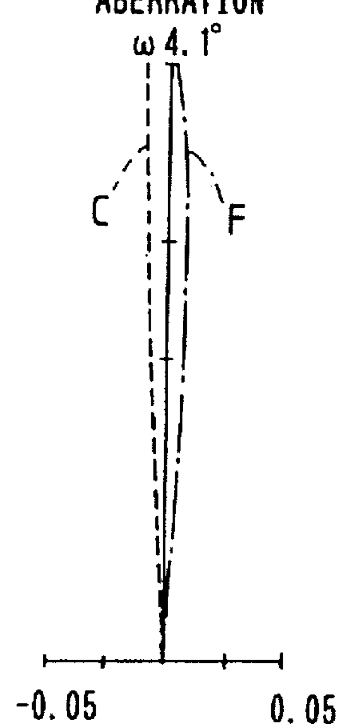
FIG. 11D LATERAL CHROMATIC ABERRATION
