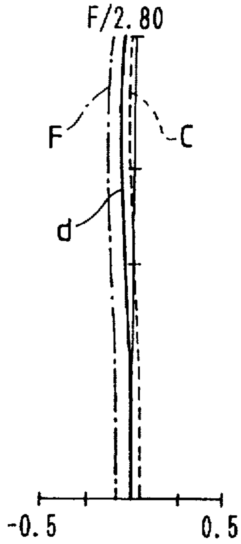
FIG. 5A SPHERICAL ABERRATION
