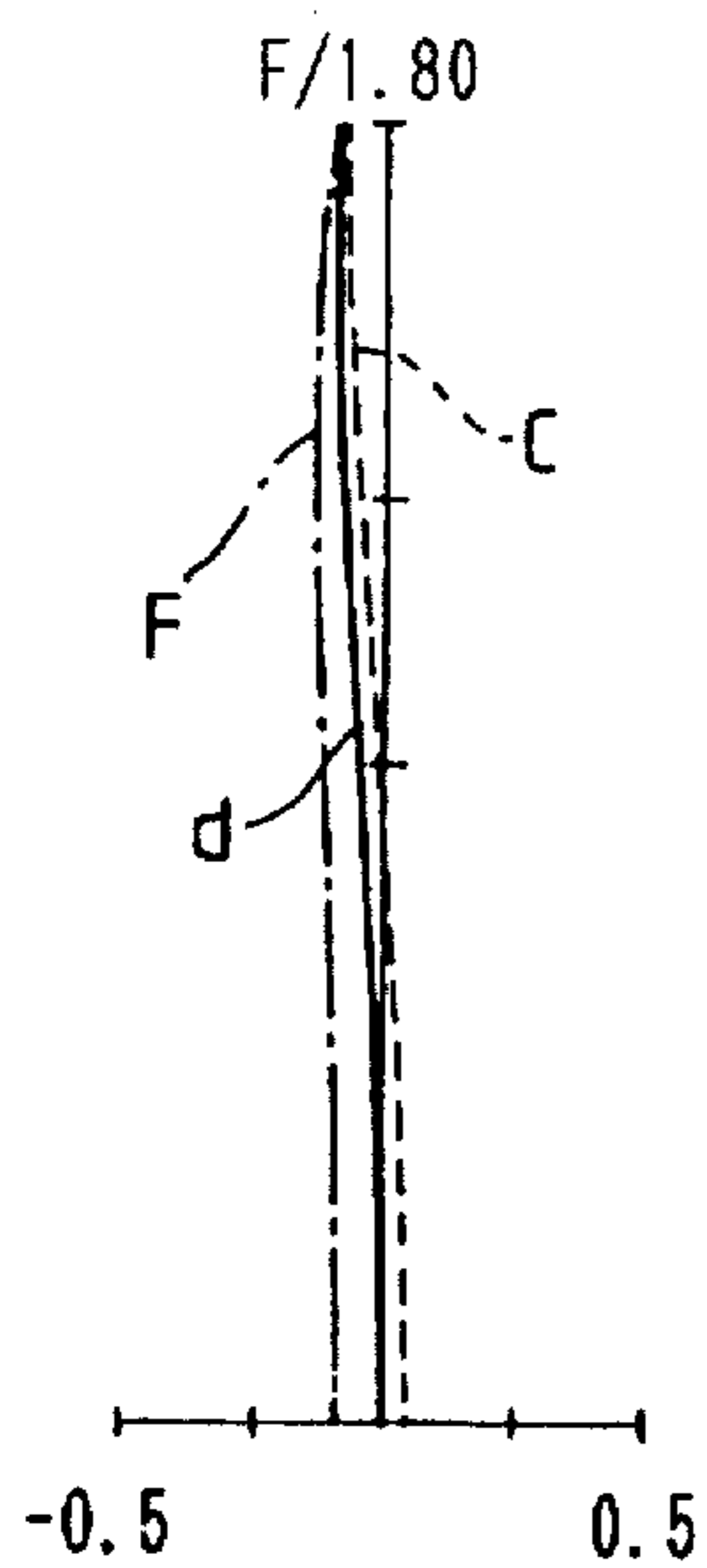
FIG. 12A SPHERICAL ABERRATION
