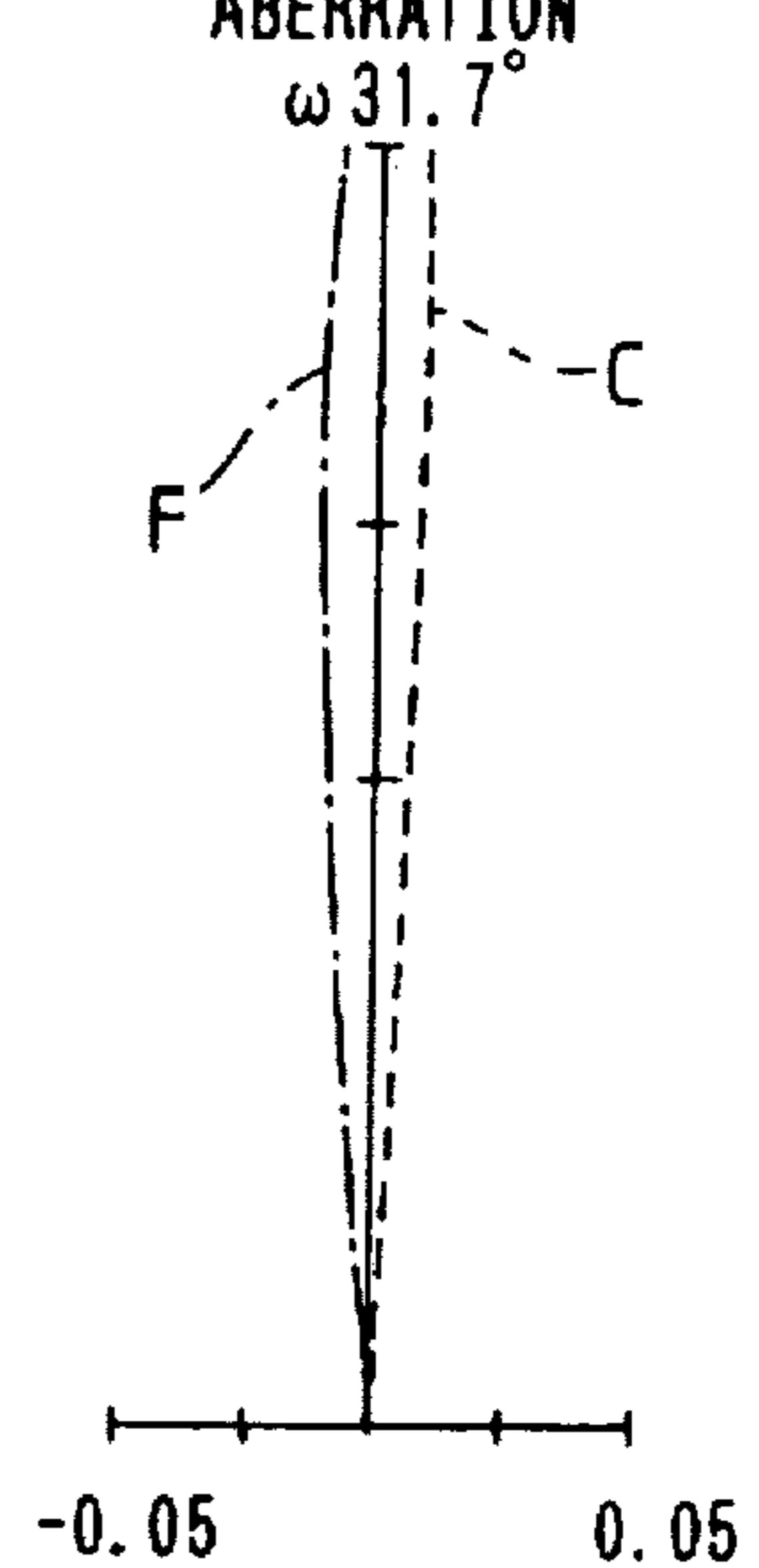
FIG. 8D LATERAL CHROMATIC ABERRATION
