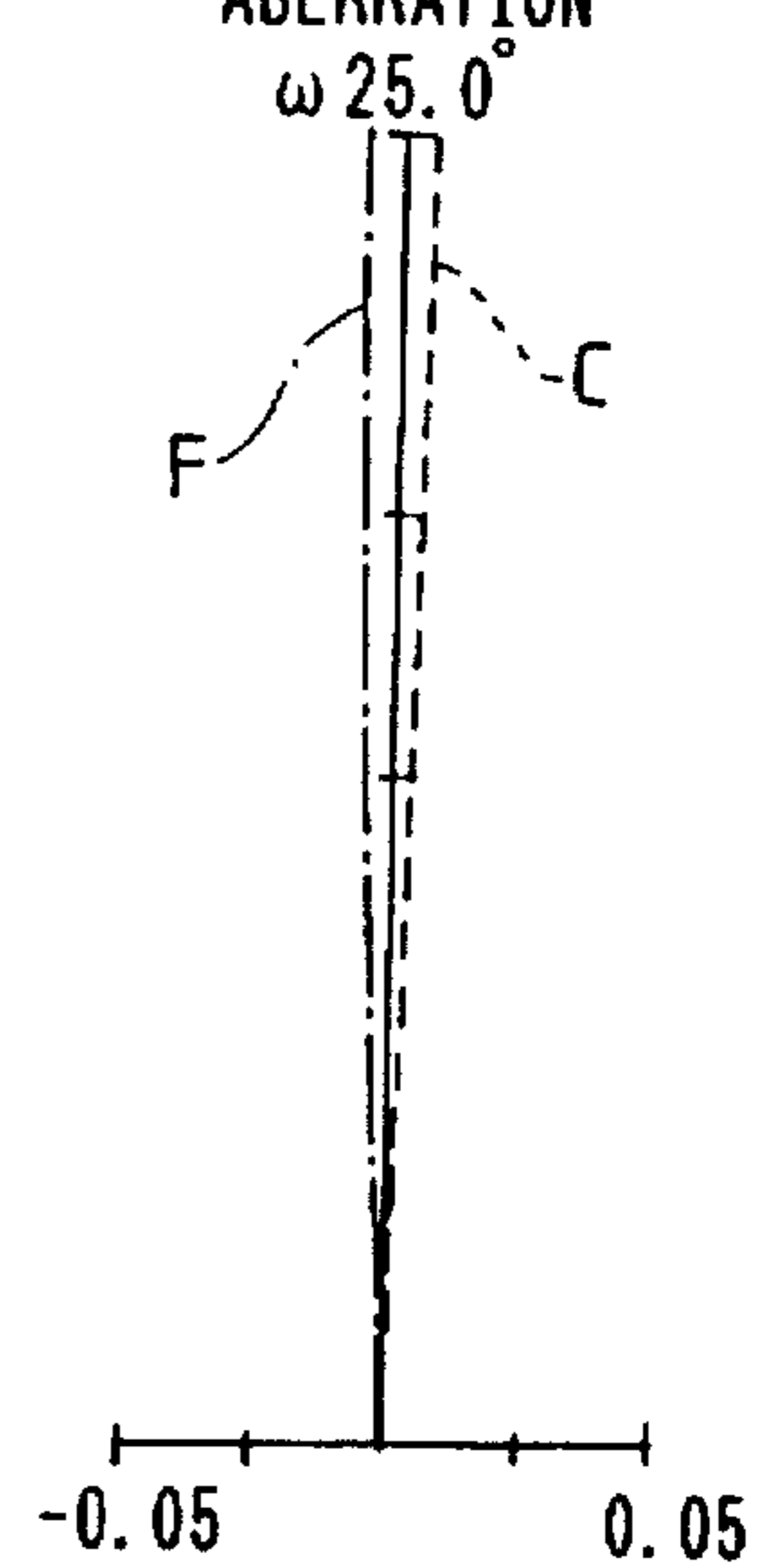
FIG. 5D LATERAL CHROMATIC ABERRATION
