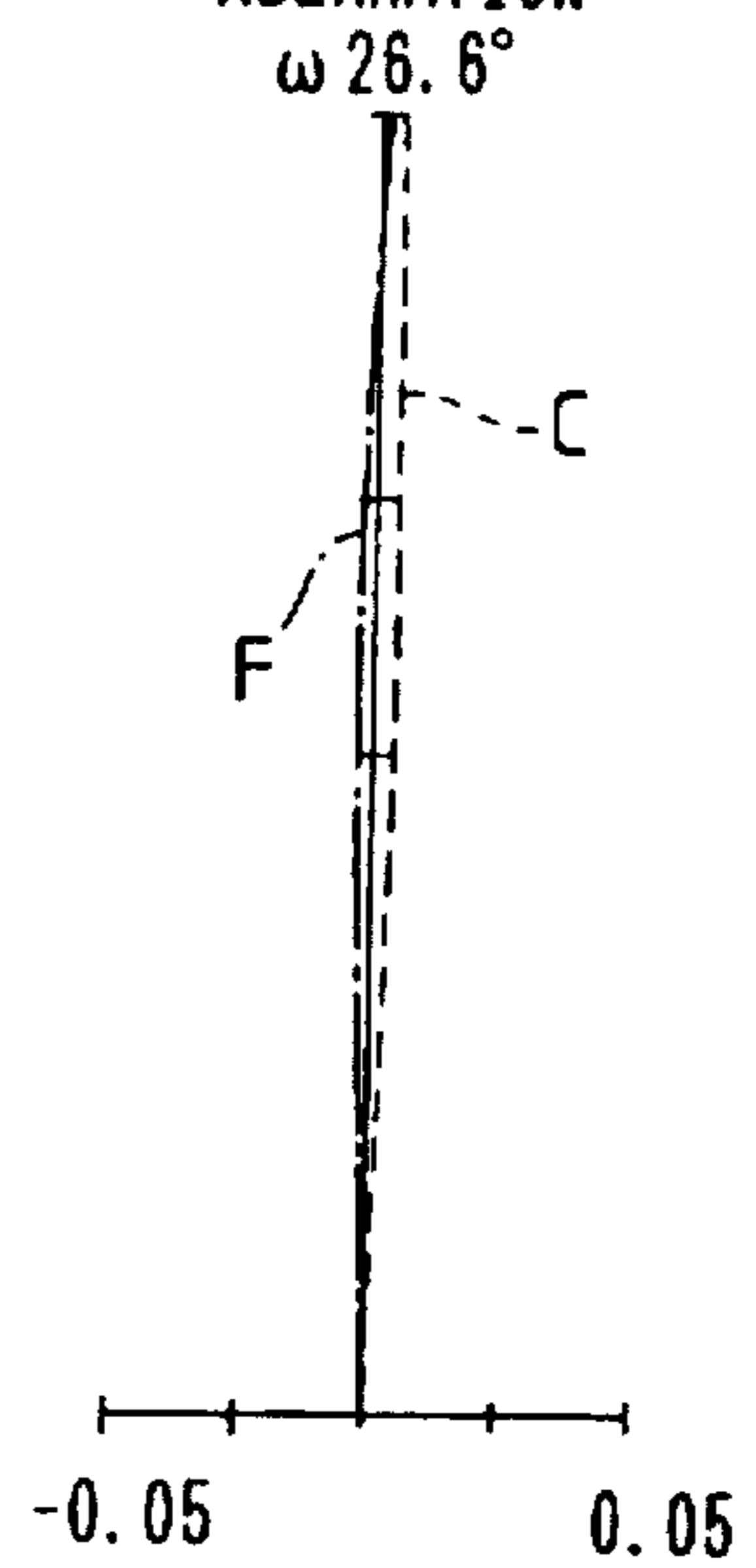
FIG. 9D LATERAL CHROMATIC ABERRATION
