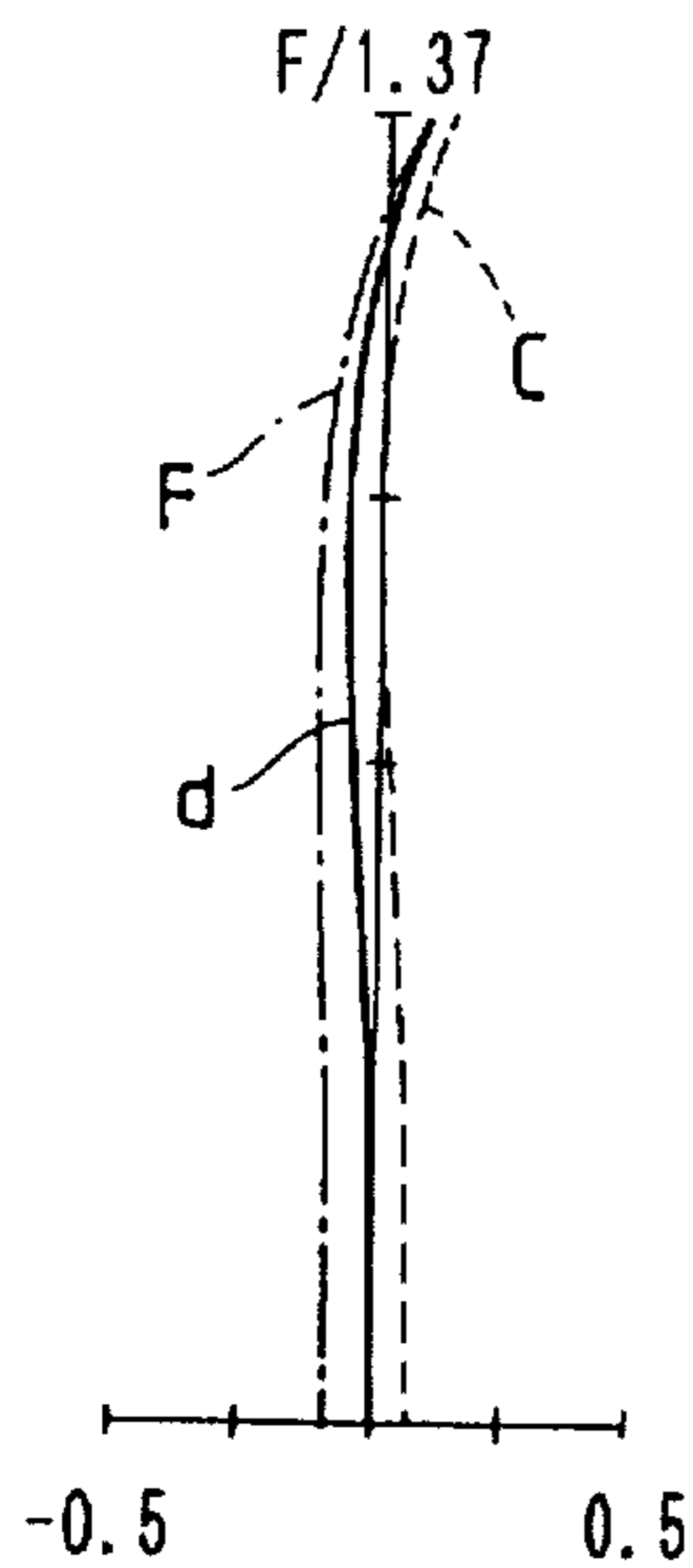
FIG. 11A SPHERICAL ABERRATION
