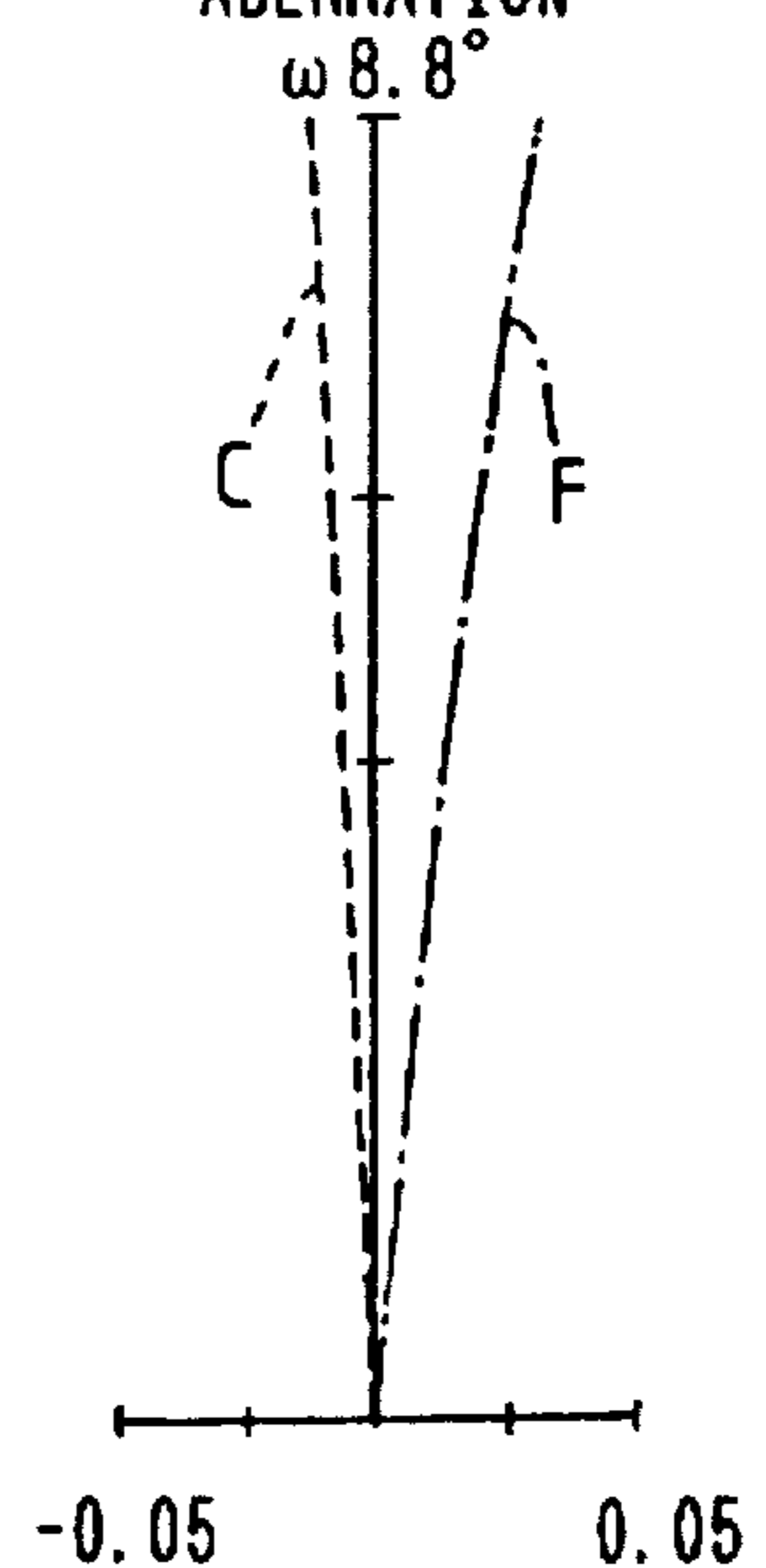
FIG. 14D LATERAL CHROMATIC ABERRATION
