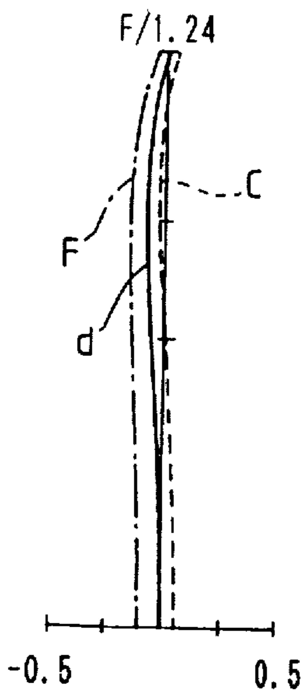
FIG. 10A SPHERICAL ABERRATION
