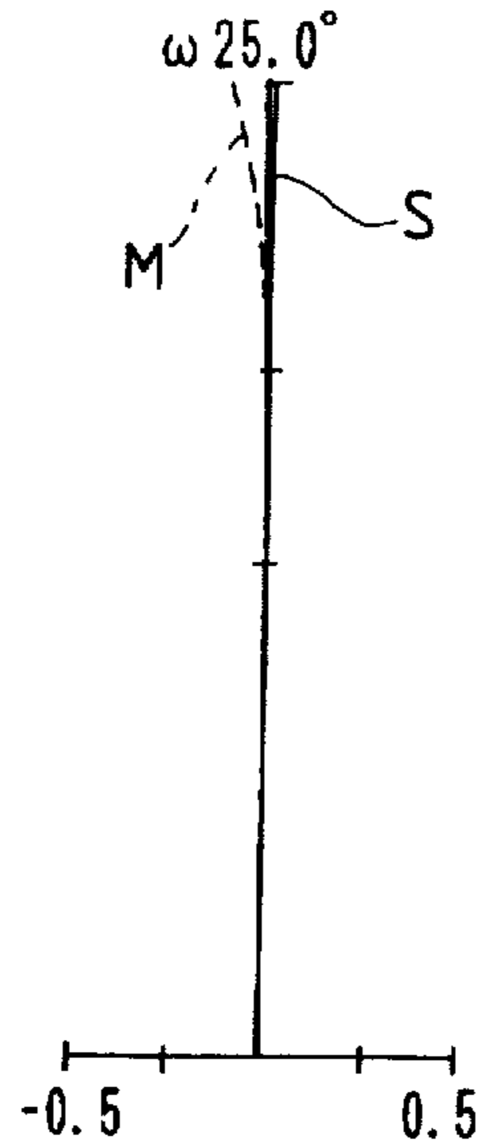
FIG. 5B ASTIGMATISM
