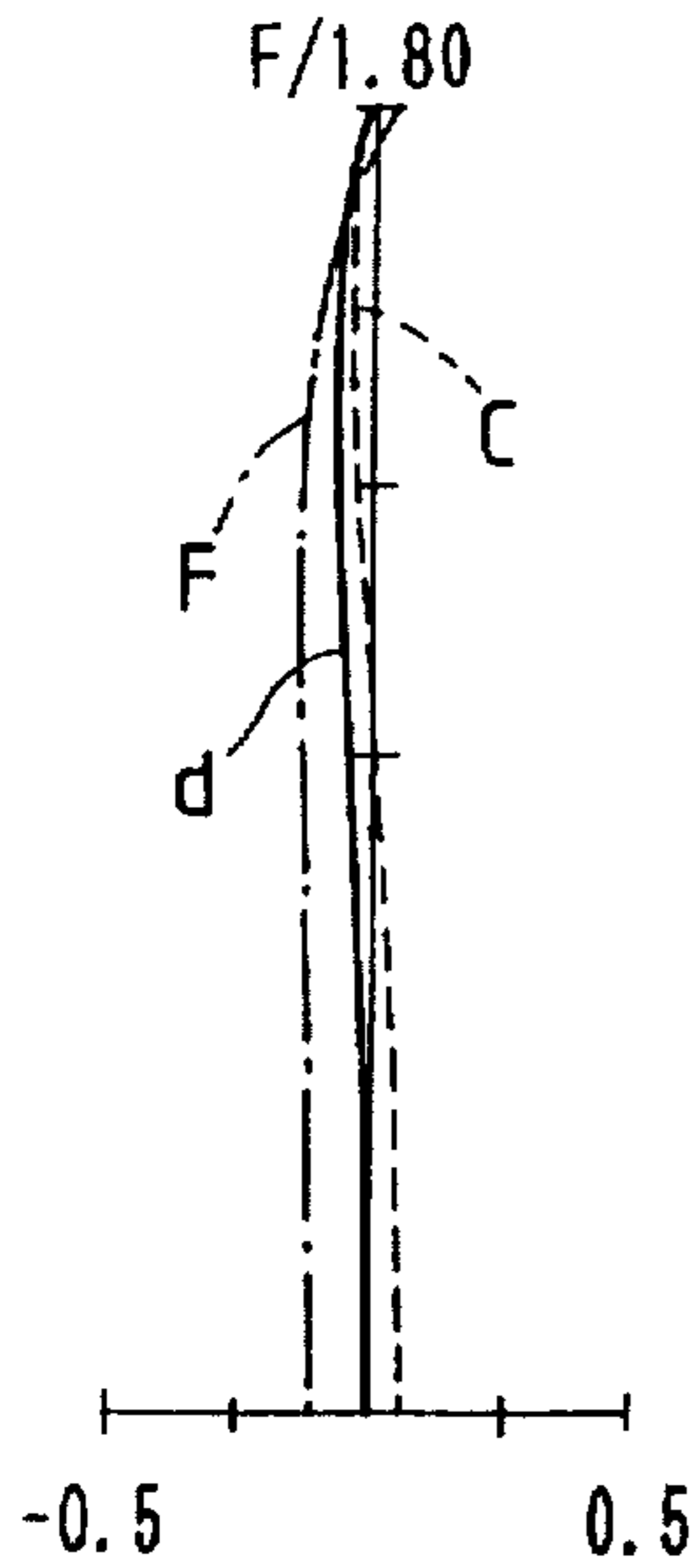
FIG. 13A SPHERICAL ABERRATION
