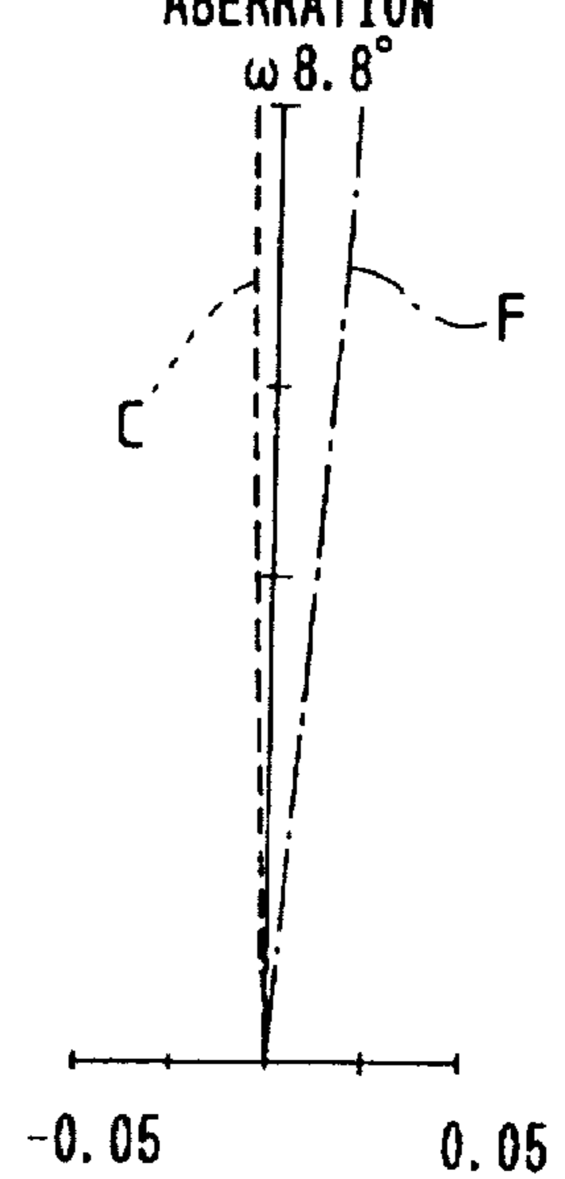
FIG. 7D LATERAL CHROMATIC ABERRATION
