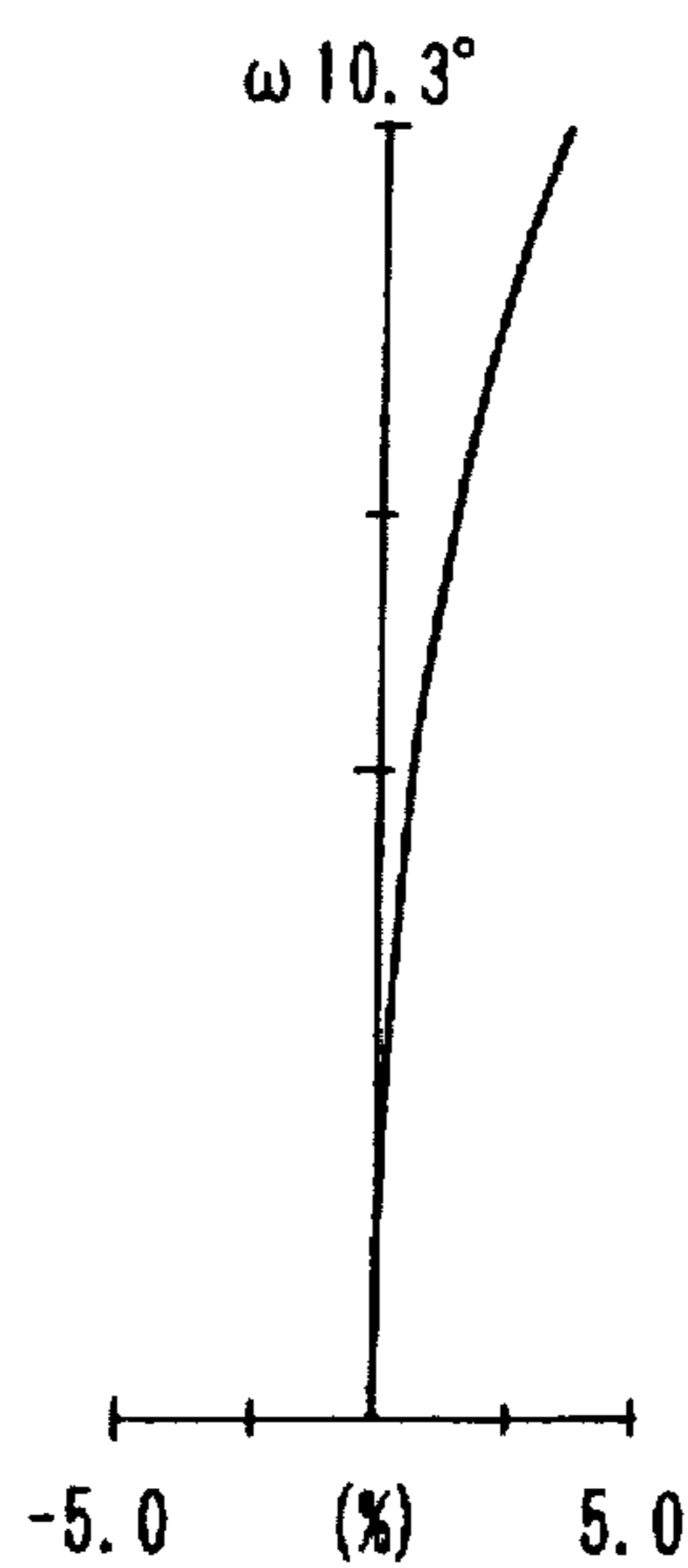
FIG. 10C DISTORTION
