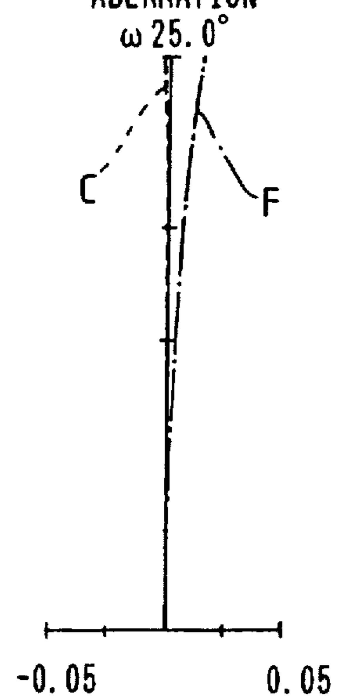
FIG. 12D LATERAL CHROMATIC ABERRATION
