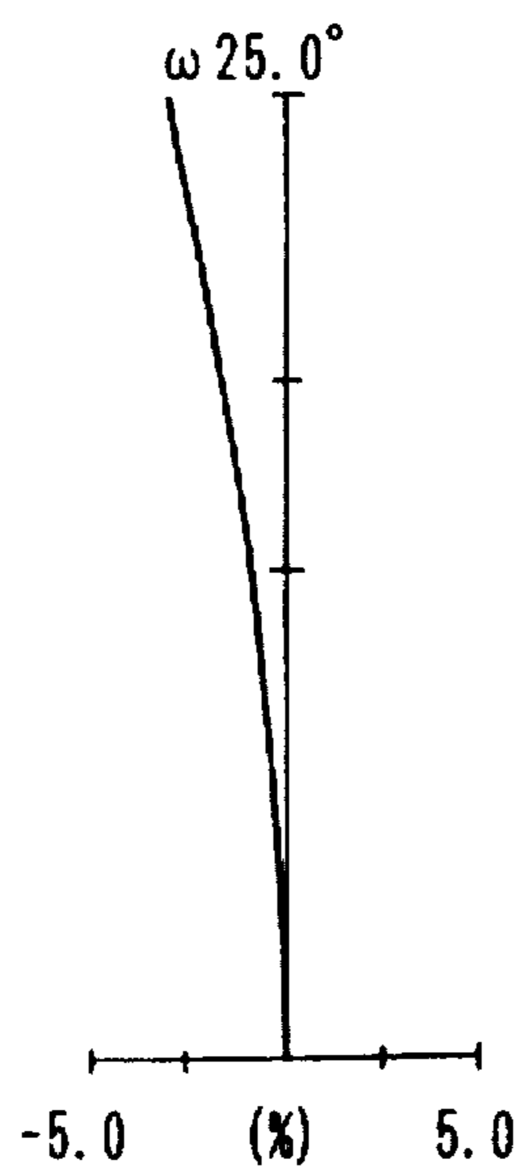
FIG. 12C DISTORTION
