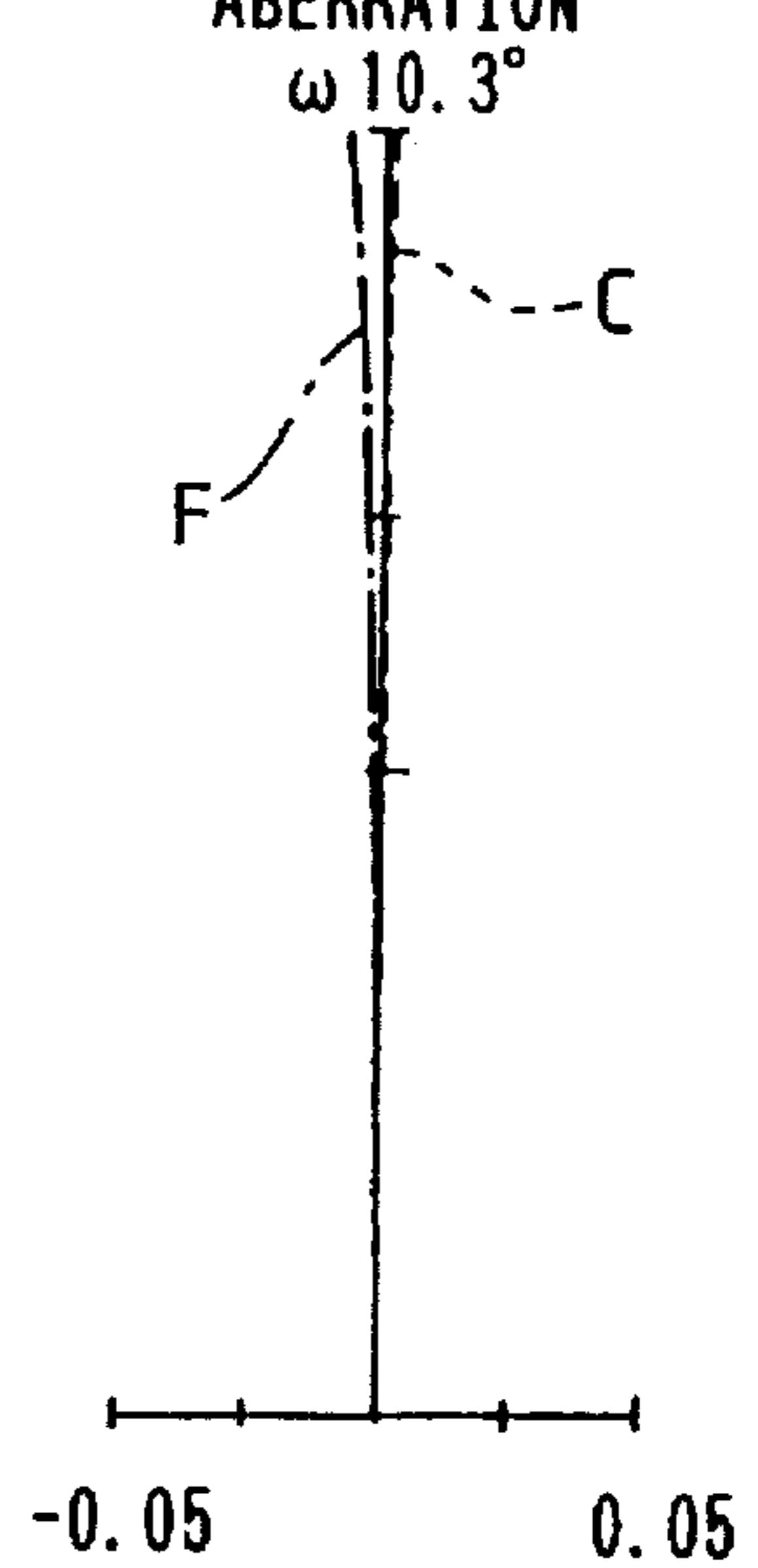
FIG. 10D LATERAL CHROMATIC ABERRATION
