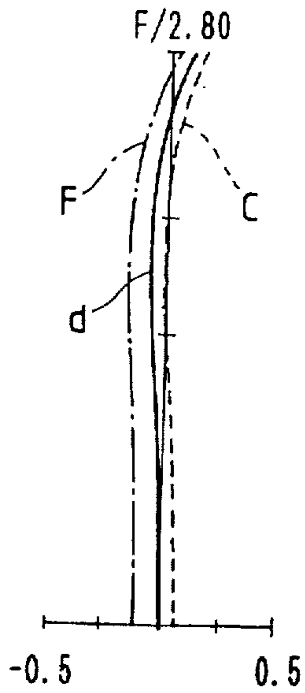
FIG. 7A SPHERICAL ABERRATION
