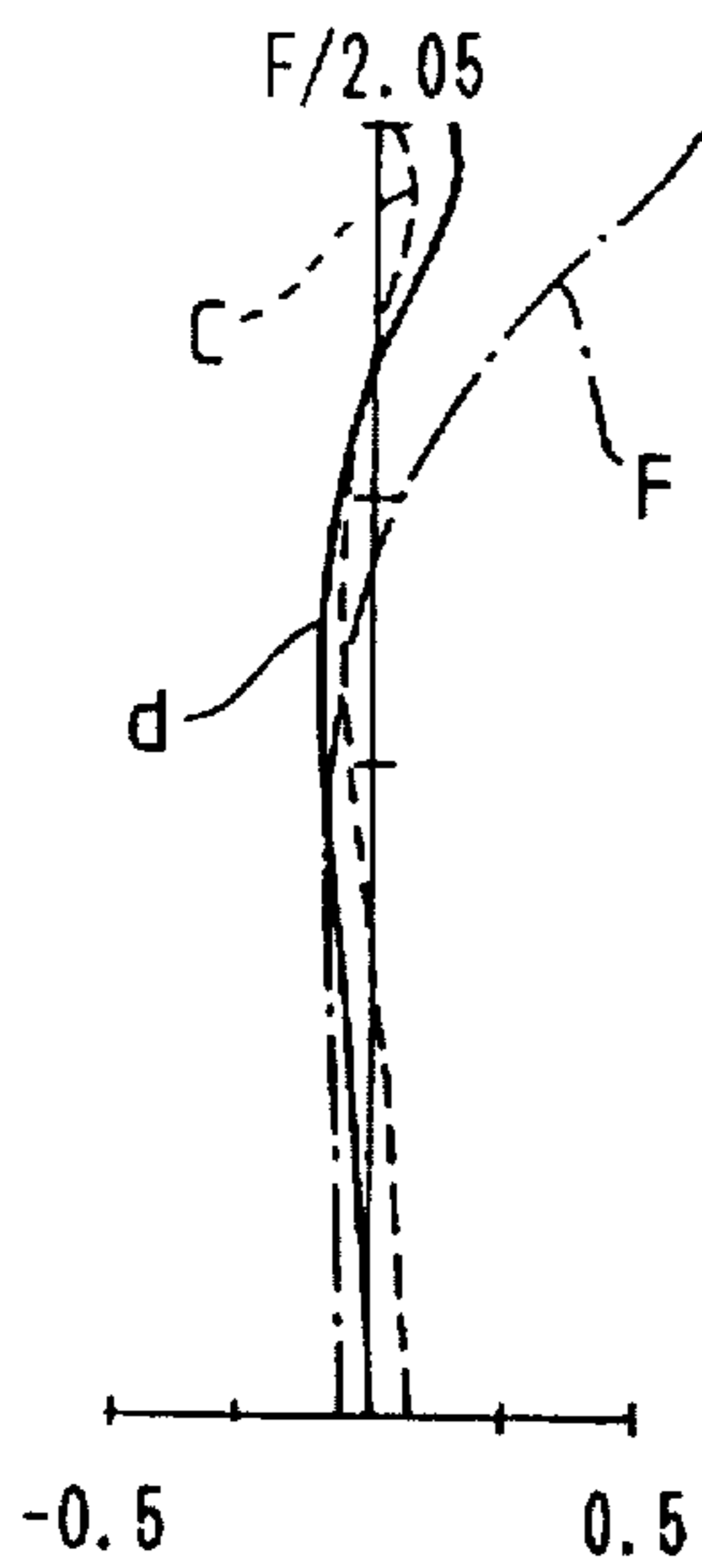
FIG. 8A SPHERICAL ABERRATION
