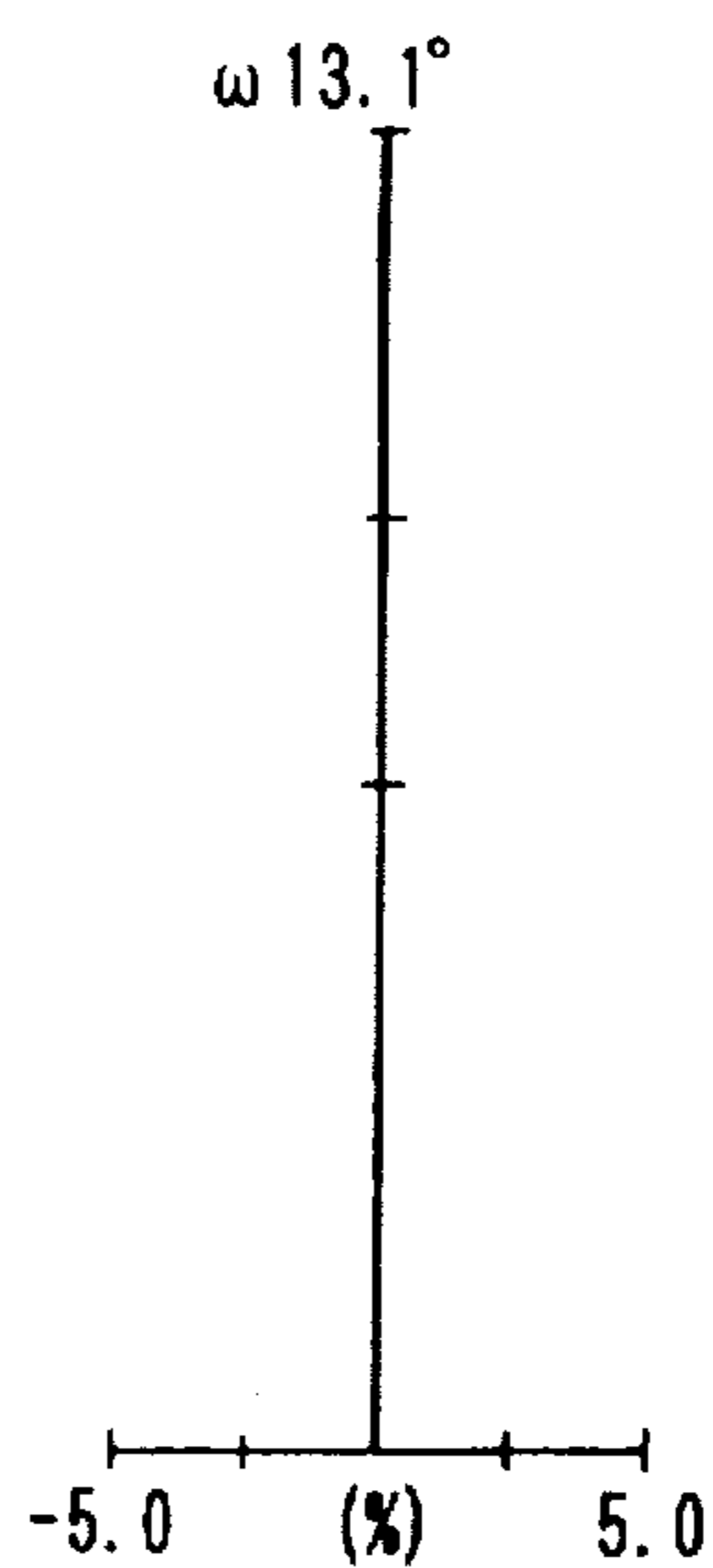
FIG. 6C DISTORTION
