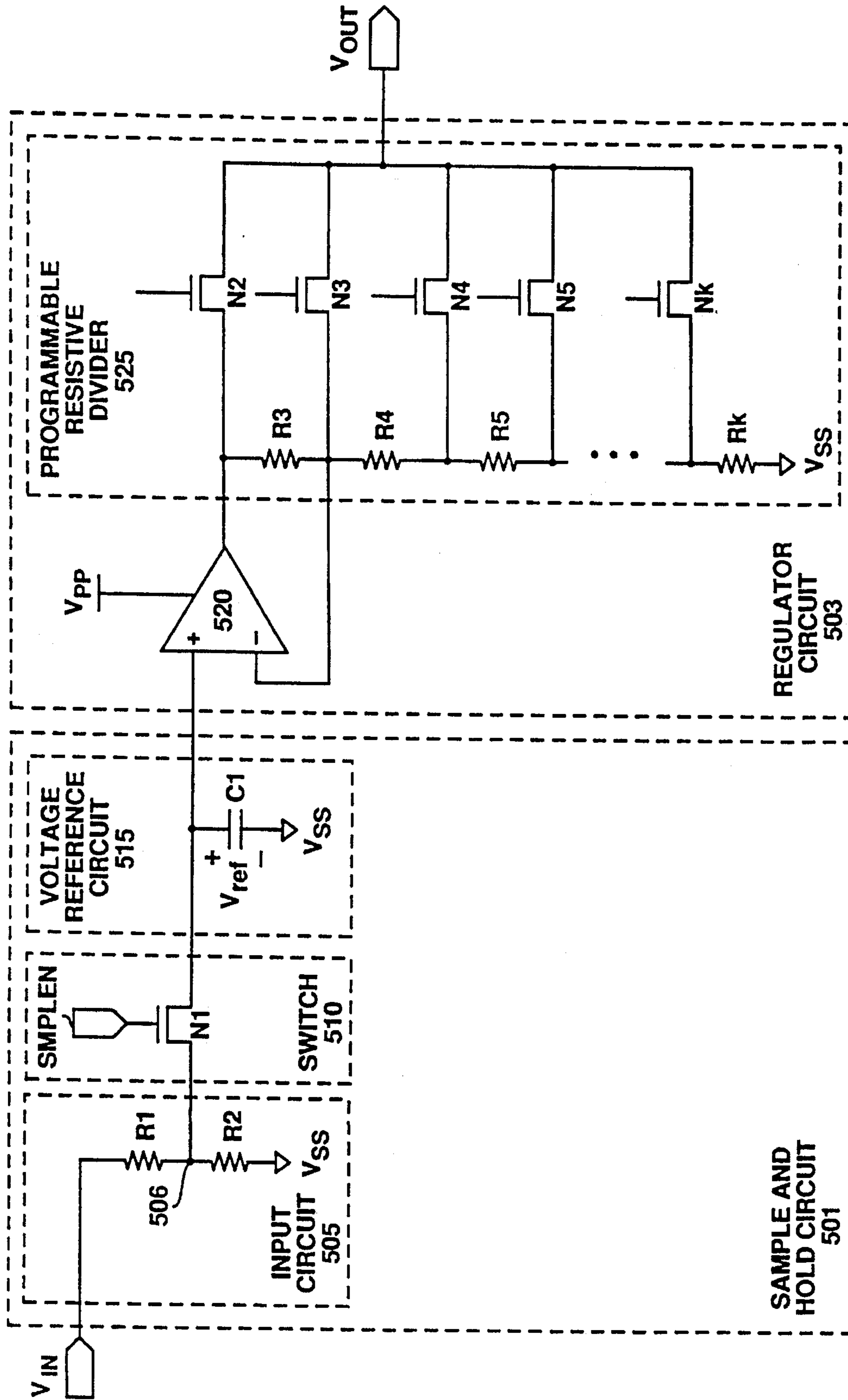
PROGRAMMING VOLTAGE REGULATION CIRCUIT 45
