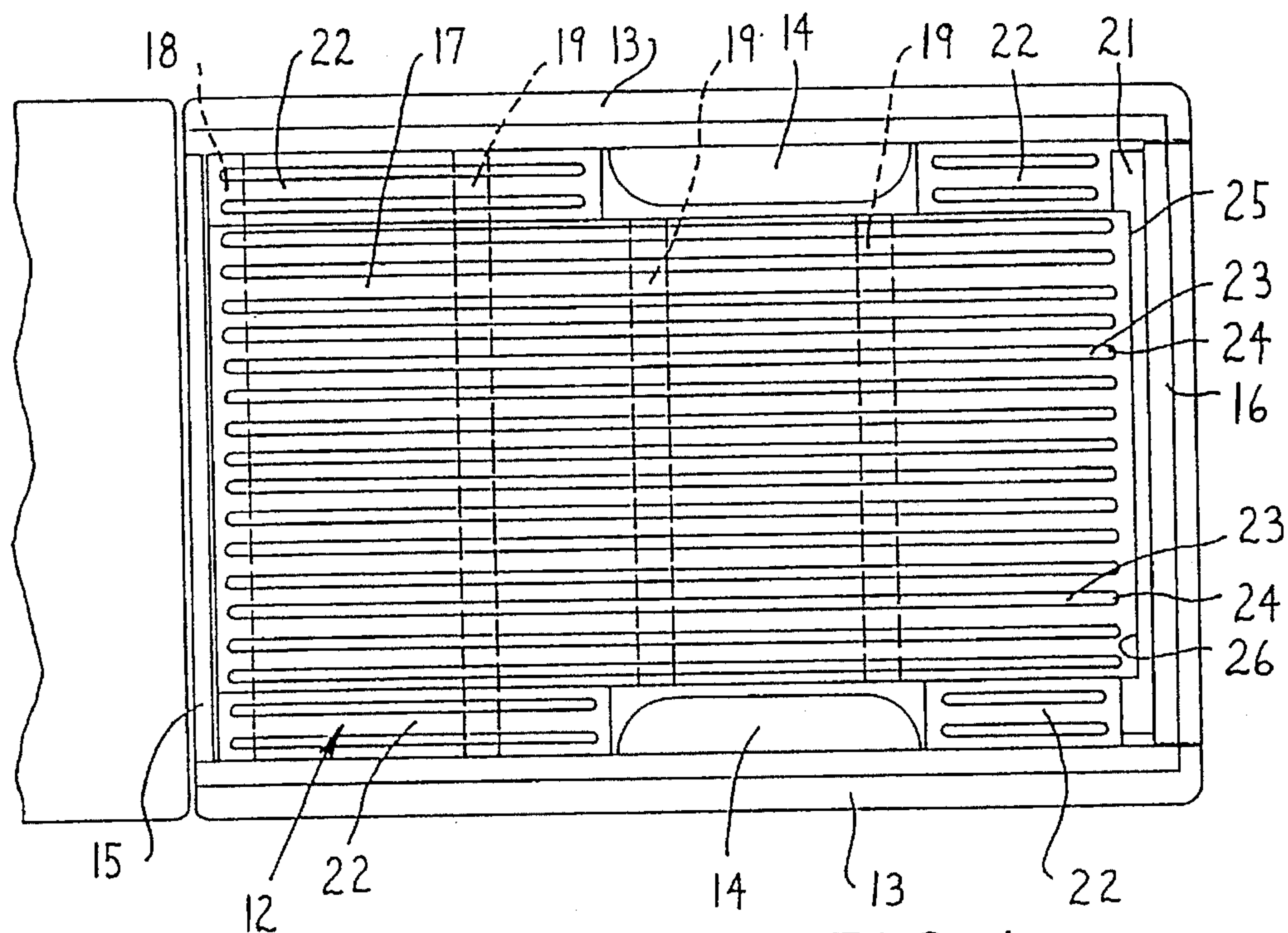
FIG. 1 PRIOR ART
