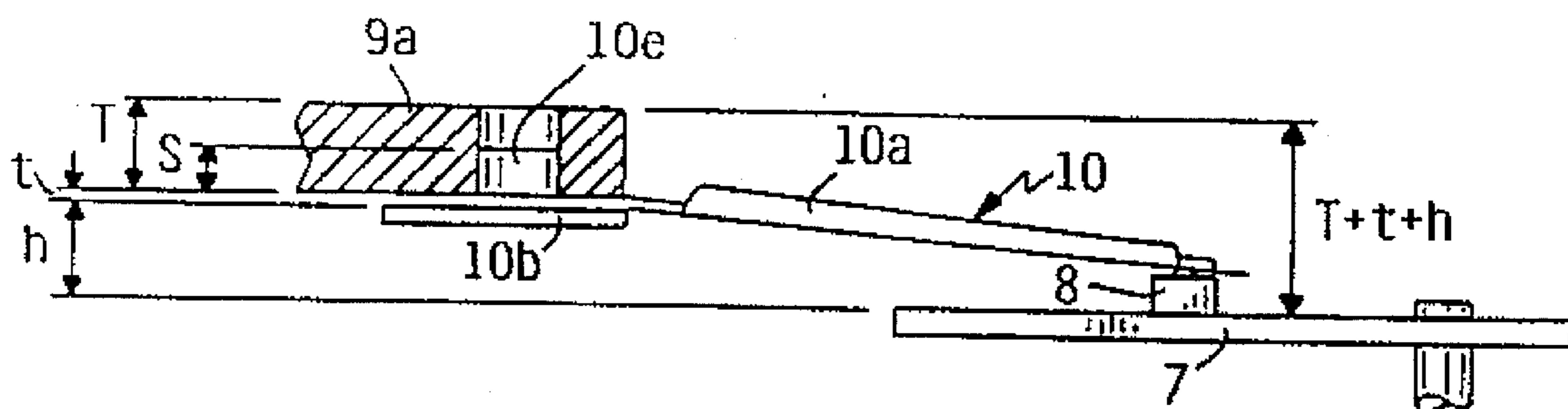
FIG. 7 (PRIOR ART)
