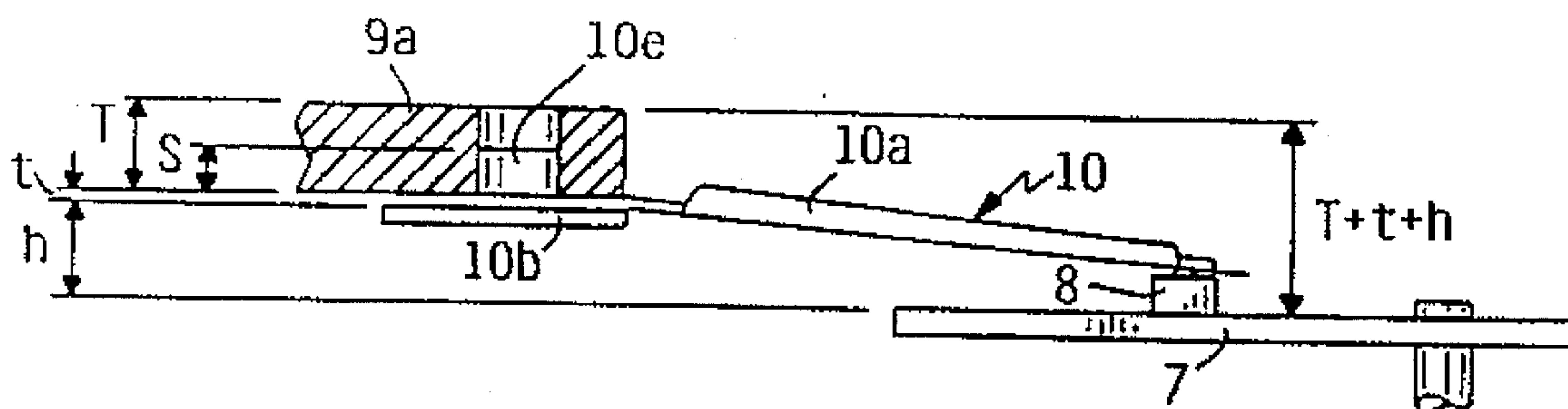
FIG. 7 (PRIOR ART)
