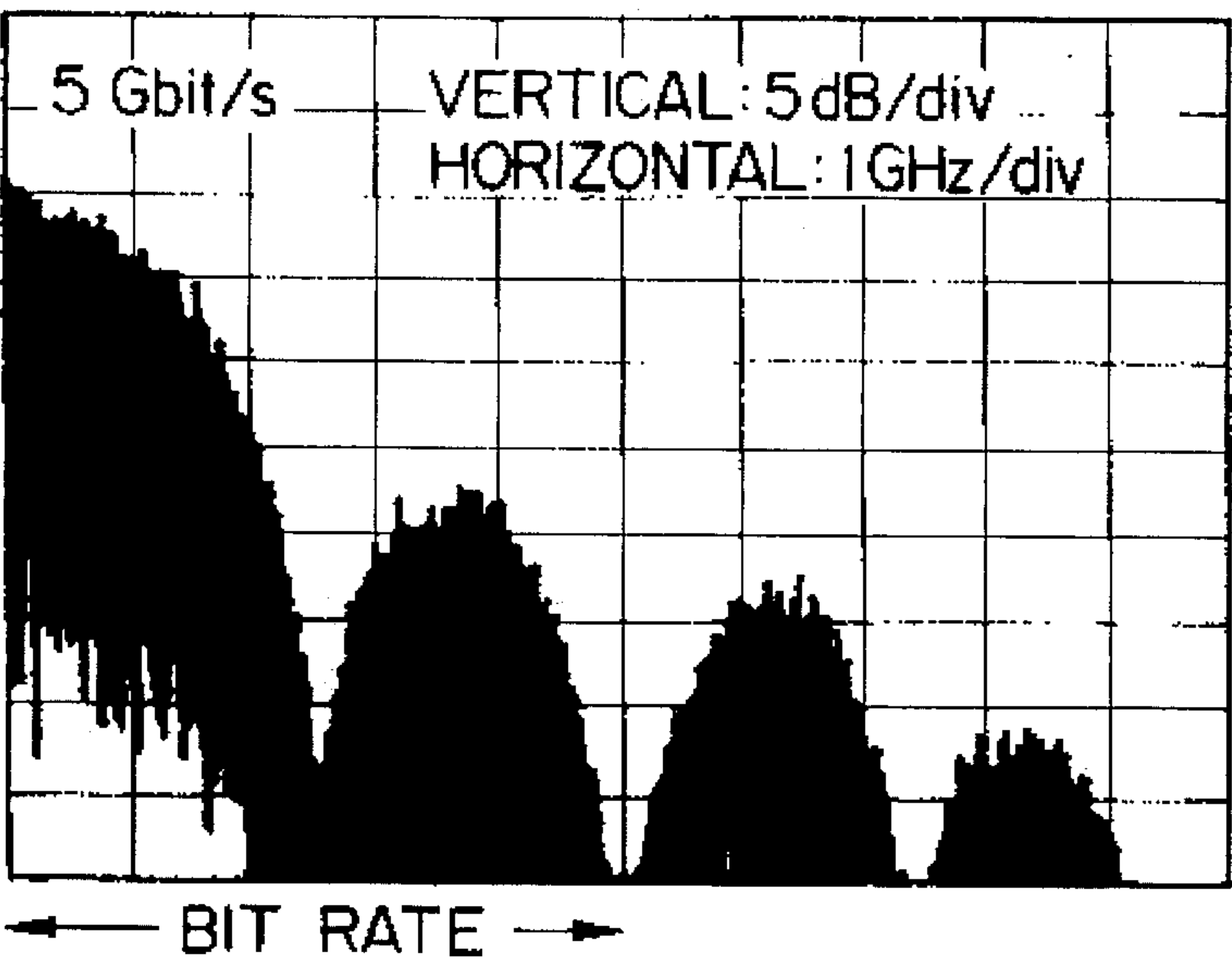
DUOBINARY SIGNAL SPECTRUM
