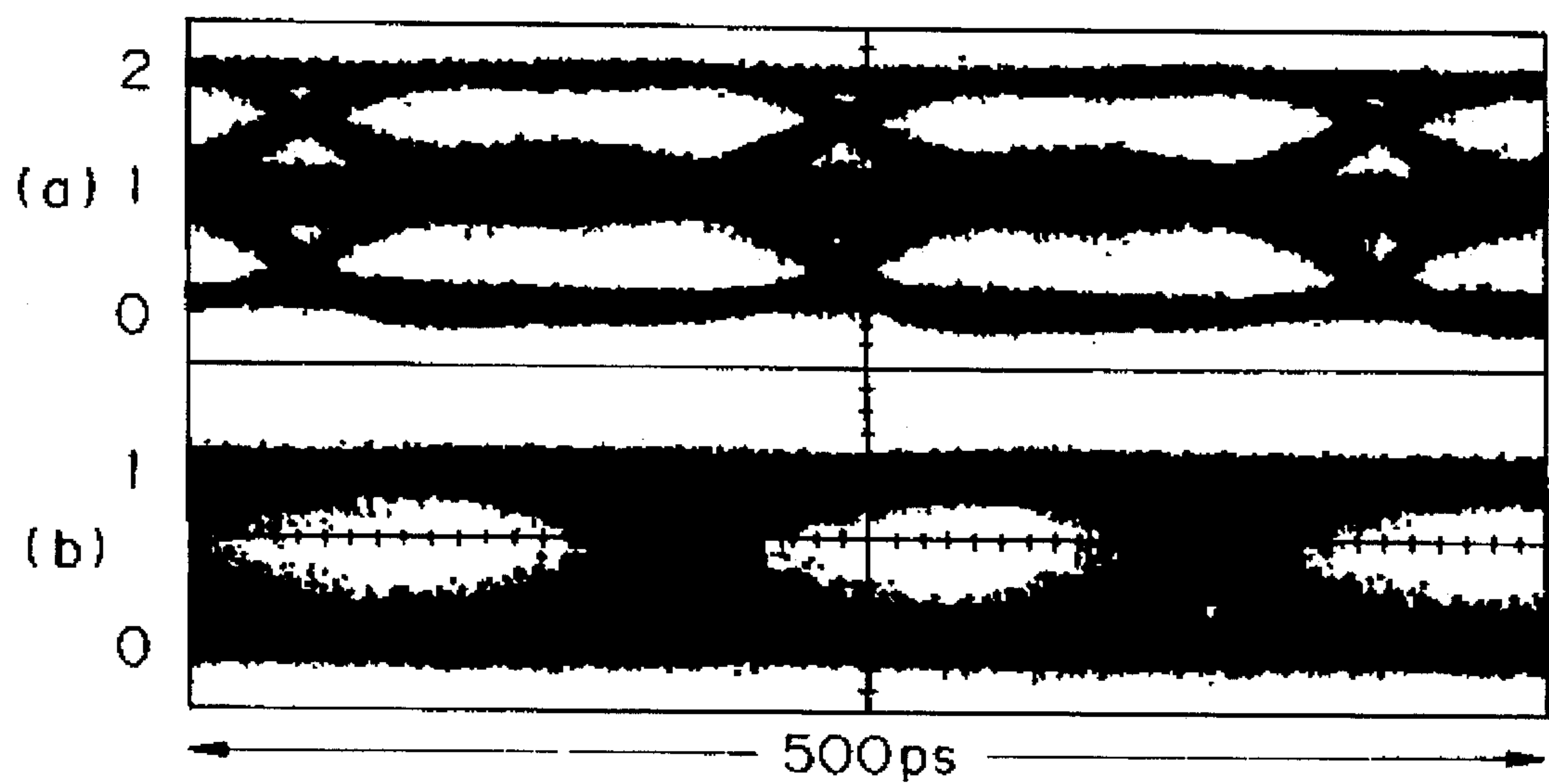
DUOBINARY SIGNAL WAVEFORM, AND RECEIVED SIGNAL WAVEFORM
