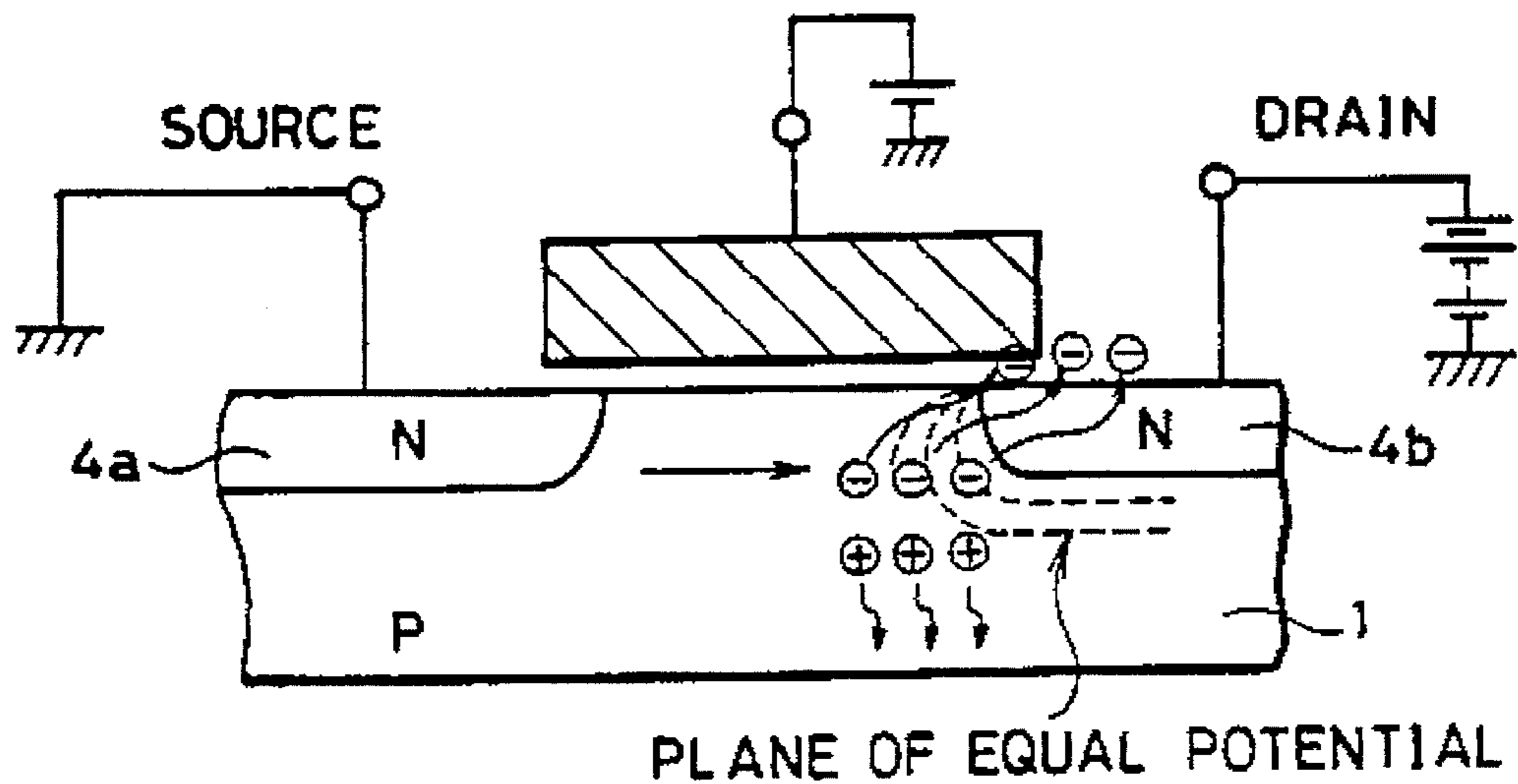
FIG. 3 PRIOR ART
