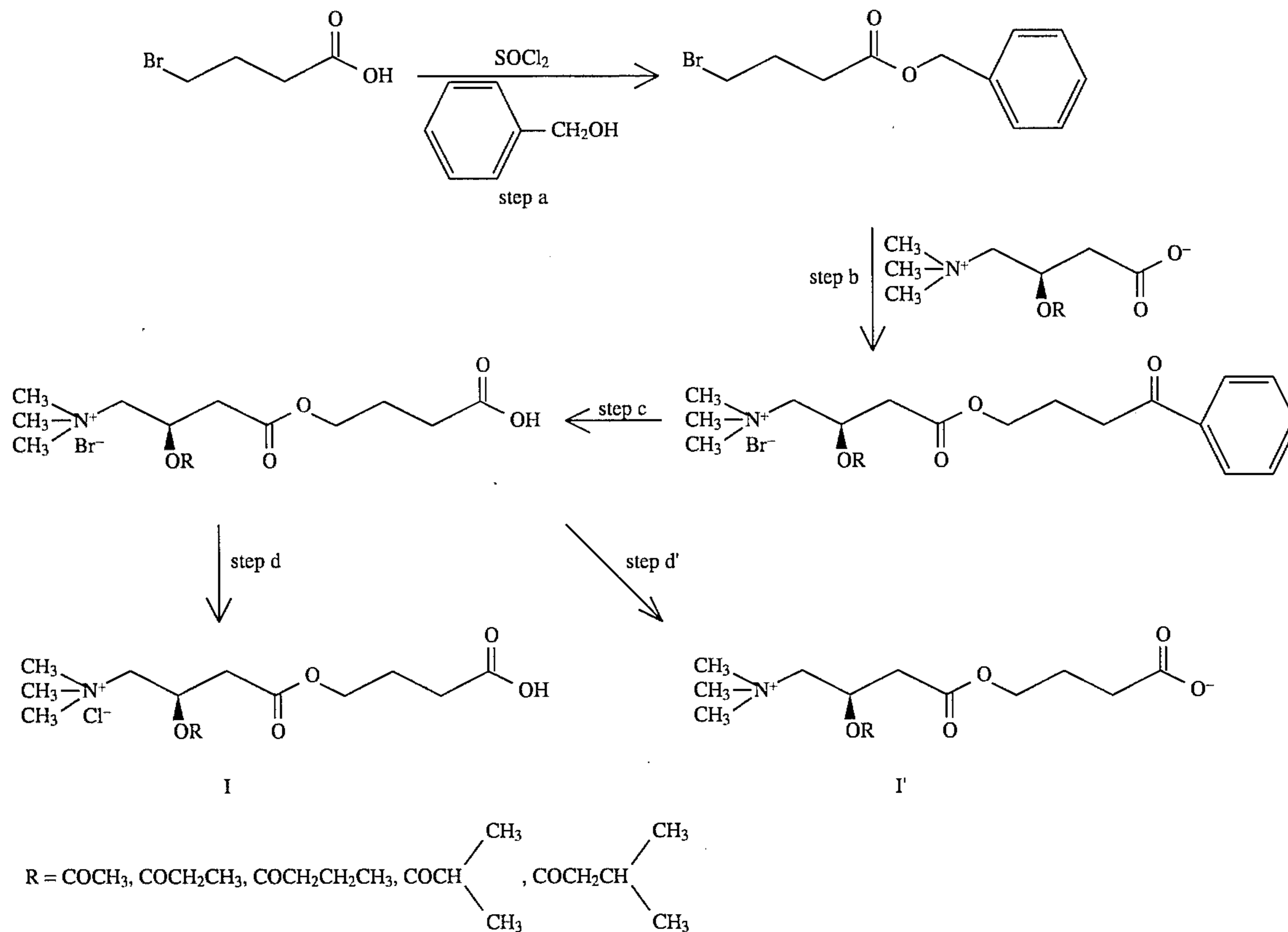
Synthesis scheme of the esters of acyl L-carnitines with gamma-hydroxybutyric acid
