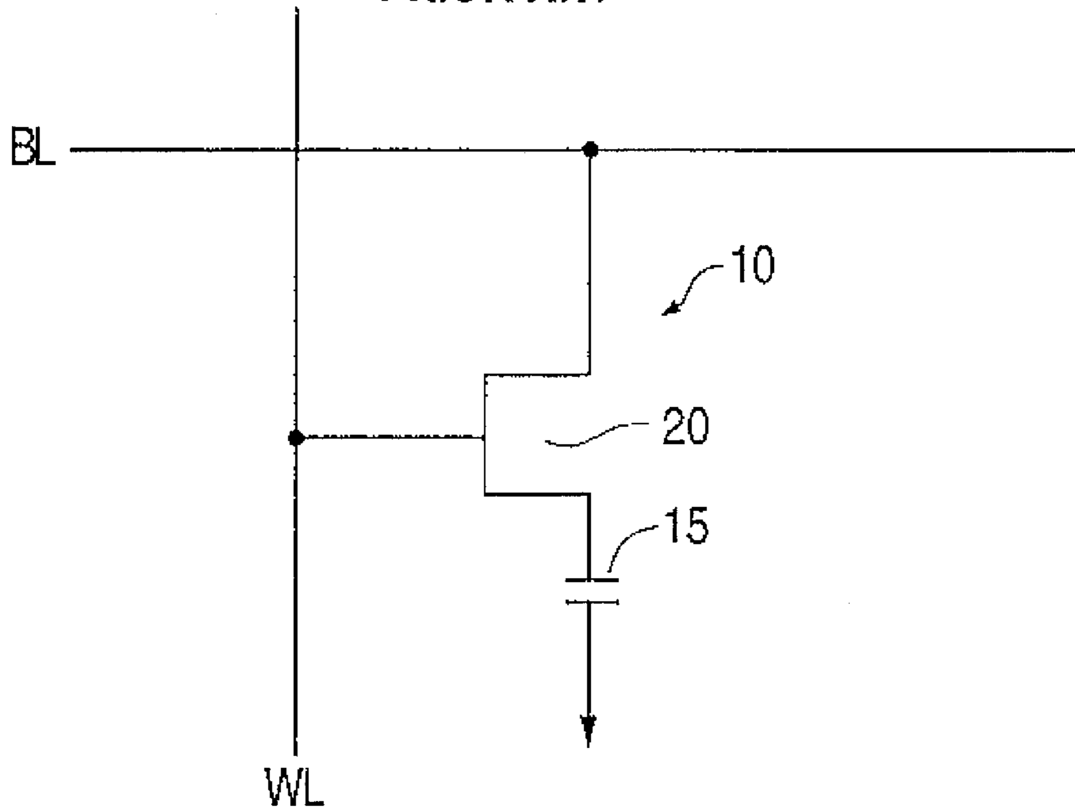
FIG. 1 PRIOR ART
