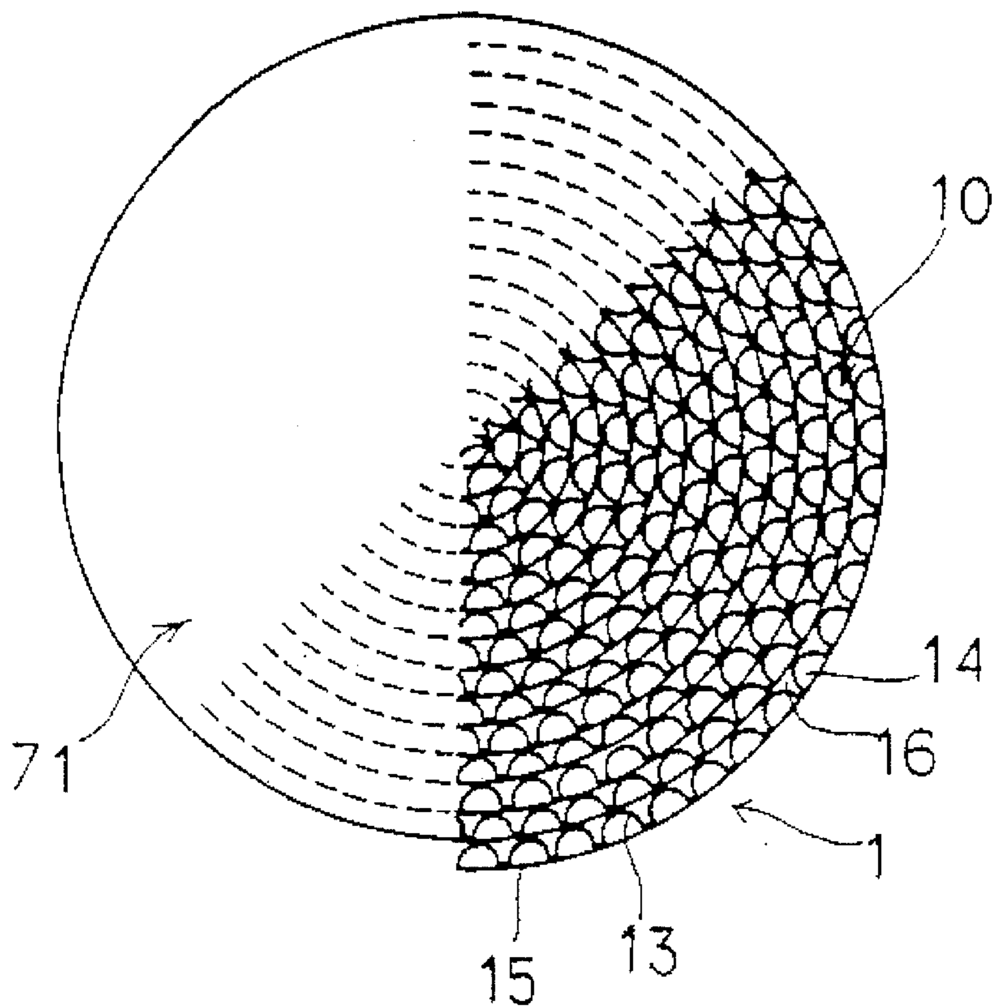
FIG. 24 PRIOR ART
