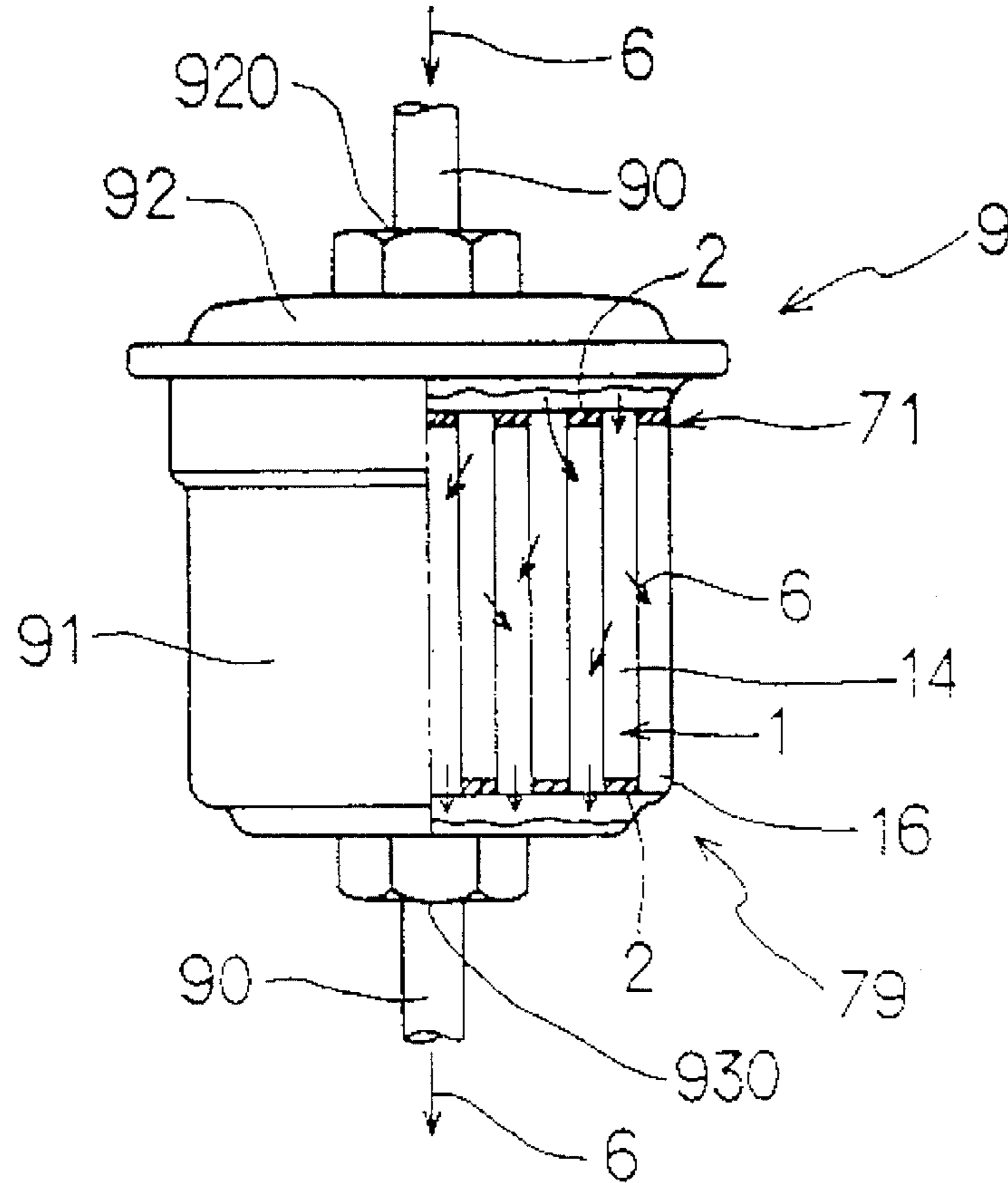
FIG. 22 PRIOR ART
