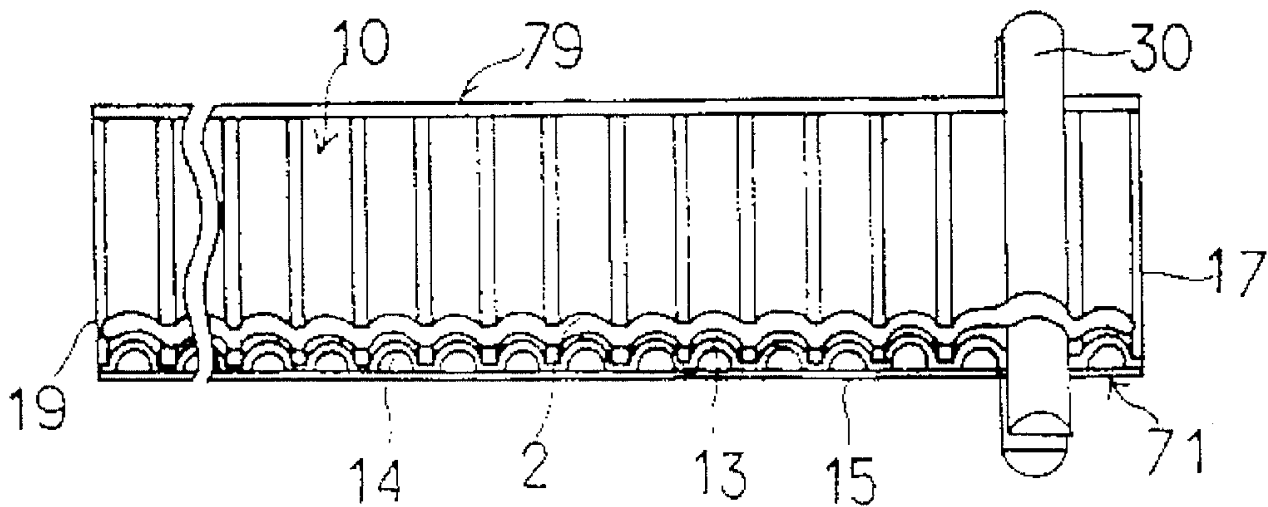
FIG. 28 PRIOR ART
