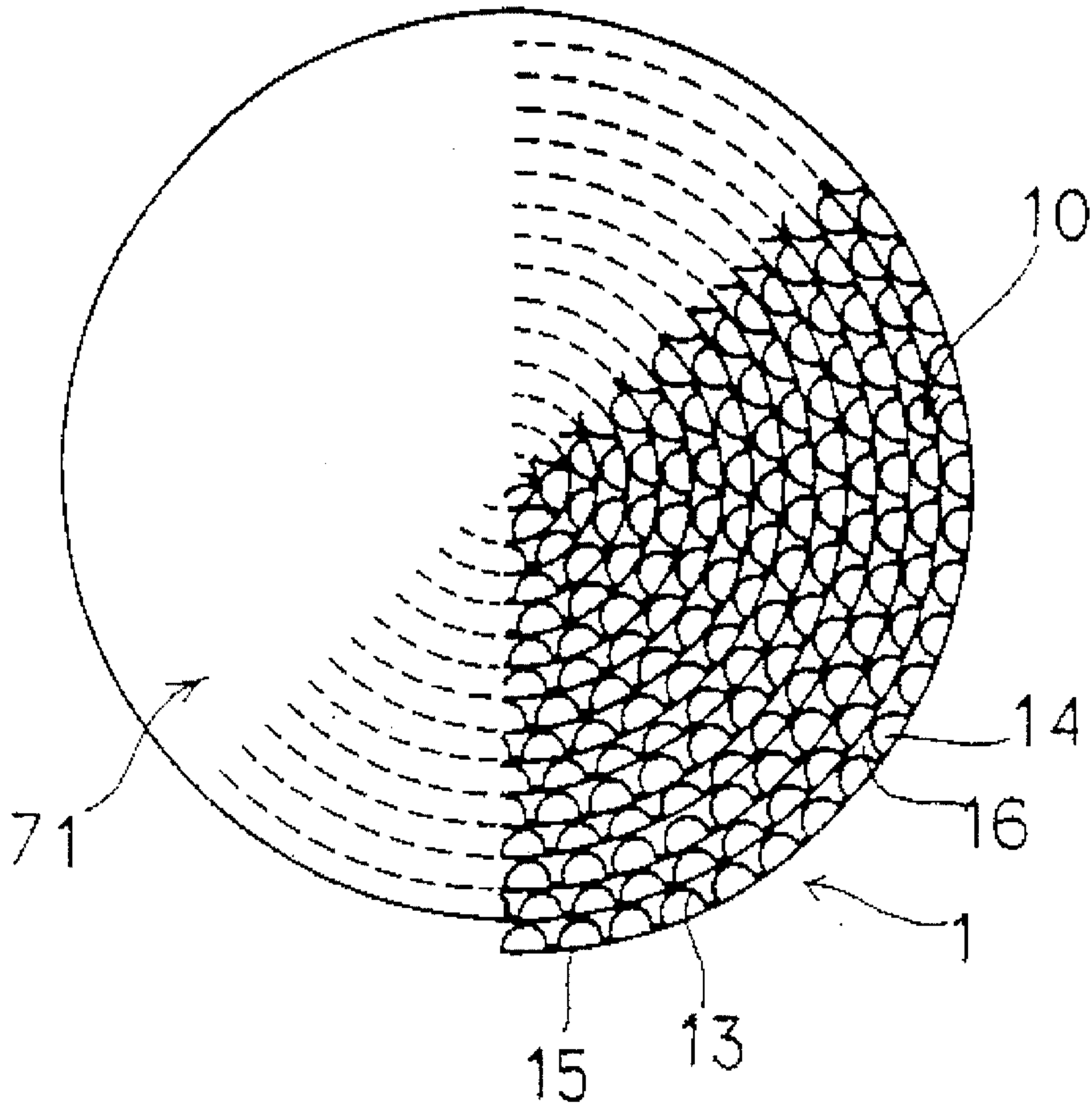
FIG. 24 PRIOR ART
