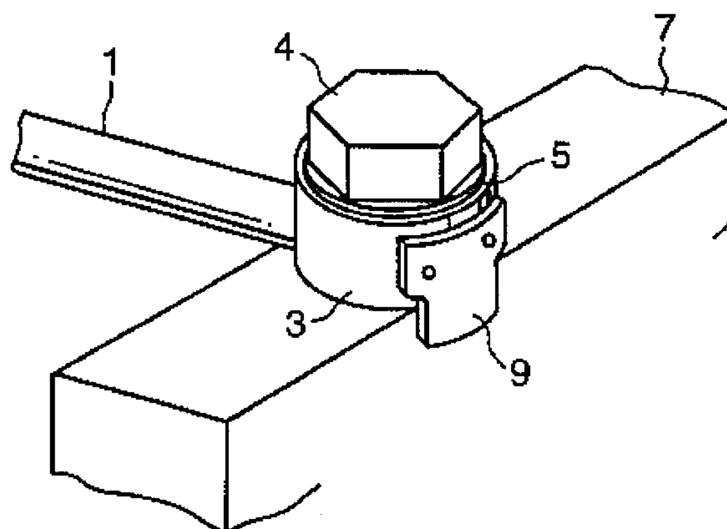
Fig. 14 (PRIOR ART)
