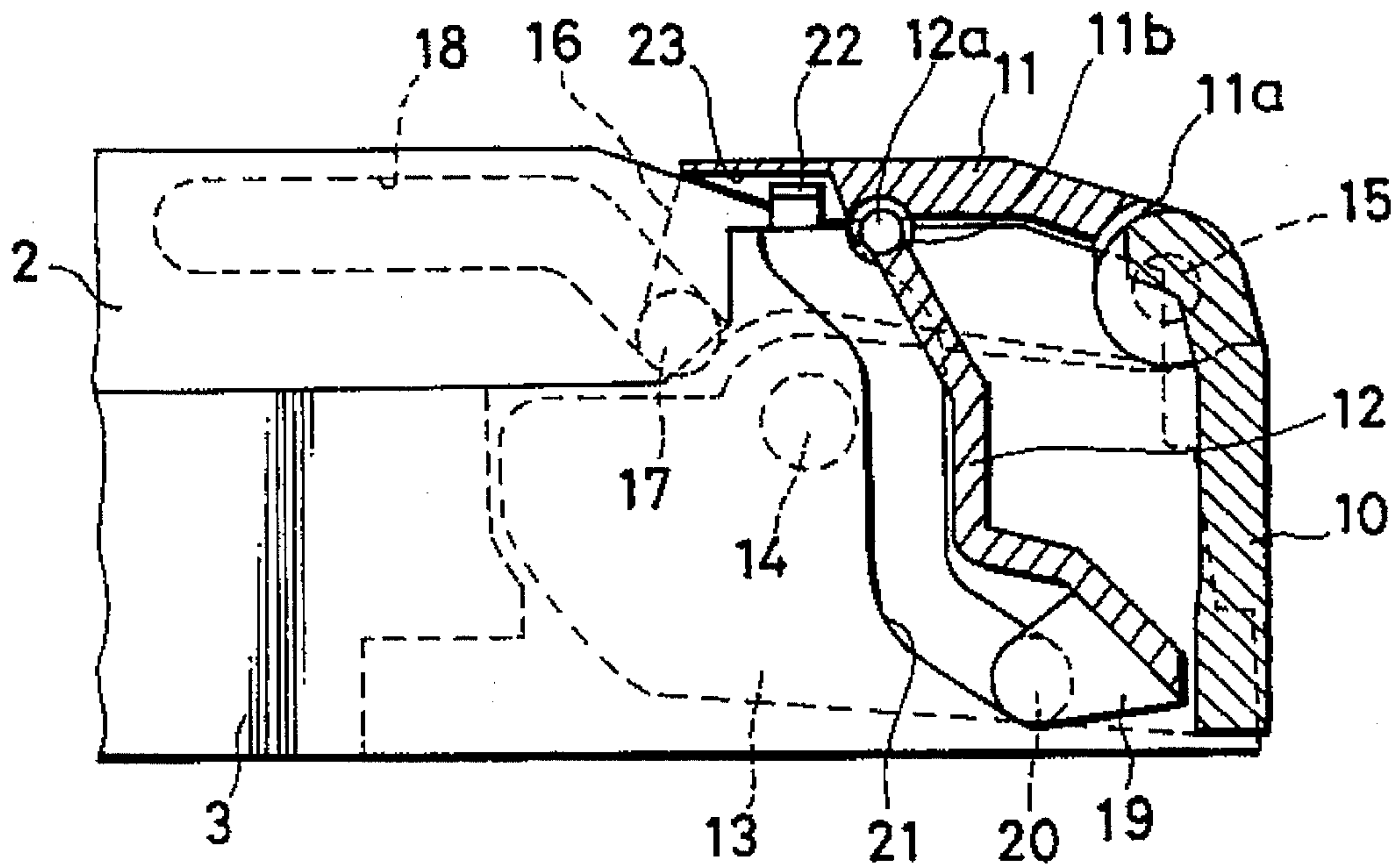
FIG. 6 (PRIOR ART)
