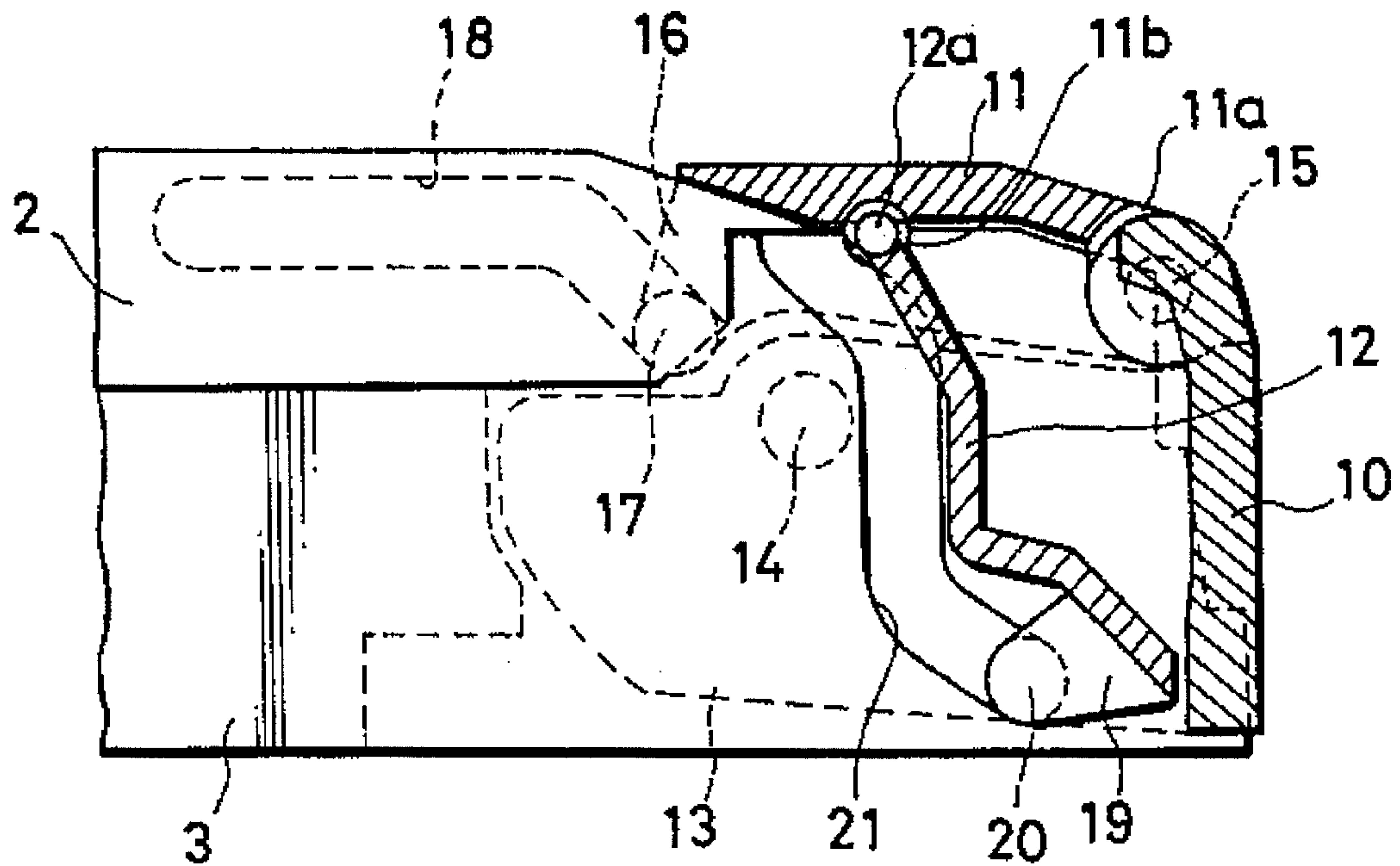
FIG. 4 (PRIOR ART)
