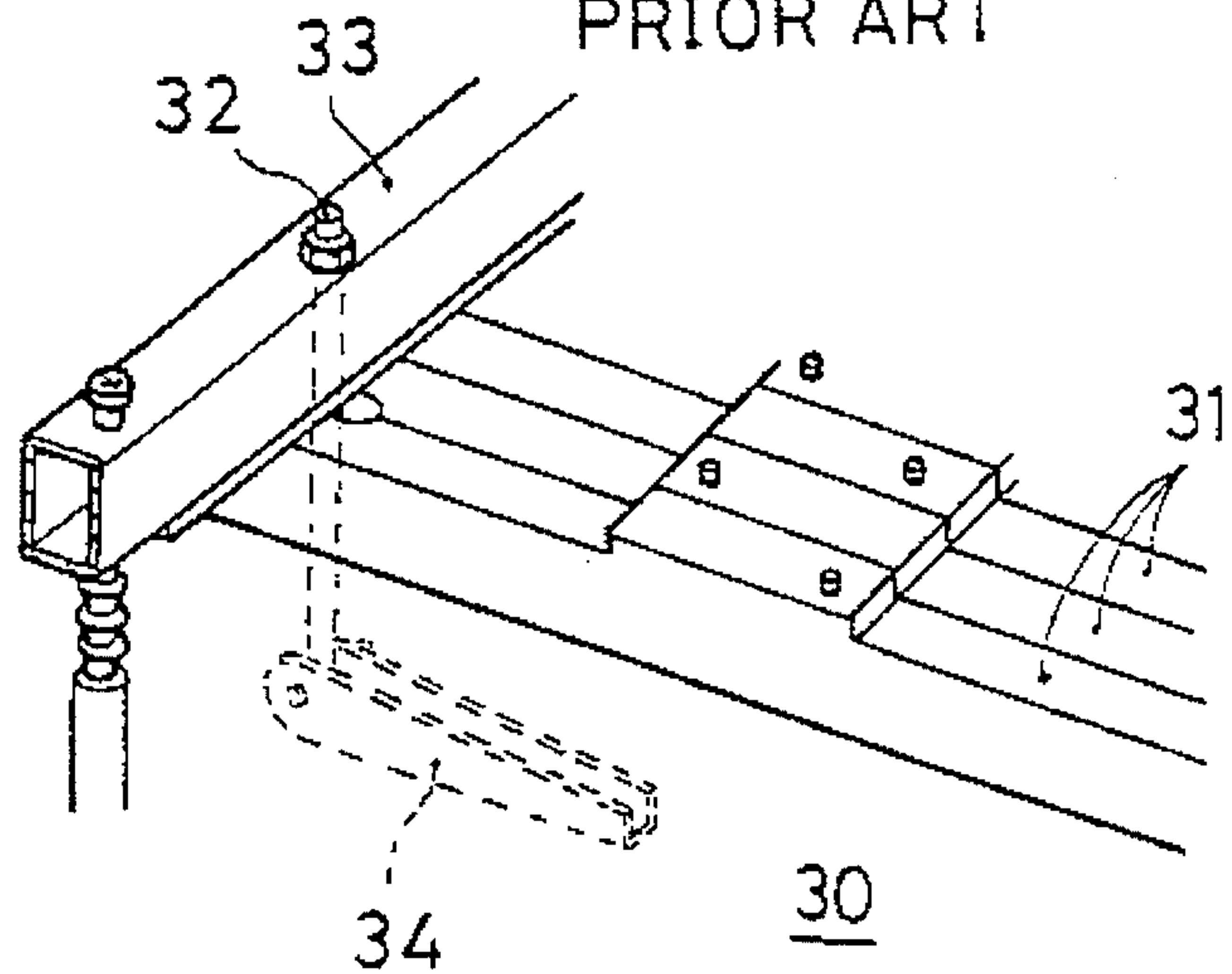
FIG. 7 PRIOR ART
