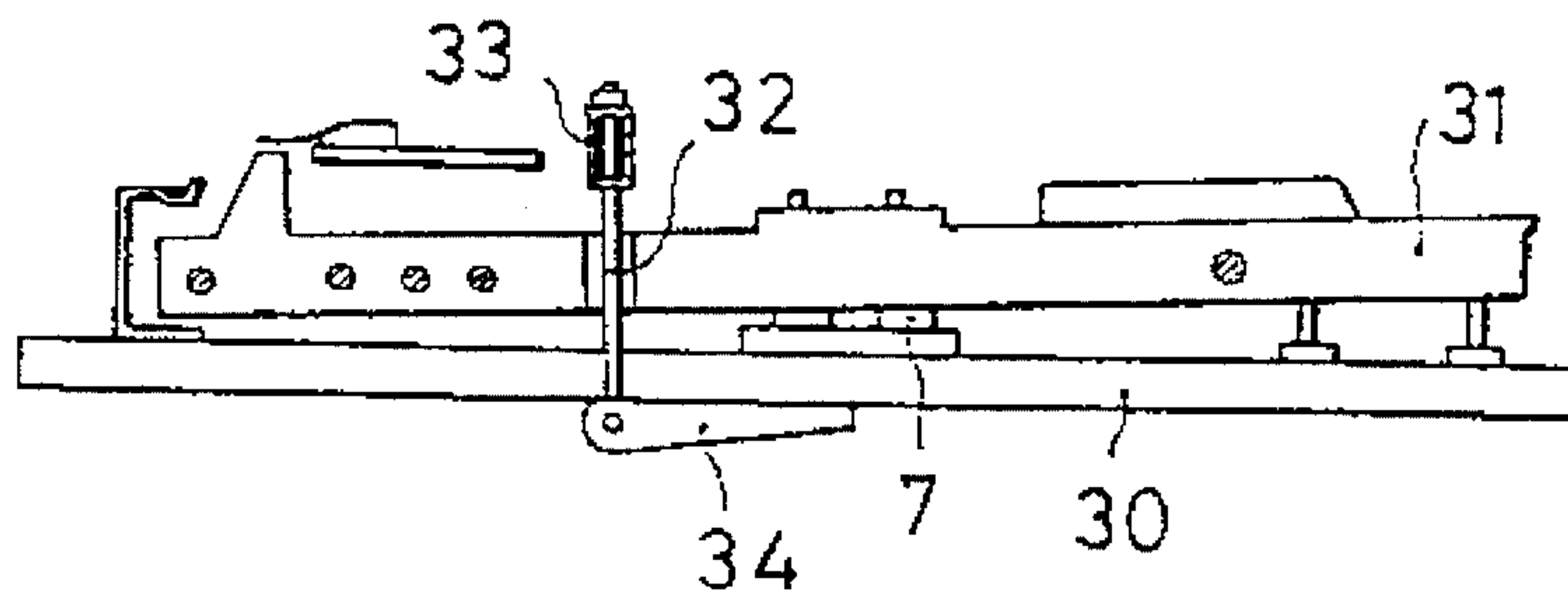
FIG. 7 PRIOR ART
