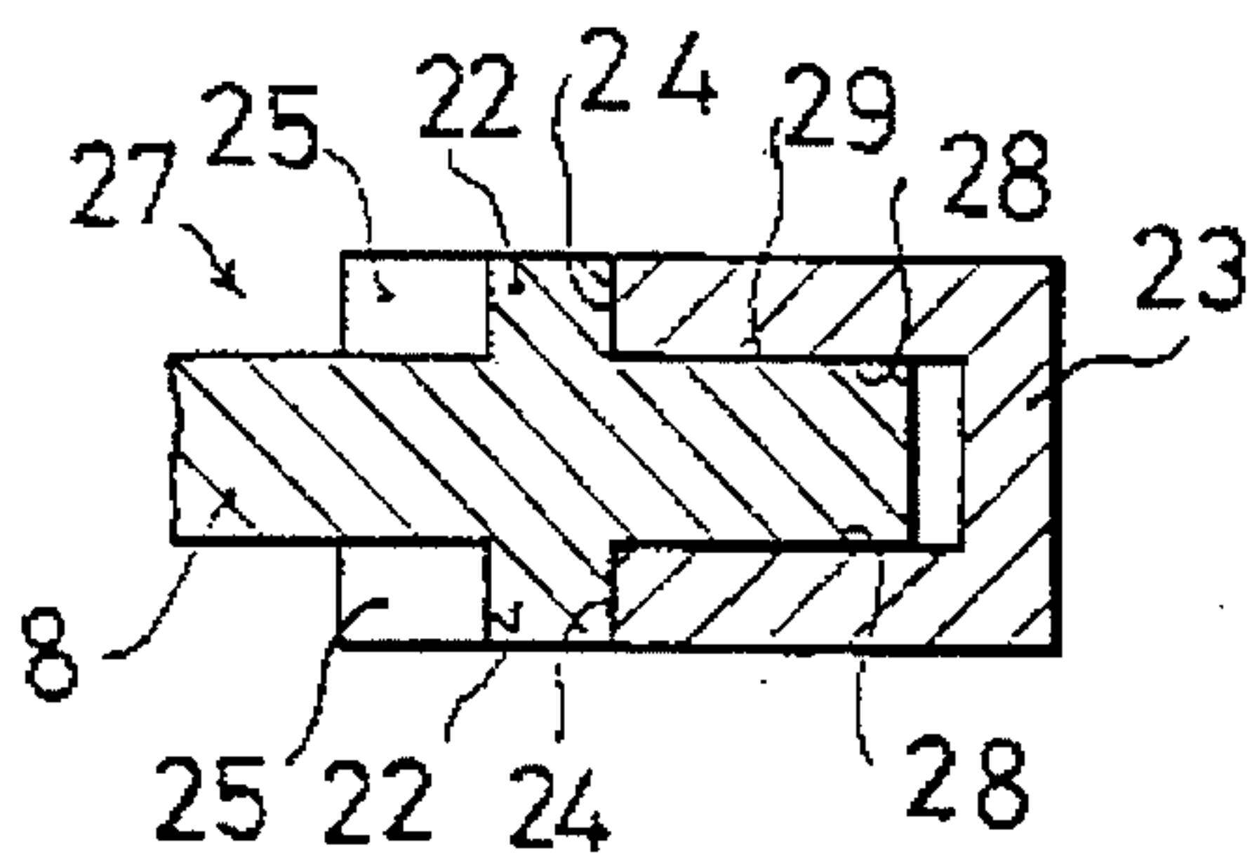
FIG. 6 PRIOR ART
