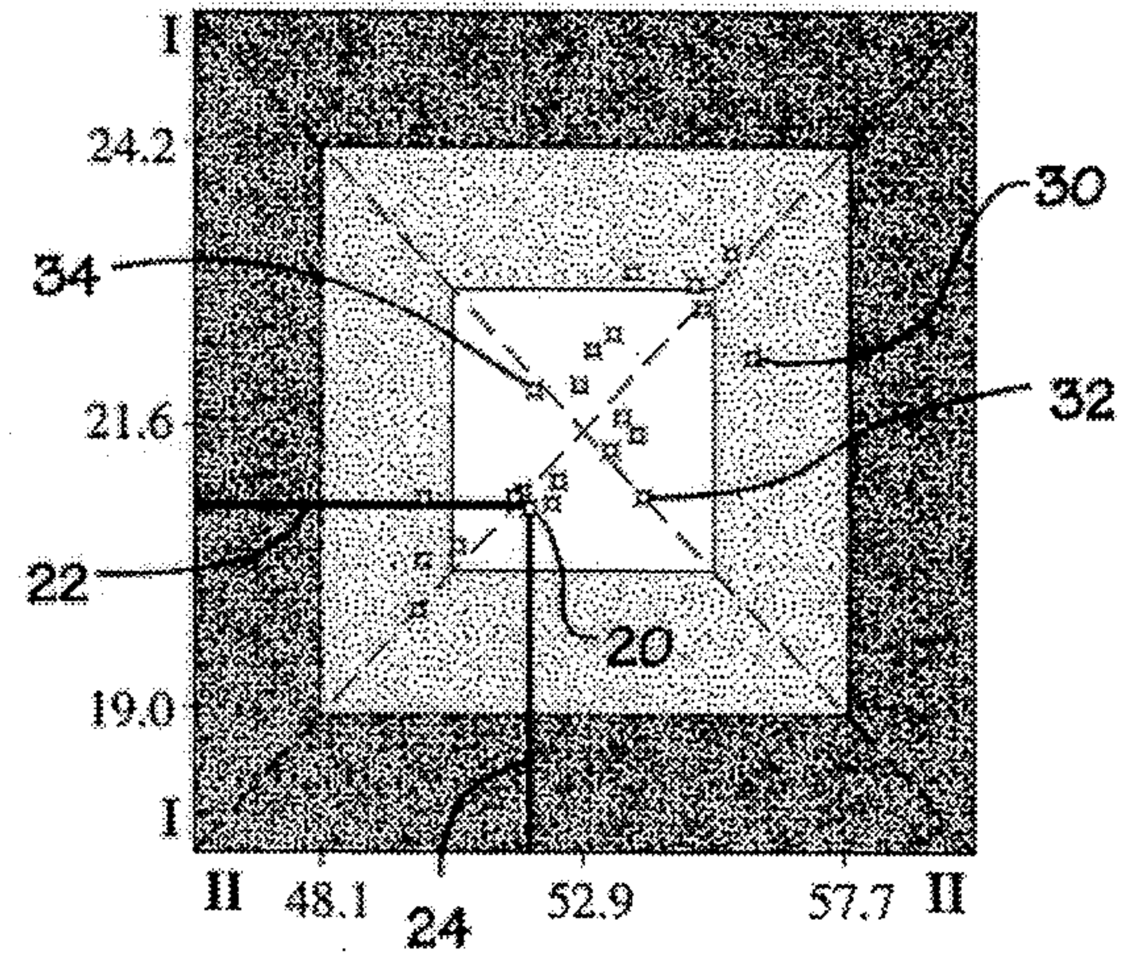
Fig. 3 - Prior Art
