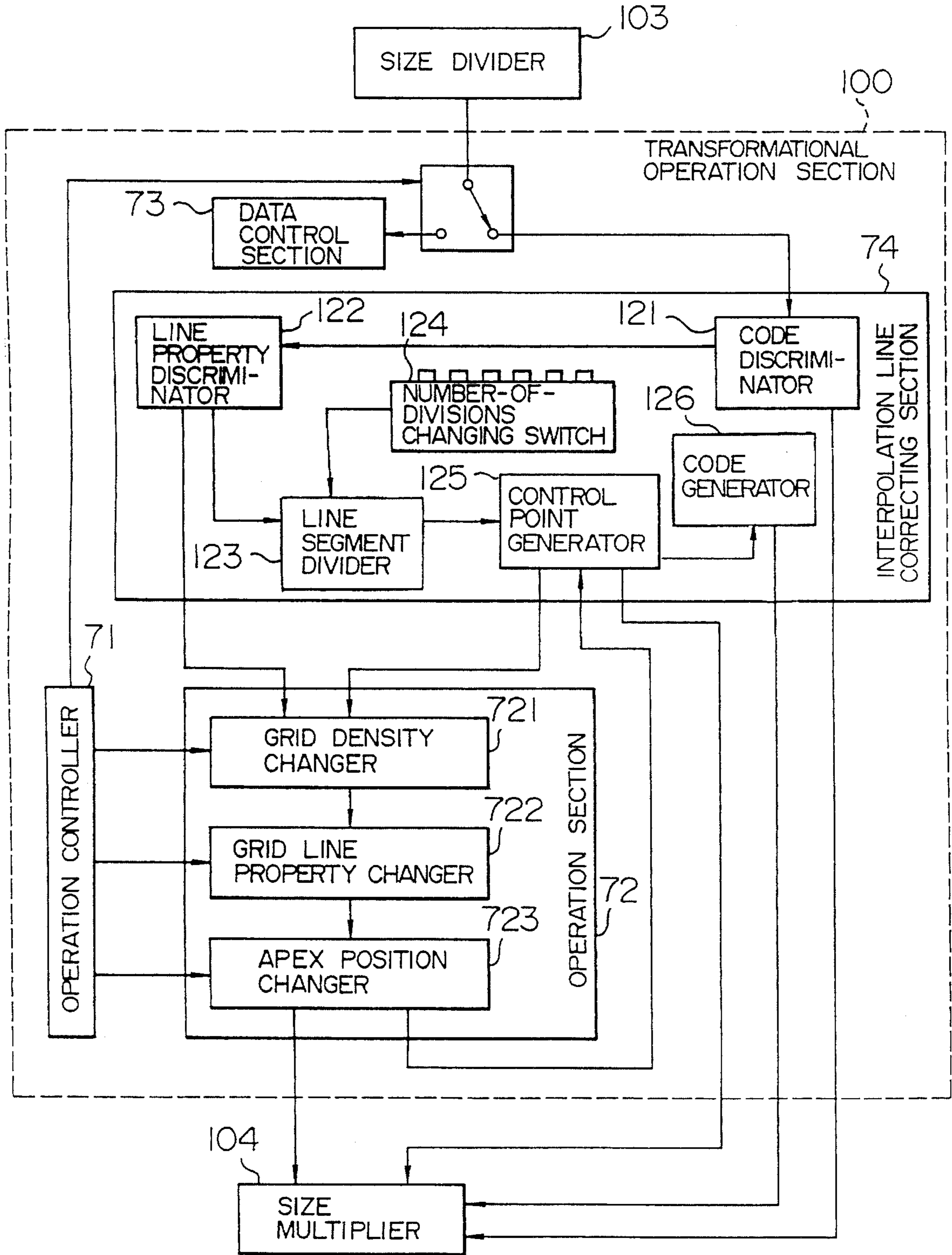
CONFIGURATION OF INTERPOLATION LINE CORRECTING SECTION
