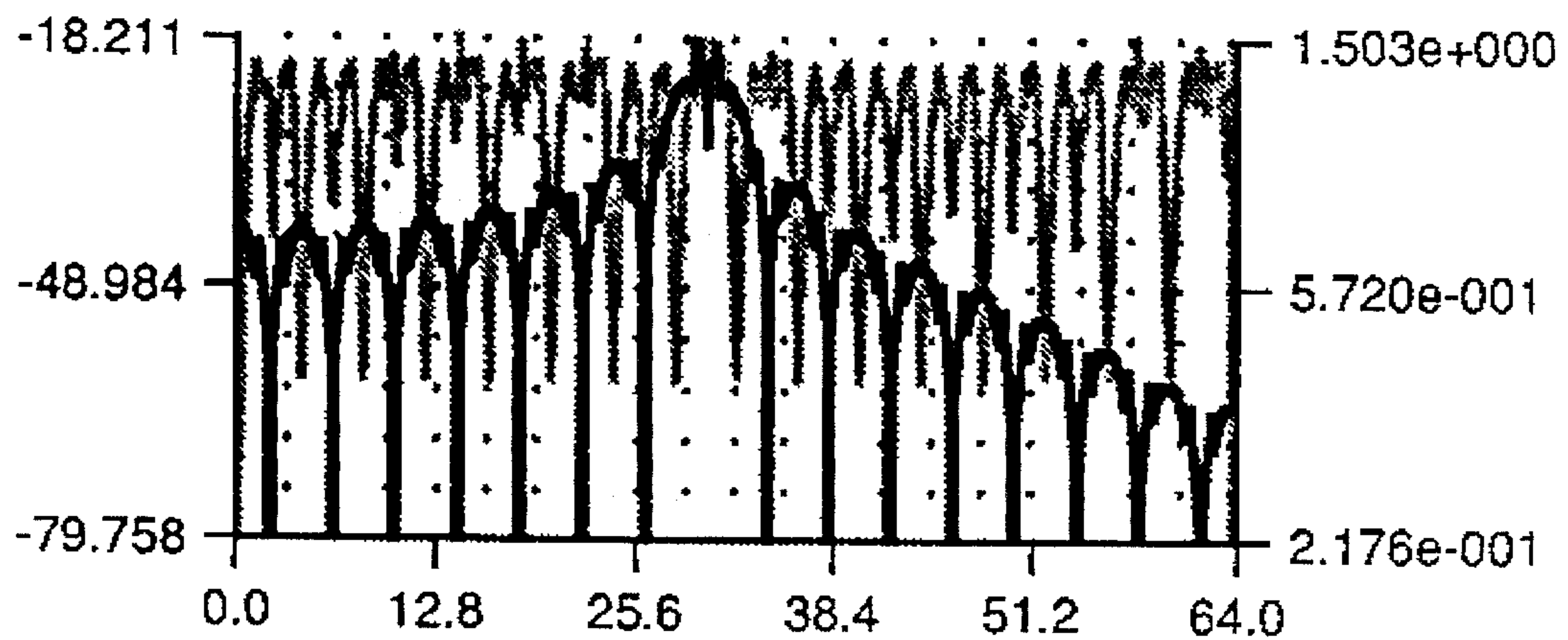
AMPLITUDE ON-OFF PLUS BIPHASE CARRIER MODULATION SPECTRUM
