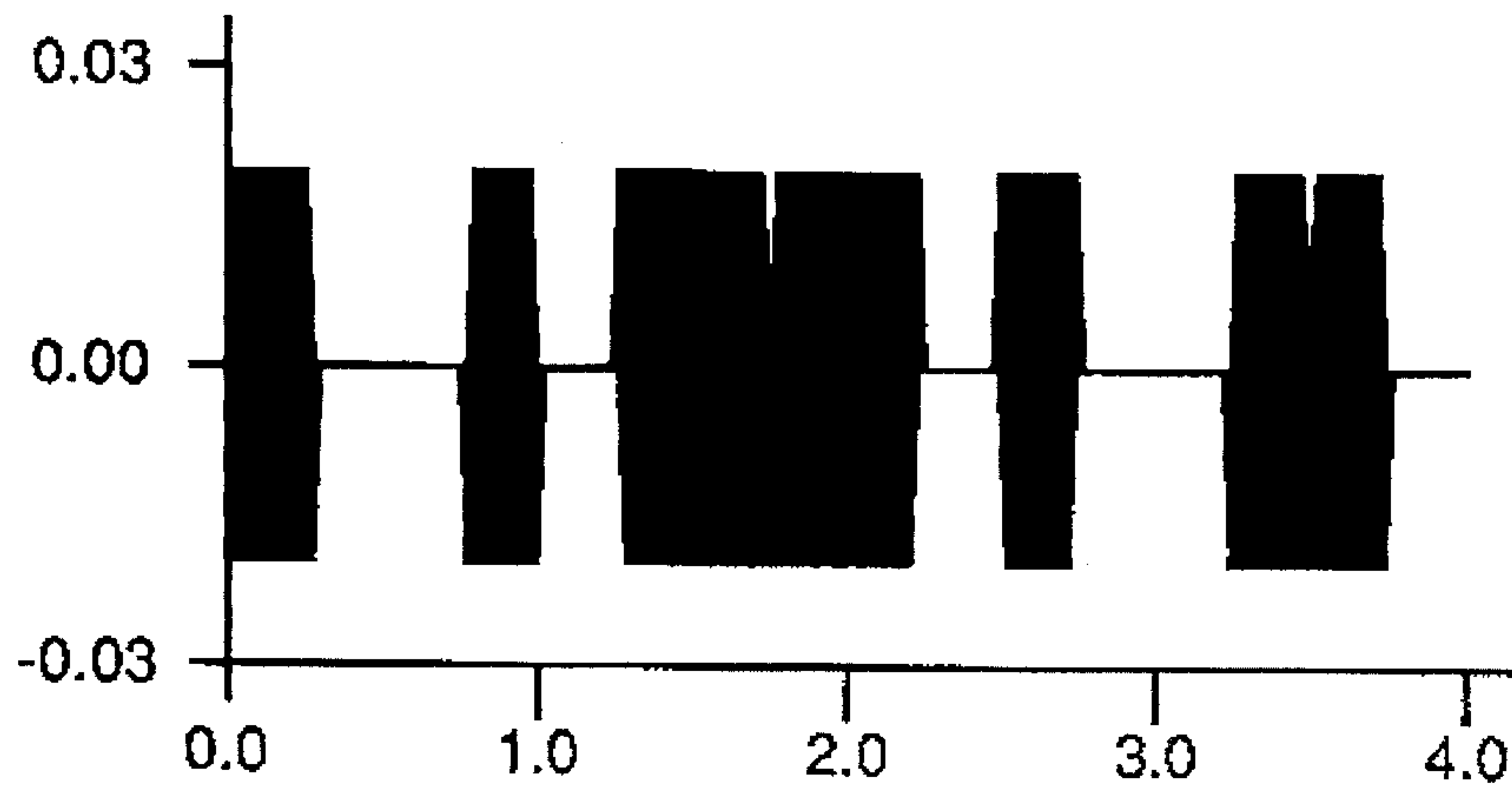
AMPLITUDE ON-OFF PLUS BIPHASE CARRIER MODULATION
