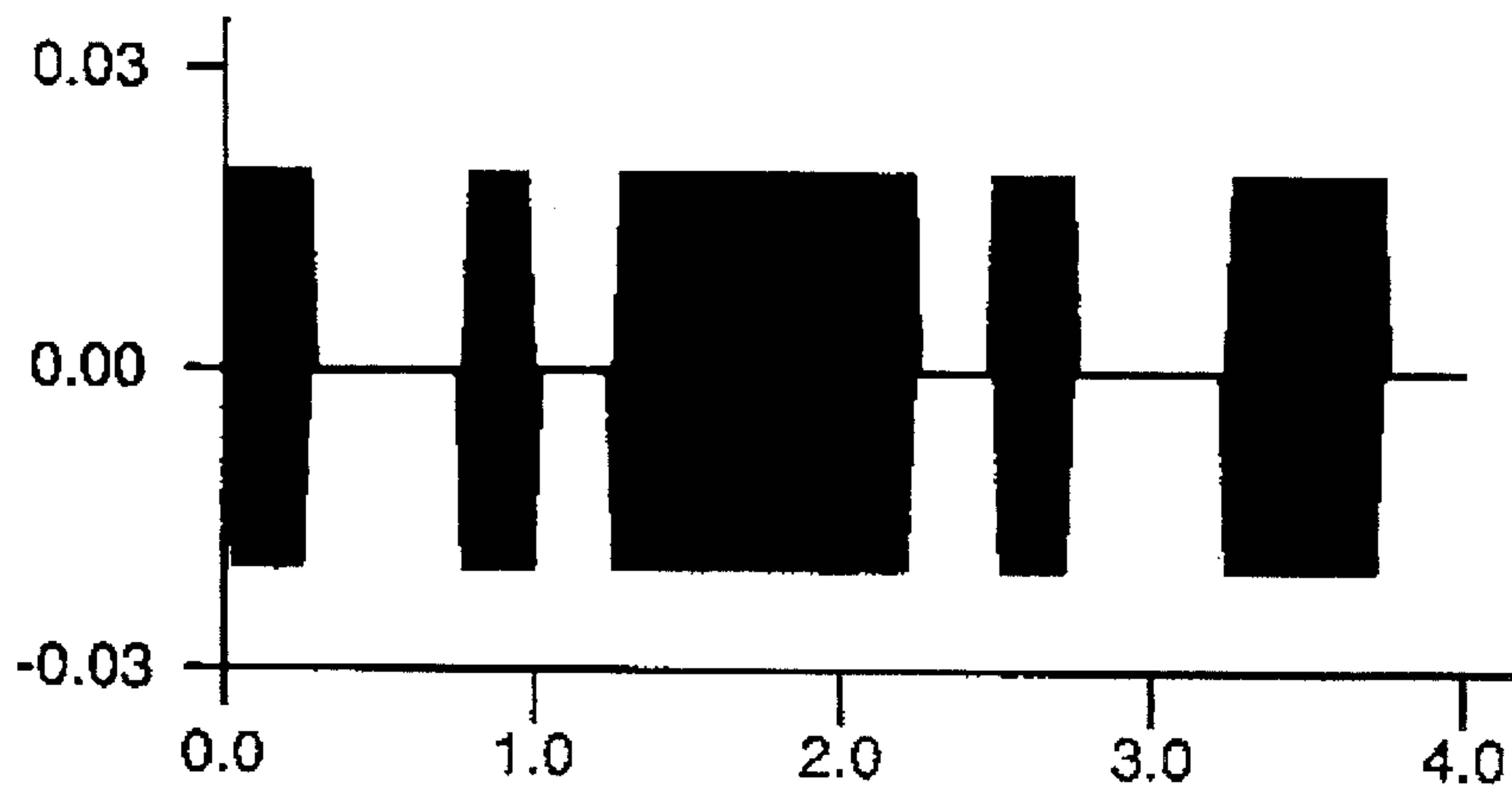
AMPLITUDE ON-OFF CARRIER MODULATION
